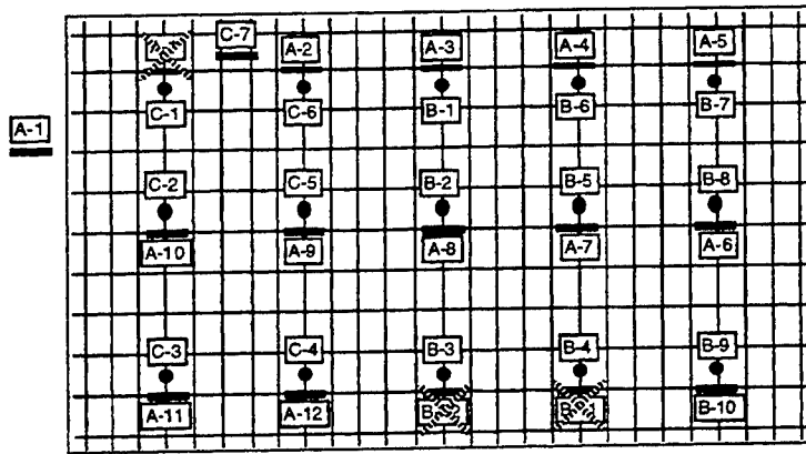
Figure 3-23 Fiber Bragg grating sensor placement in concrete deck (Davis et al, 1996)
