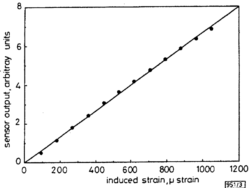
Figure 3-8 Response of sensor output voltage to three-point bending induced strain (Davis and Kersey, 1994)
