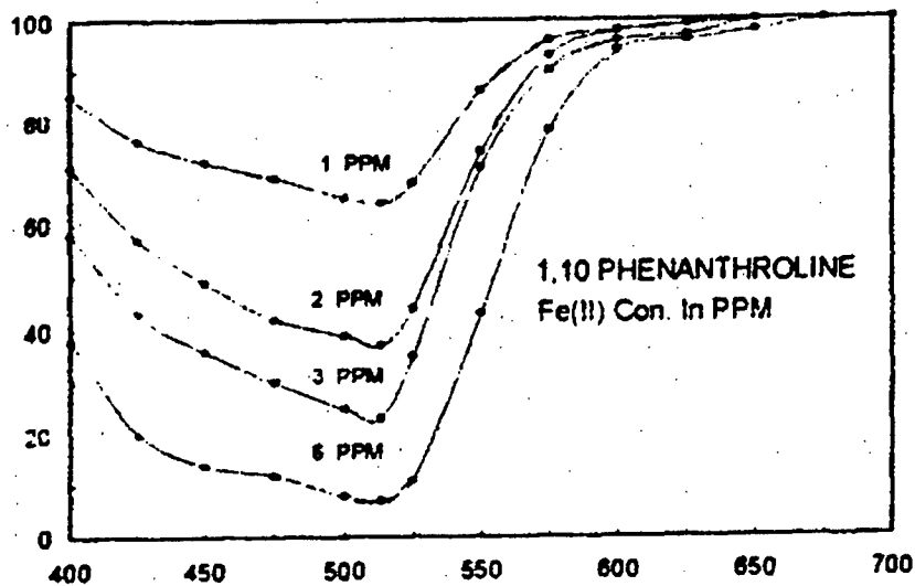
Figure 3-29 Absorption spectral of Ferriin ((Perez et al, 1995)
