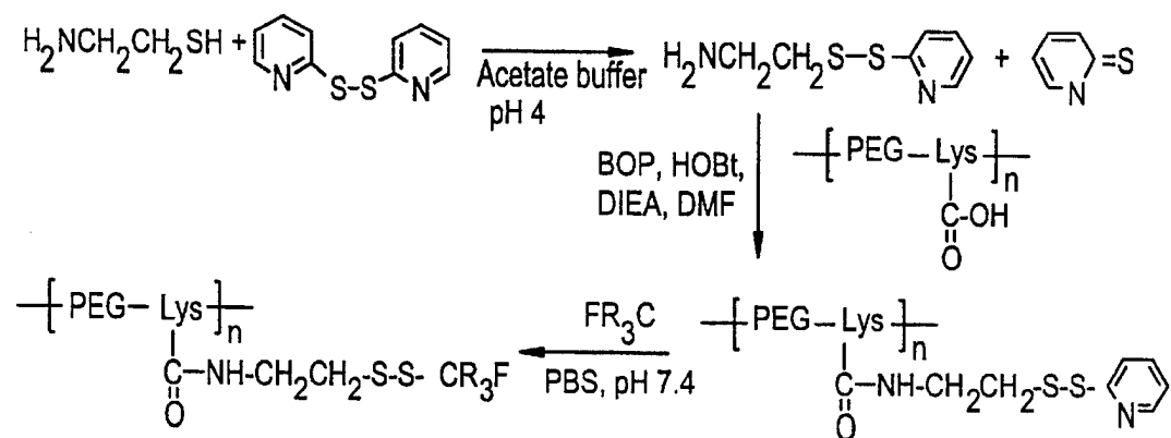
Scheme I
