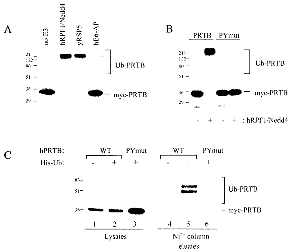
FIG. 3. hPRTB is an in vitro and in vivo ubiquitination substrate. A, hRPF1/Nedd4 ubiquitinates hPRTB in vitro . ^{35} S-labeled Myc-hPRTB was incubated with purified hRPF1/Nedd4 (whect), yRSP5, or hE6-AP in the presence of ATP, ubiquitin, and bacterially expressed E1 and E2 (UbcH5B) enzymes. B, the hPRTB-PY mutant is unable to be ubiquitinated by hRPF1/Nedd4 (whect). hPRTB and hPRTB-PYmut, containing a two-amino acid substitution (P40A/Y42A) of the PPAY motif, were assayed in a standard ubiquitination assay using E1, E2 (UbcH5B), and hRPF1/Nedd4 (whect) as the E3 enzyme. C, His-ubiquitin conjugates of hPRTB isolated from HeLa cells. HeLa cells were transfected with expression plasmids for His-ubiquitin and Myc-hPRTB or Myc-hPRTB-PYmut. Forty hours posttransfection, denatured lysates were prepared (lanes 1–3), and His-conjugates were purified on nickel resin (lanes 4–6). Myc-hPRTB or Myc-hPRTB-PYmut. His-ubiquitin conjugates were detected by Western immunoblot analysis using an antibody directed against c-Myc (9E10). WT, wild type.
