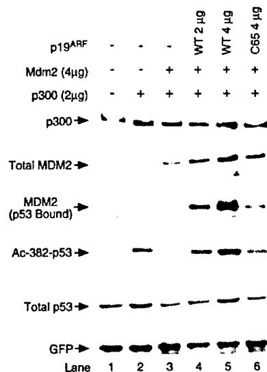
Fig. 5. p19 ARF reverses the inhibition of p53 acetylation by MDM2. H1229 cells were transfected with either expression plasmid for p53 wild-type and internal control GFP (lane 1) or co-transfected with c-myc-tagged p300 (lanes 2–6), in combination with MDM2 and p19 expression plasmid as indicated. Analysis of p53 protein and acetylation levels was carried out as described for Figures 1 and 2. Note that expression of p19 effectively neutralized the effects of MDM2 on p53 acetylation (lanes 4 and 5). p300 levels were determined by RW128.
