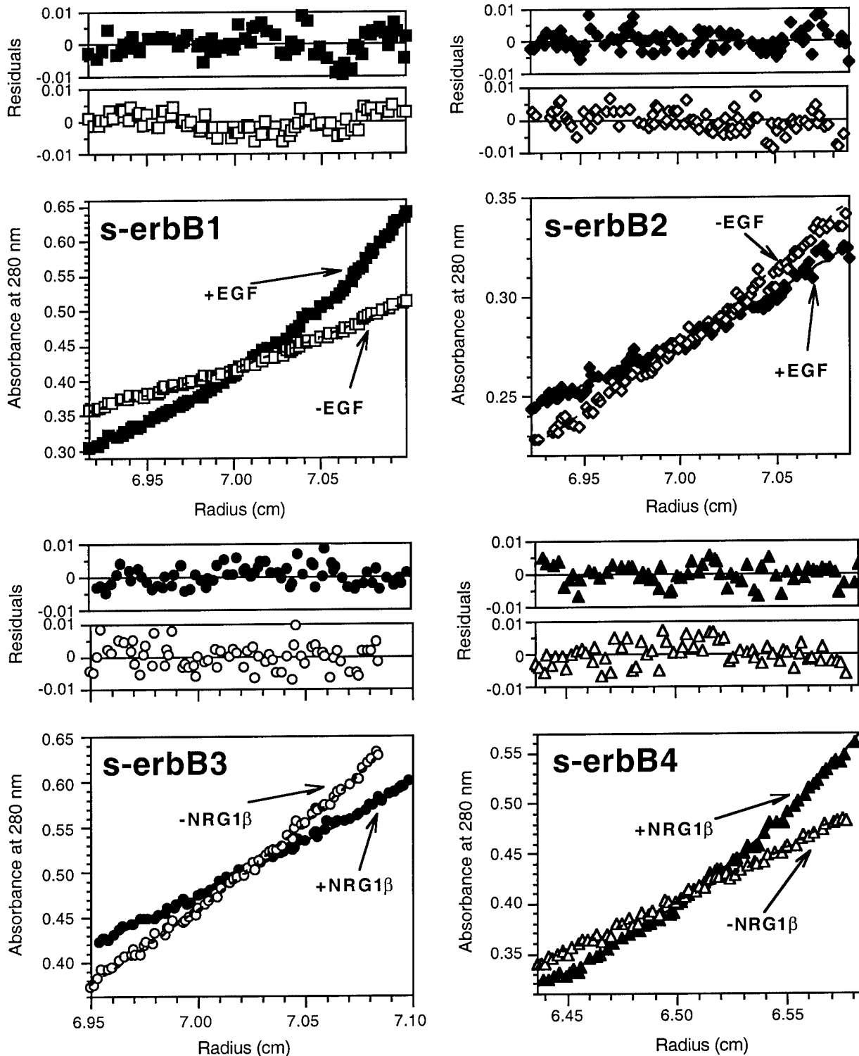
Figure 6 Representative sedimentation equilibrium analytical ultracentrifugation data for analysis of s-erbB homodimerization induced by EGF or NRG1- \beta 1. In each case, open symbols represent the unliganded receptor, which is fit as an ideal single species (molecular mass range from 80 kDa for s-erbB1 to 97 kDa for s-erbB4). Filled symbols represent samples to which has been added a two-fold molar excess of the noted ligand. Fits to these data are with two ideal species - fixing the Mw of the ligand and floating the Mw of the complex. Fits return Mw of 198 kDa for s-erbB1 (dimer), 77.5 kDa for s-erbB2 (monomer), 85 kDa for s-erbB3 (monomer), and 197 kDa for s-erbB4 (dimer). As described in the text, this result is clear from inspection of the
