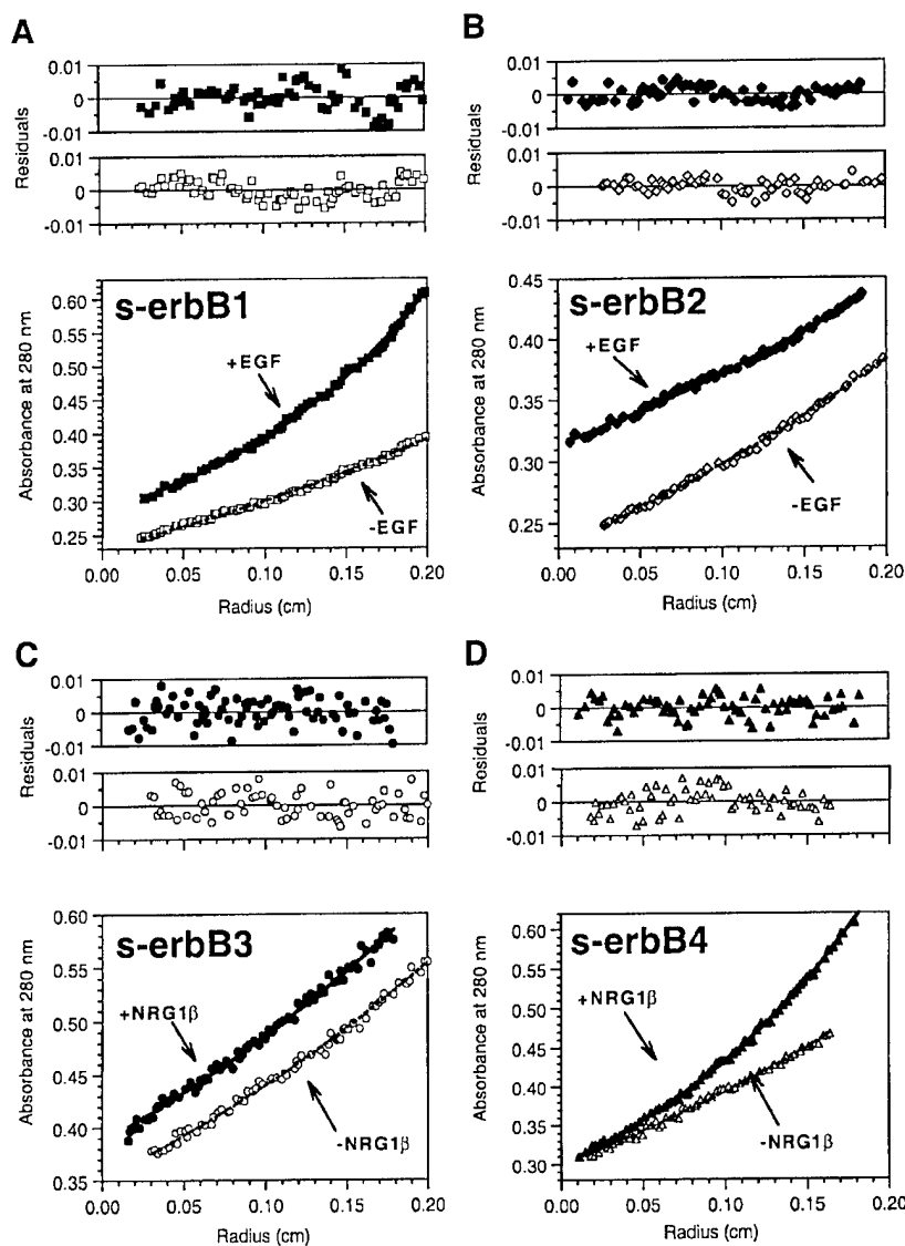
Fig. 4. Representative sedimentation equilibrium analytical ultracentrifugation data for analysis of s-erbB homo-oligomerization induced by EGF (A and B) or NRG1-β1 (C and D). In each case, open symbols represent s-erbB protein without added ligand, which is fit as a single non-ideal species. Filled symbols represent samples to which a 2-fold molar excess of the noted ligand has been added. As discussed in the text, fits to these data are with two ideal species (complex plus excess free ligand)—fixing the mass of the ligand and floating the mass of the complex. Purified s-erbB protein was used at 5 μM for each sample. All experiments shown were performed at 6000 r.p.m. Repeats at 9000 and 12 000 r.p.m. gave the same results. Residuals for the fits described above are shown, and are seen to be both small and random, indicative of a good fit. EGF induced homo-oligomerization of s-erbB1 only, while NRG1-β1 induced homo-oligomerization of s-erbB4 only. Radius is plotted as (r - r_0) , where r is the radial position in the sample, and r_0 the radial position of the meniscus.
