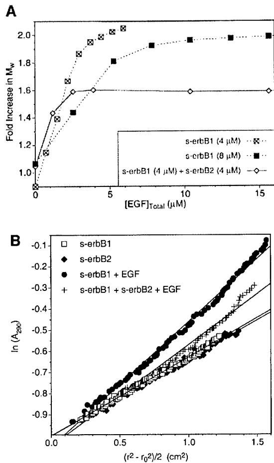
Fig. 5. (A) A MALLS experiment demonstrating that, while EGF induces complete homo-dimerization of s-erbB1 at 4 \mu\text{M} (crossed squares) or 8 \mu\text{M} (filled squares), it does not induce the formation of heterodimers between s-erbB2 and s-erbB1 (open diamonds). The experiment was performed as described for Figure 3. With 4 \mu\text{M} s-erbB1, complete dimerization is seen after addition of 4 \mu\text{M} EGF (note that the horizontal axis here is EGF concentration, and not ligand:receptor ratio). With 8 \mu\text{M} s-erbB1, addition of 8 \mu\text{M} EGF is required for complete dimerization. When the 1:1 s-erbB1:s-erbB2 mixture is studied, with a total s-erbB protein concentration of 8 \mu\text{M} , only 4 \mu\text{M} EGF is required for maximal dimerization, and the maximum fold increase in M_w is consistent only with a mixture of s-erbB1 homodimers and s-erbB2 monomers. Lines are drawn to guide the eye, and do not represent fits to the data. (B) Plots of the natural logarithm of absorbance at 290 nm (monitoring protein concentration) against a function of the radius squared ( r^2 - r_0^2 )/2 (see text for explanation) for sedimentation equilibrium analytical ultracentrifugation data obtained at 6000 r.p.m. with s-erbB1 and s-erbB2. For an ideal single species, this representation of the data should appear as a straight line with a gradient proportional to the molecular mass (see text). When analyzed alone, both s-erbB1 (open squares) and s-erbB2 (filled diamonds) yield good straight lines, with gradients proportional to their monomeric molecular masses (see also fits in Figure 4). Each sample contained a total s-erbB concentration of 10 \mu\text{M} . The increase in gradient for the s-erbB1/s-erbB2/EGF mixture (crosses) is consistent with the formation of s-erbB1 homodimers only.
