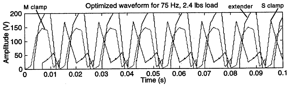
Figure 6.15. Optimized waveform for 75 Hz frequency with 2.4 lbs load.
