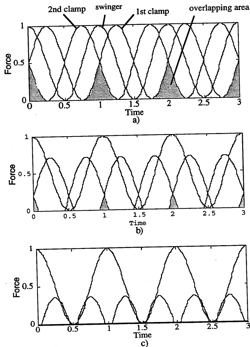
Figure 4.4. a) Force output form of three parts of motor without gap, b) With small gap, c) With large gap.
