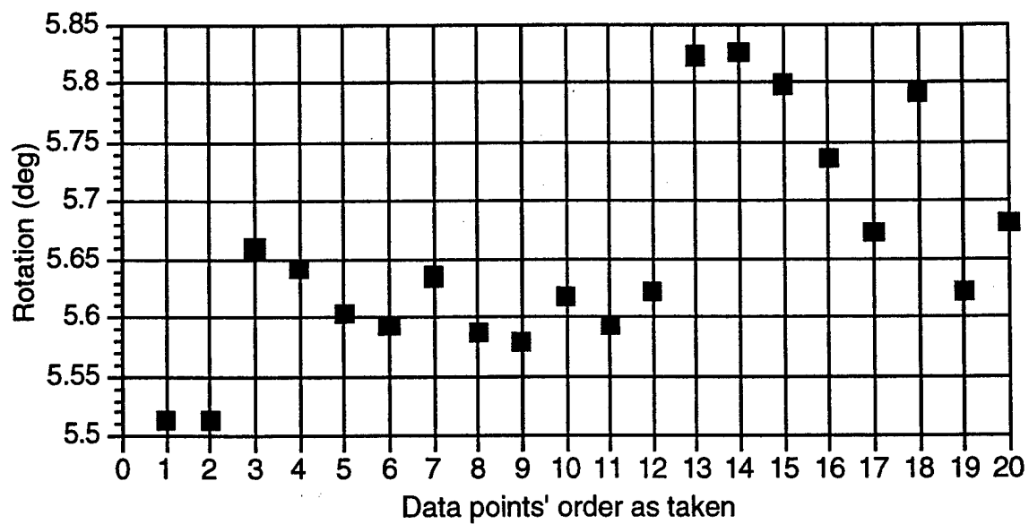
Figure 7.26. Distance traveled after fifteen steps with optimized signals, 30 Hz.
