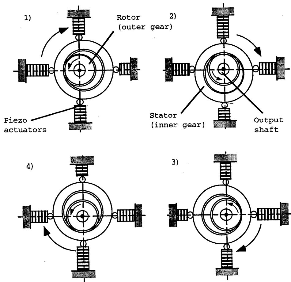
Figure 2.14. Direct drive motor - cycloid motor (Hayashi 1992).
