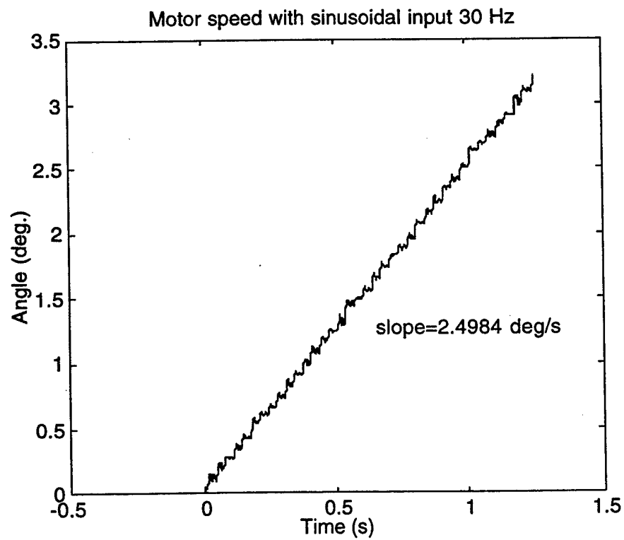
Figure 7.3. Motor steps with sinusoidal input at 30 Hz.
