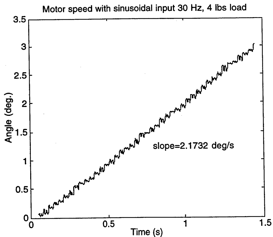
Figure 7.10. Motor speed with sinusoidal input at 30 Hz, 4 lbs load.
