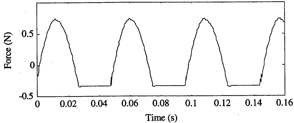
Figure 4.3. Clamping force of contact shoe versus time with initial gap.
