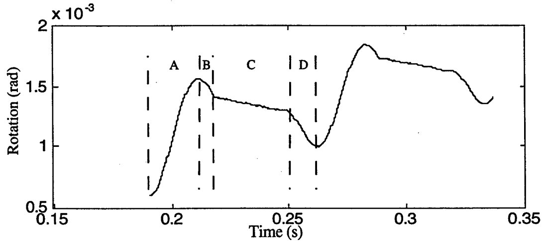
Figure 4.12. Detail step of motor.
