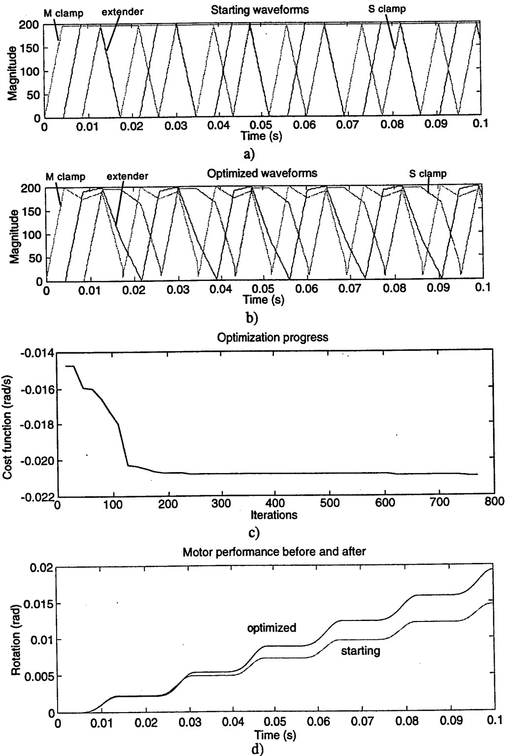
Figure 6.8. Optimization with square wave starting location: a) starting waveform, b) Optimized waveform, c) Optimization progress, d) Performance before and after optimization.
