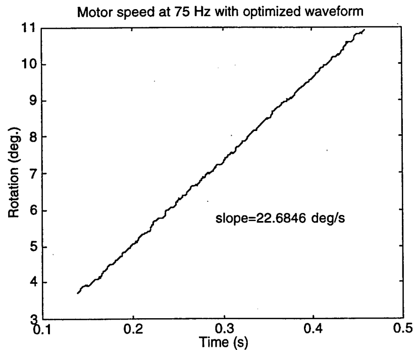
Figure 7.19. Motor speed with optimized waveform input at 75 Hz.
