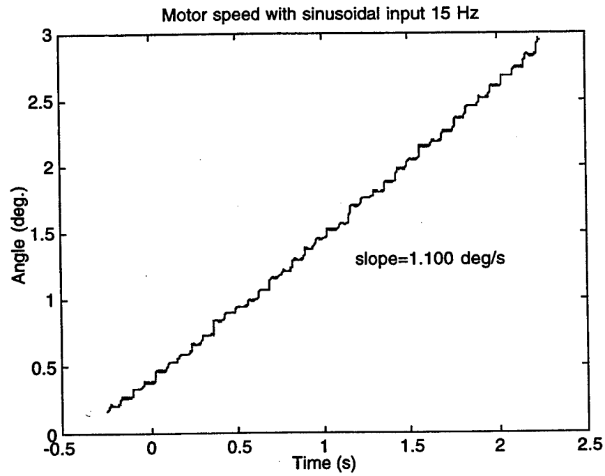
Figure 7.2. Motor steps with sinusoidal input at 15 Hz.
