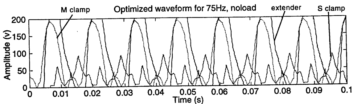
Figure 6.12. Optimized waveform for 75 Hz frequency, noload.
