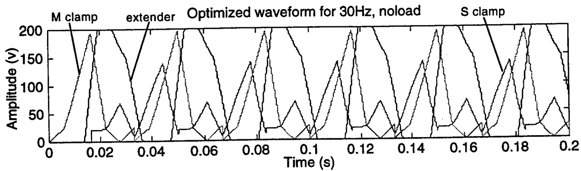
Figure 6.10. Optimized waveform for 30 Hz frequency, noload.
