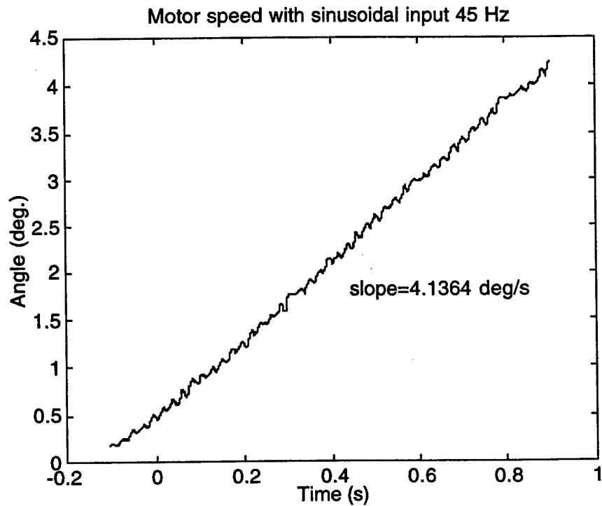
Figure 7.4. Motor steps with sinusoidal input at 45 Hz.
