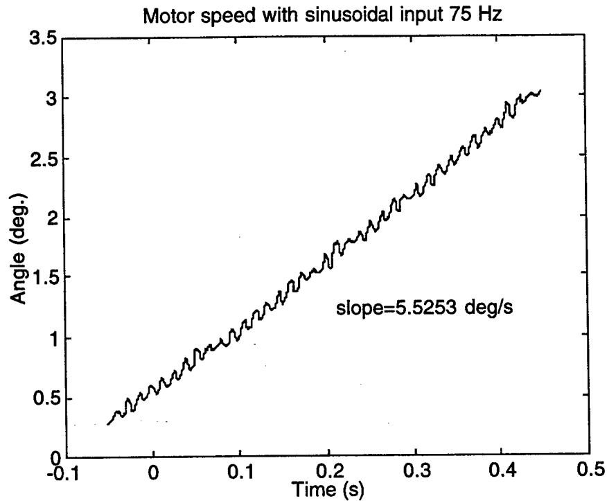
Figure 7.6. Motor steps with sinusoidal input at 75 Hz.
