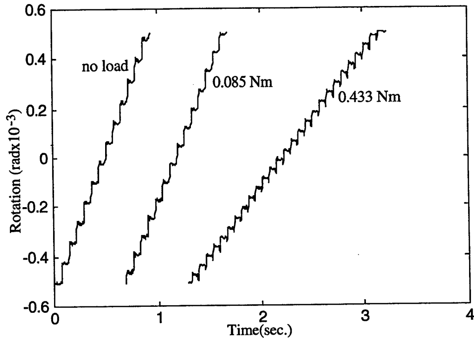
Figure 4.11. Motor steps taken experimentally.
