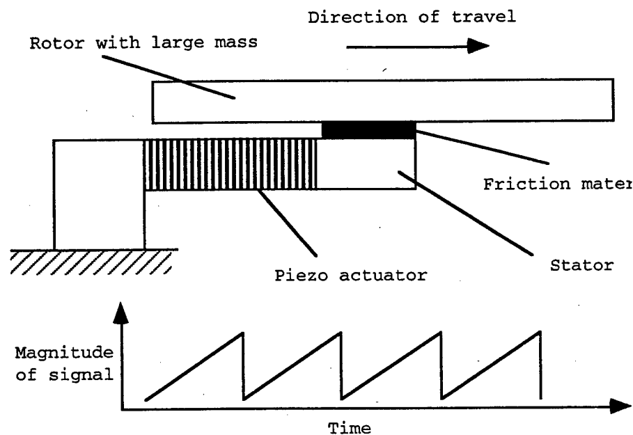
Figure 2.13. Inertial stepper motor.
