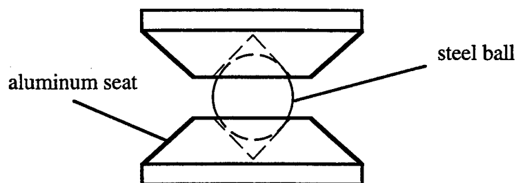
Figure 3.2. Stress relief device.
