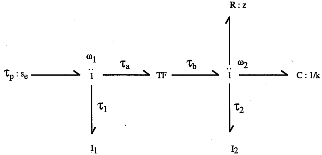
Figure 5.2. Bond diagram of clamping mechanism.
