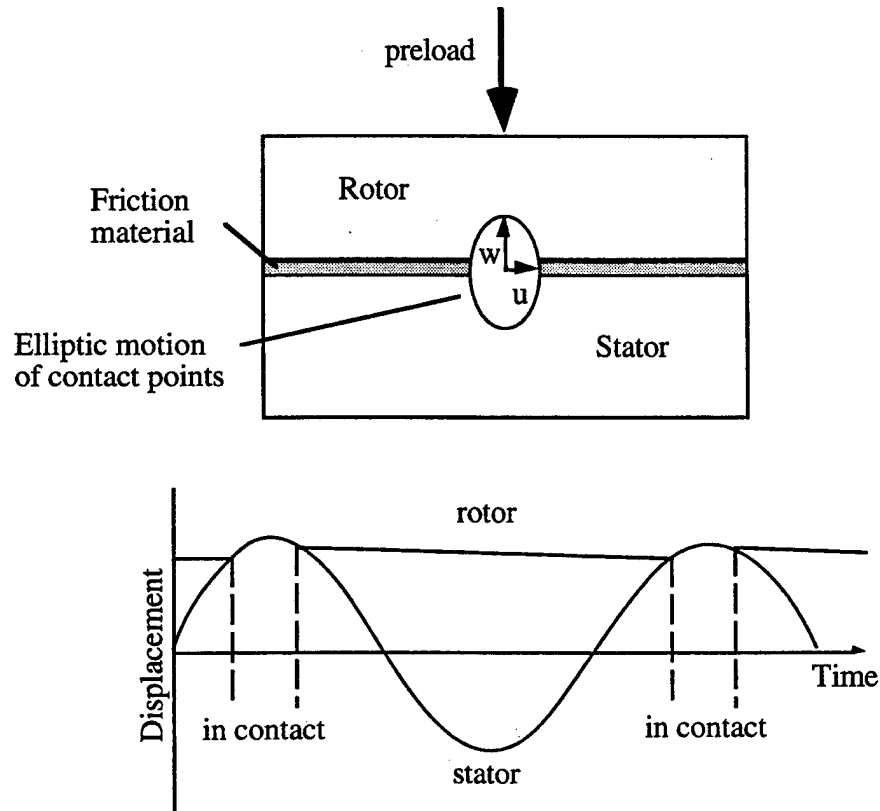
Figure 2.3. Operating principle of ultrasonic motors (Ueha, 1989) [12].
