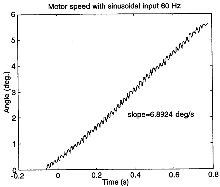
Figure 7.5. Motor steps with sinusoidal input at 60 Hz.
