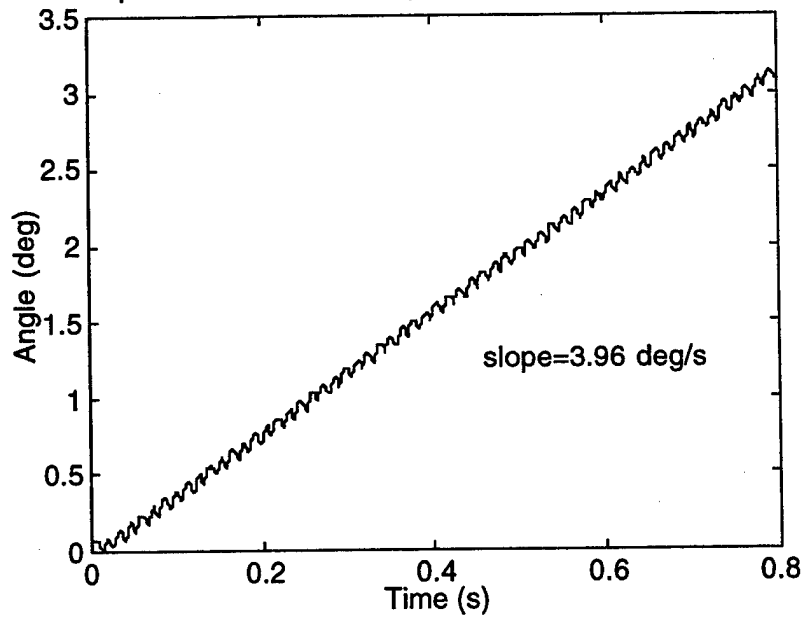
Motor speed with sinusoidal input, 75 Hz, 2.4lbs load, simulated
