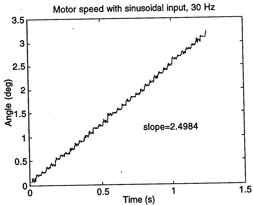
Figure 5.7. Motor step profile at 30 Hz frequency.
