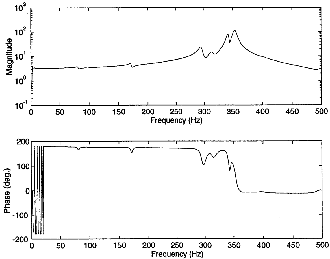
Figure 4.5. Experimental transfer function of clamping arm.
