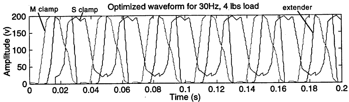
Figure 6.13. Optimized waveform for 30 Hz frequency with 4 lbs load.
