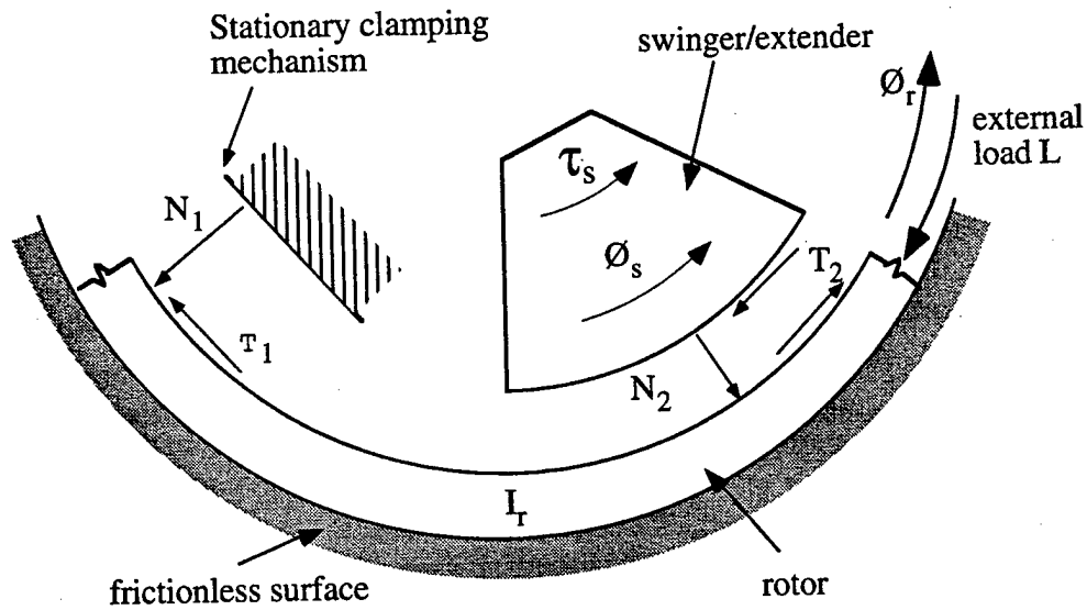
Figure 5.6. Rotor dynamic model.
