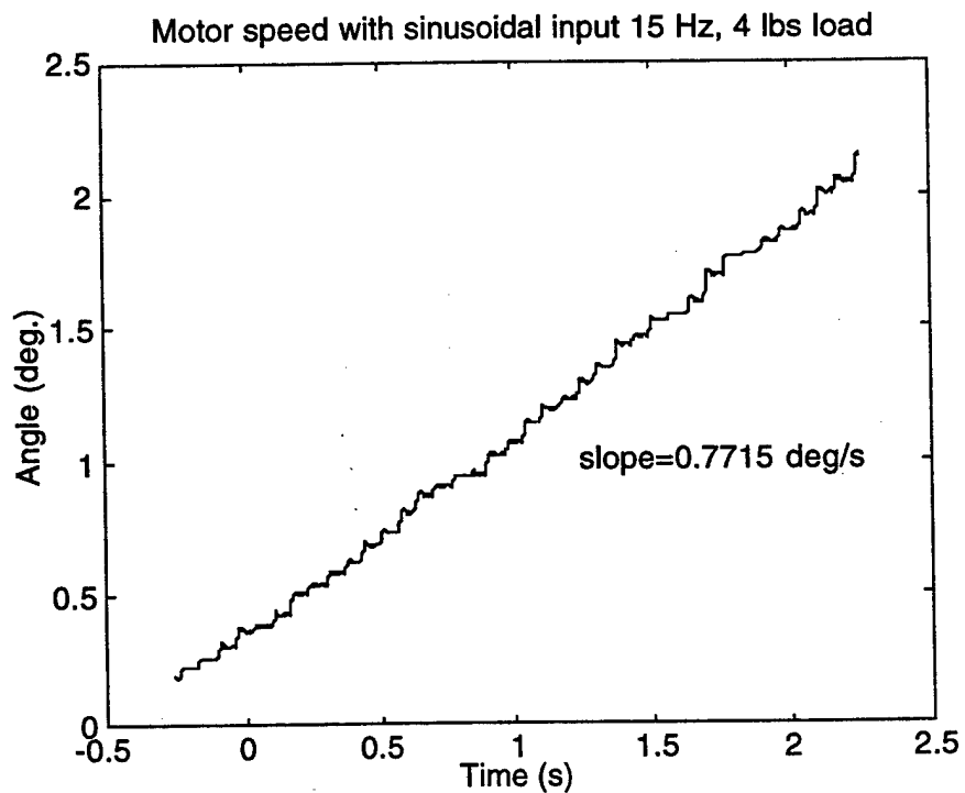
Figure 7.9. Motor speed with sinusoidal input at 15 Hz, 4 lbs load.
