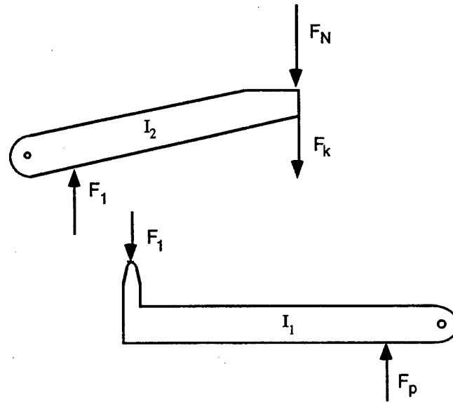
Figure 5.3. Free-body diagram of clamping mechanism components when in contact.
