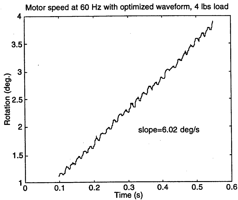
Figure 7.21. Motor speed with optimized waveform input at 60 Hz, 4 lbs.
