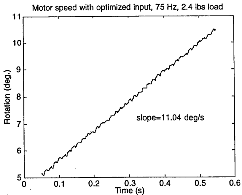
Figure 7.22. Motor speed with optimized waveform input at 75 Hz, 2.4 lbs.
