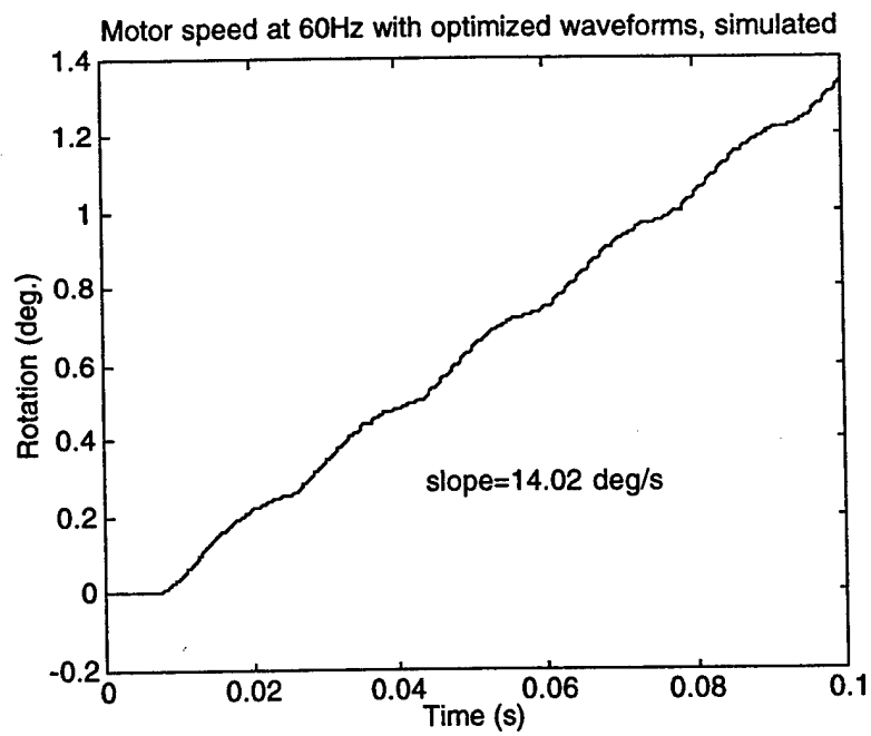
Figure 7.15. Simulated motor speed with optimized waveform at 60 Hz.
