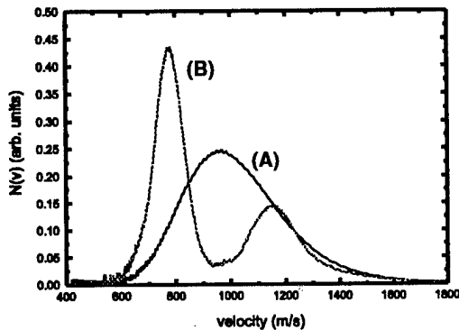
FIG. 1. The measurable force is limited by the geometry of this experiment to be \sim 10F_{rad} , but we believe it to be closer to \sim 50F_{rad} . Curve A shows the velocity distribution measured by transforming the TOF signal directly from the source. Curve B shows the distribution with a bichromatic cooling force whose parameters correspond to \Delta v \sim 300 \text{ m/s} . The slow atoms appear as a peak in the velocity distribution almost completely outside the residual velocity distribution of unslowed atoms.
