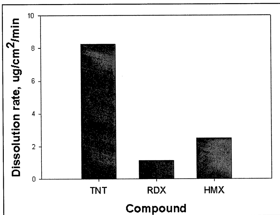
Figure 27. Dissolution rates of TNT, RDX, and HMX at 10 °C and 150 rpm stirring rate
