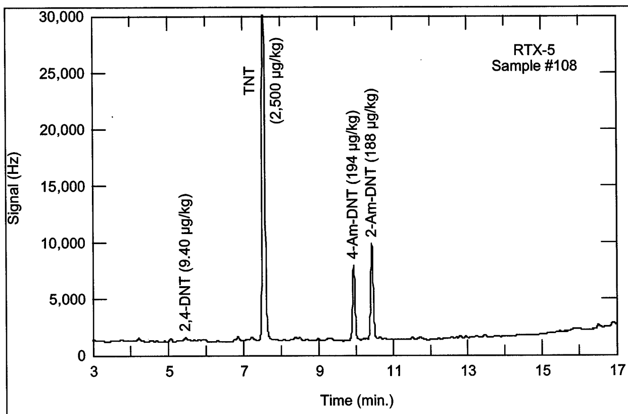
Figure 21. Chromatogram of soil sample collected 15 cm from position of a low-order 155-mm howitzer round
