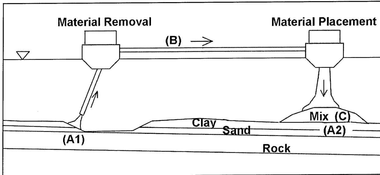
Figure 1. Illustration of dredged material fate
