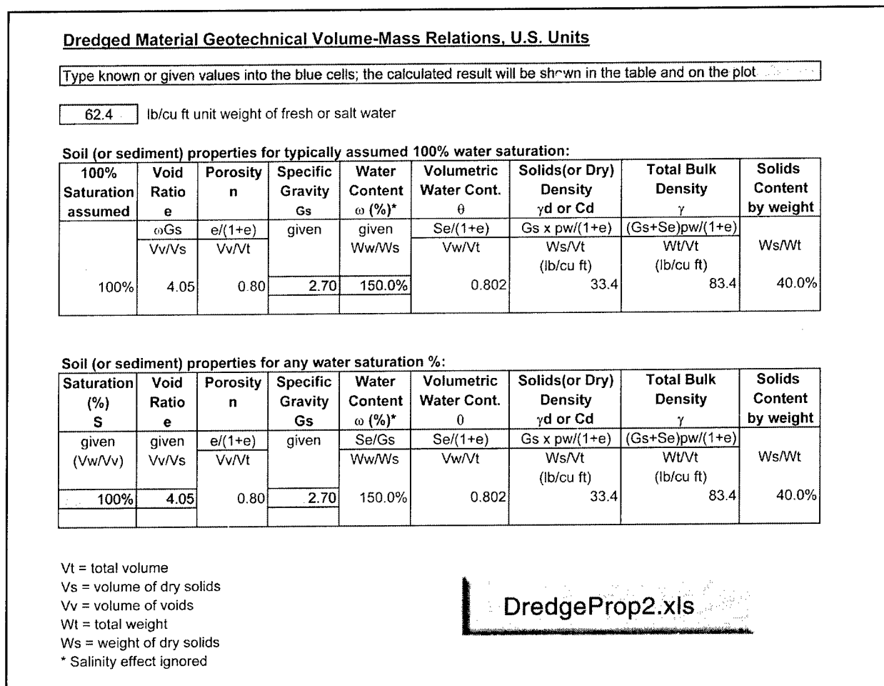
Figure 3. Spreadsheet for computing selected weight – volume relationships
