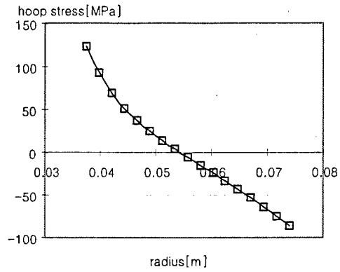
(b) hoop stress of cylinder A
