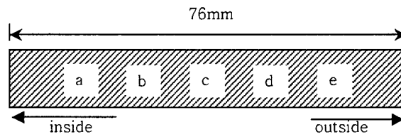
(a) radial locations for measurement of the fiber volume fractions
