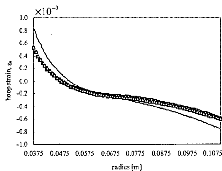
(e) hoop strains
