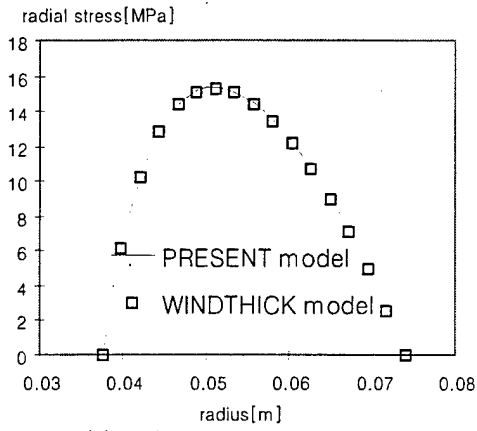
(a) radial stress of cylinder A
