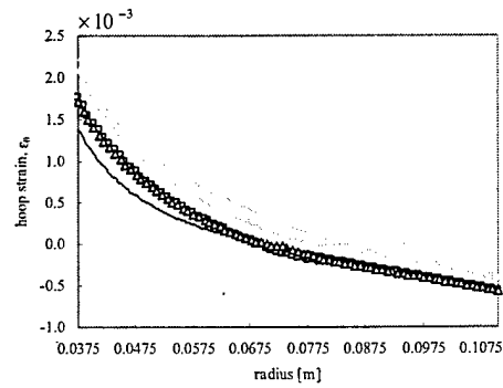
(e) hoop strains
