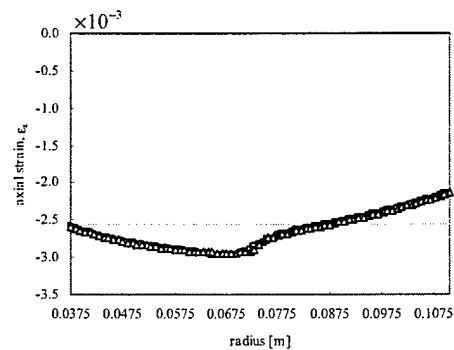
(f) axial strains
