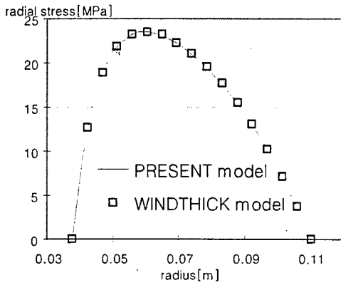
(c) radial stress of cylinder B
