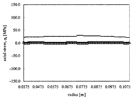
(c) axial stresses
