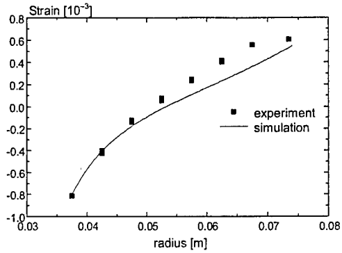
(b) hoop strain of Specimen A
