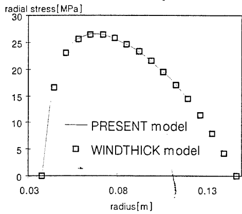
(e) radial stress of cylinder C
