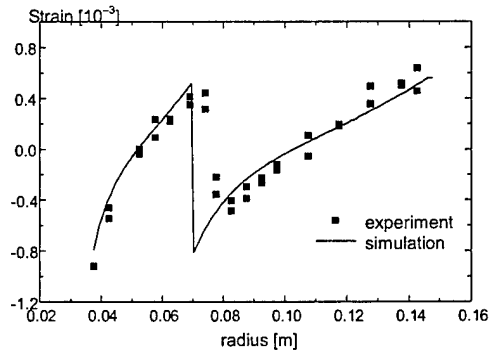
(f) hoop strain of Specimen C
