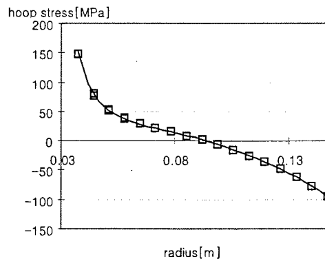
(f) hoop stress of cylinder C
