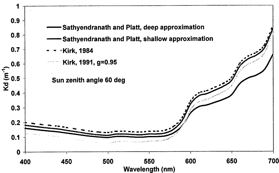
Figure 9. Comparison between different approximations for the attenuation coefficient of downwelling irradiance. Sun zenith angle \theta_s = 60 \text{ deg} . Phase function asymmetry parameter g = 0.95 .
