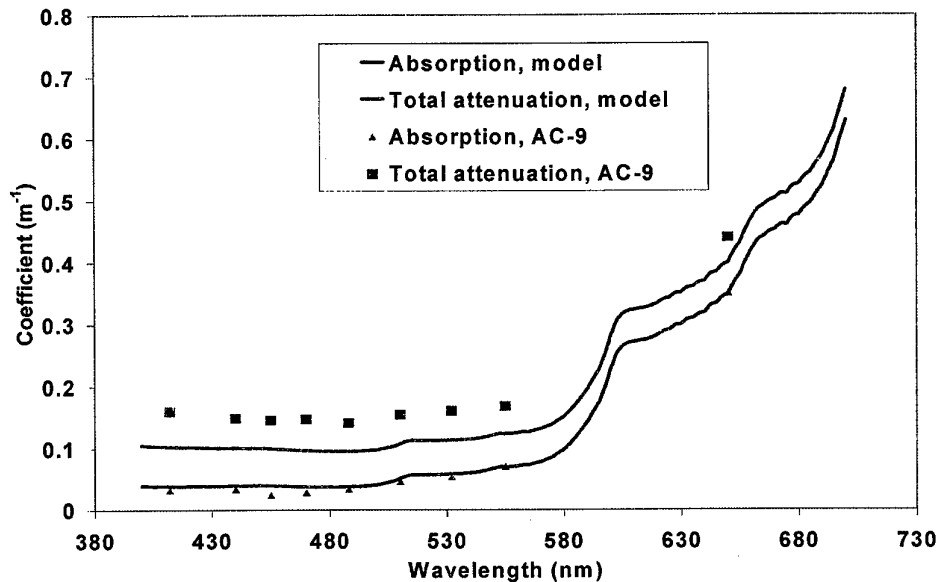
Figure 17. Comparison between the measured data and the one-parameter model for water off Kangaroo Island at depth of 5 m. The concentration of chlorophyll obtained from minimisation of (7.1) is 0.212 \text{ mg/m}^3 .
