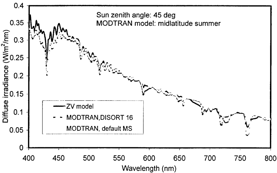
Figure 4. Diffuse irradiance at horizontal surface. Sun zenith angle is 45 degrees.
