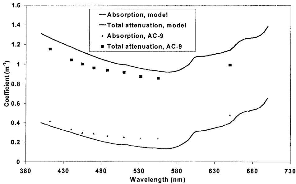
Figure 16. Comparison between the measured data and the one-parameter model for water at Cowley Beach at depth of 1.05 m. The concentration of chlorophyll obtained from minimisation of (7.1) is 2.89 mg/m 3 .
