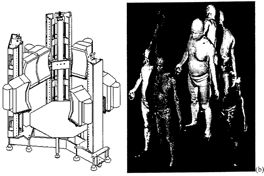
Figure 10. ITRI whole body scanner. (a) System schema, (b) multi-view merging and rendering of measured human body 3D data.
