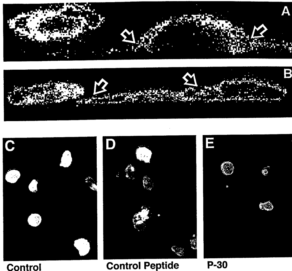
Fig. 3. Involvement of the galectin-1 (A) and galectin-3 (B) in the adhesion of the MDA-MB-435 human breast carcinoma cells to the monolayer of human umbilical endothelial cells as revealed by laser confocal microscopy. The X-Z sections shown were obtained as described in "Materials and Methods" using a \times 60 lens. The images were pseudocolored (green, galectin-1; red, galectin-3). Arrows, clustering toward the cell contacts of galectin-1 on cancer cells (A) and of galectin-3 on endothelial cells (B). The superimposed fluorescent photomicrographs of DiI-labeled MDA-MB-435 breast cancer cells adhered to the monolayer of HUVEC cells (C-E). There is an inhibition of the adhesion by 0.1 mg/ml of the T antigen-specific synthetic P-30 (E) but not by the same concentration of the control peptide (D) compared with the control (C).
