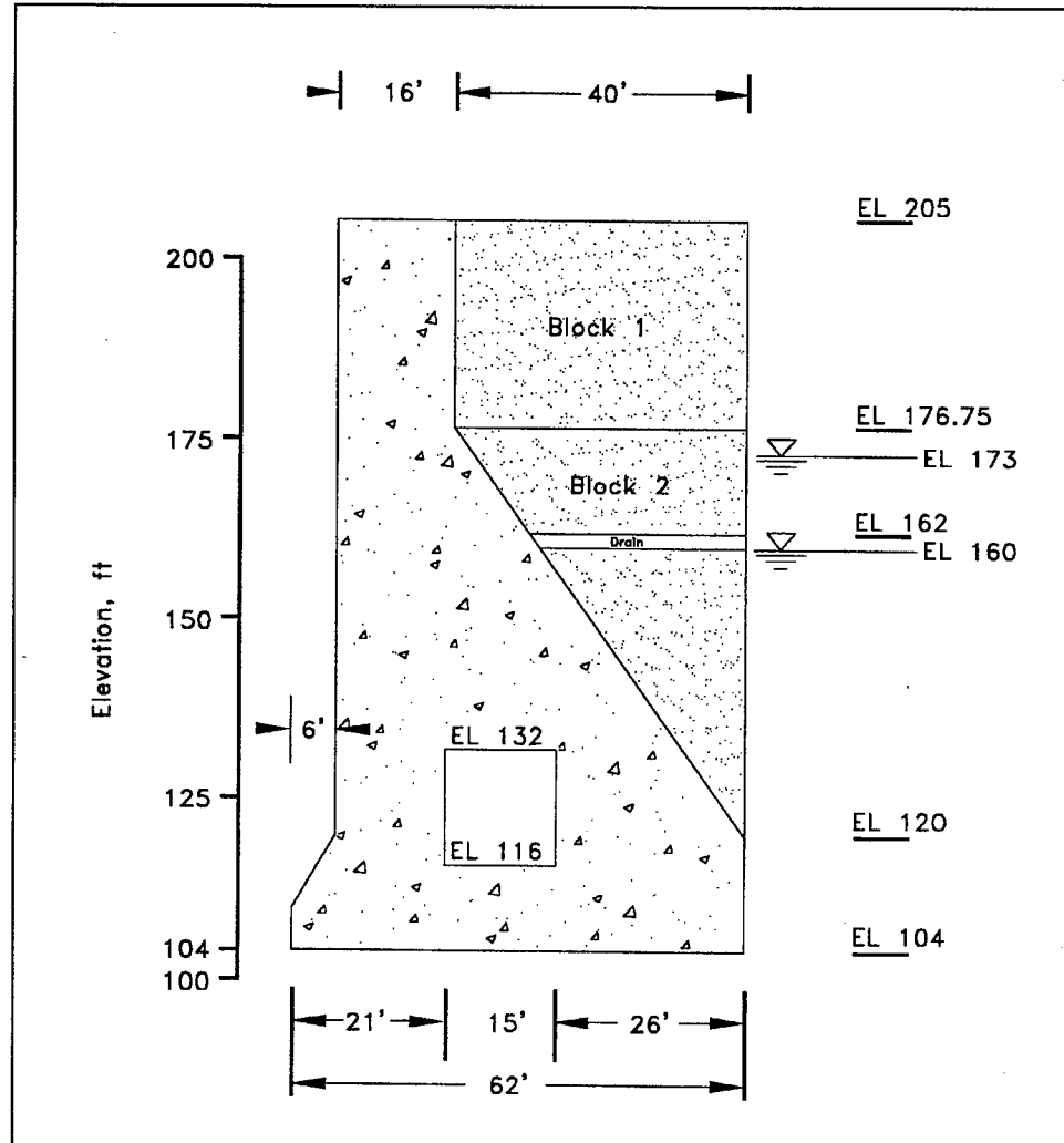
Figure A-1. Two blocks comprising the soil wedge behind Monolith N-56 at Snell Lock (1 ft = 0.305 m)
