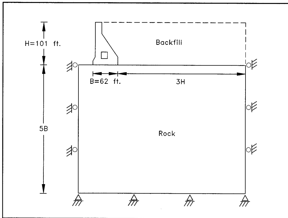
Figure 4-2. Snell Lock and elastic rock foundation model (1 ft = 0.305 m)
