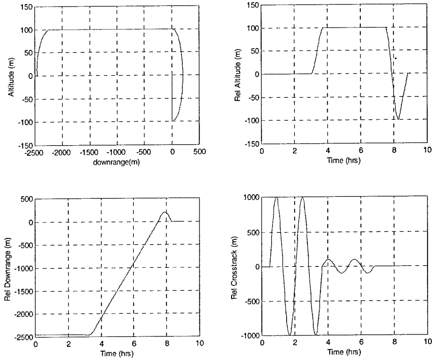
Figure 4-32: Hybrid trajectory 1 – R-bar final approach, \Delta V=3m/s
