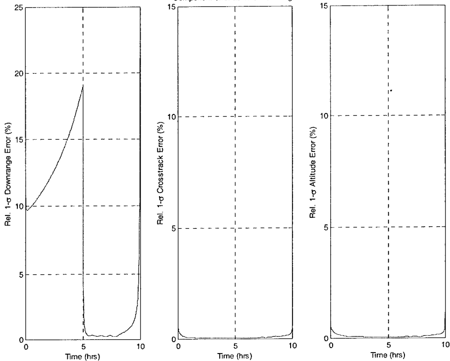
Figure 4-20: Relative position uncertainty for V-bar approach from 360m at 1cm/sec with 2 orbits of 100m cross-track motion starting at 5 hours, \Delta V=1.03m/s
