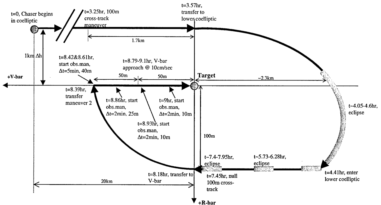
Figure 5-4: Orbital Express trajectory option 2 schematic
