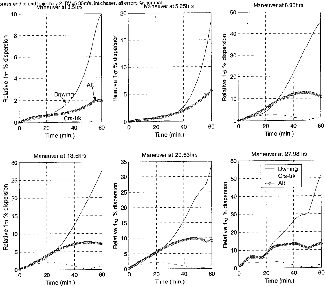
Figure 5-15: Relative position dispersions resulting from velocity uncertainty at maneuver execution times for Orbital Express end-to-end trajectory
