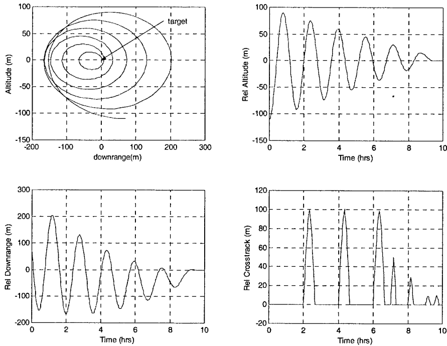
21-Jan-2001, spiral, 0rshrinking, hshrinking, ertmotion, ult, bs Spiral w/10mshrinking delta h and shrinking vert motion from 100m, Mult Observation Man., DV=1.55m/s
