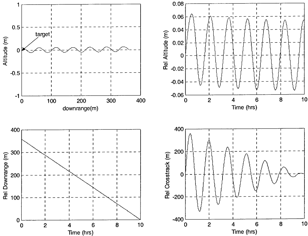
18-Jan-2001, vbar_60mback_cmsec_amped_cross_track Vbar approach from 360m @ 1cm/sec, Damped cross-track oscillations, DV=1.59m/s
