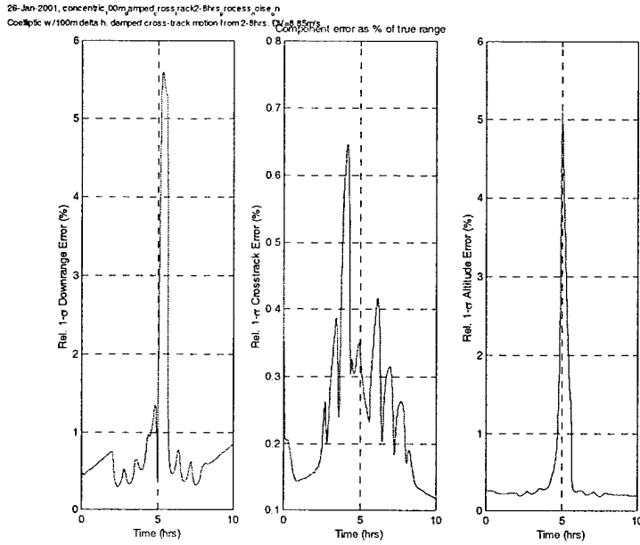
Figure 4-28: Relative position uncertainty with process noise for Coelliptic with 100m \Delta h and damped cross-track oscillations symmetric with respect to flyby point from 2-8 hours, \Delta V=8.85m/s
