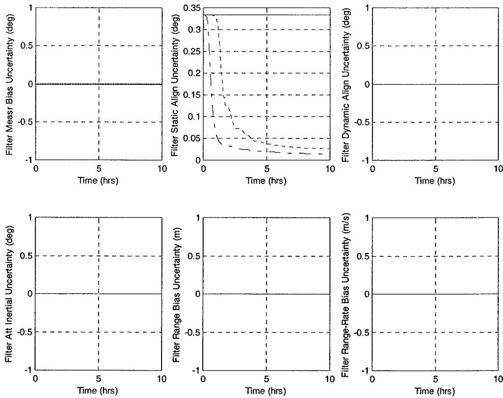
11-Apr-2001, football_00mback_0rmdelh_st1err Stn-keeping football 100m away w/ +/- 10m vert. motion, 1 deg/axis 3sig. static alignment error
