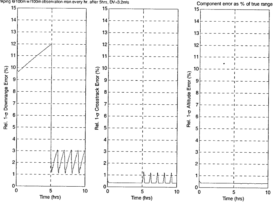
Figure 4-18: Relative position uncertainty with process noise for Co-circular station-keeping 100m away with 100m observation maneuvers every hour starting at 5 hours, \Delta V=3.2m/s
