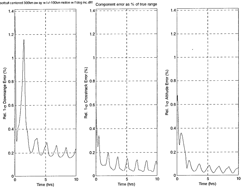
Figure 3-19: Relative position uncertainty for Football station-keeping 300km away with 100km vertical motion and 100km cross-track motion
