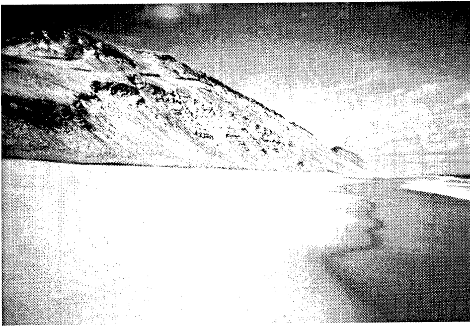
Figure 6. Coastal bank eroding due to wave action providing sediment to beaches and dunes, Wellfleet, Massachusetts
