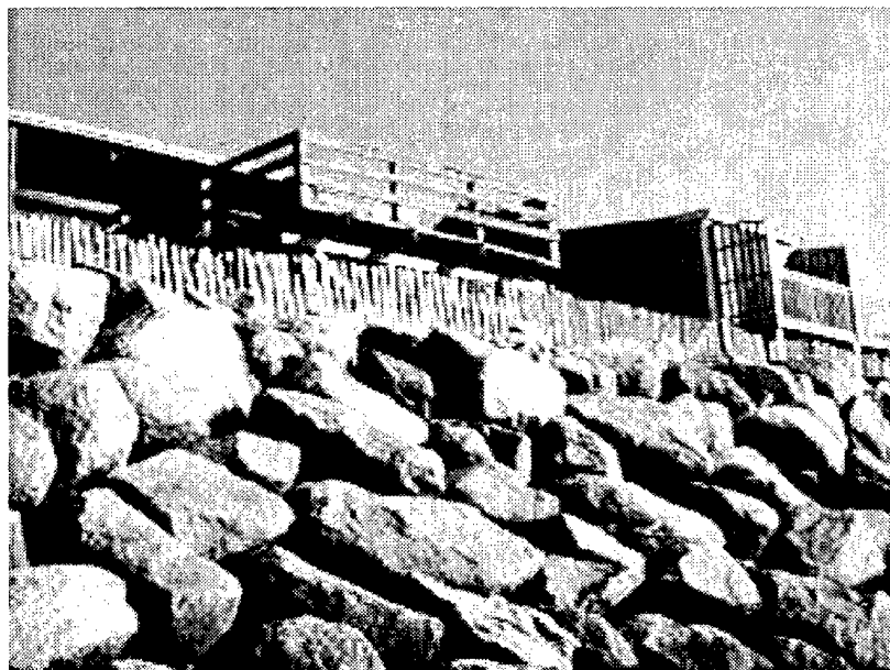
Figure 11. Revetment constructed of stone riprap on a coastal bank
