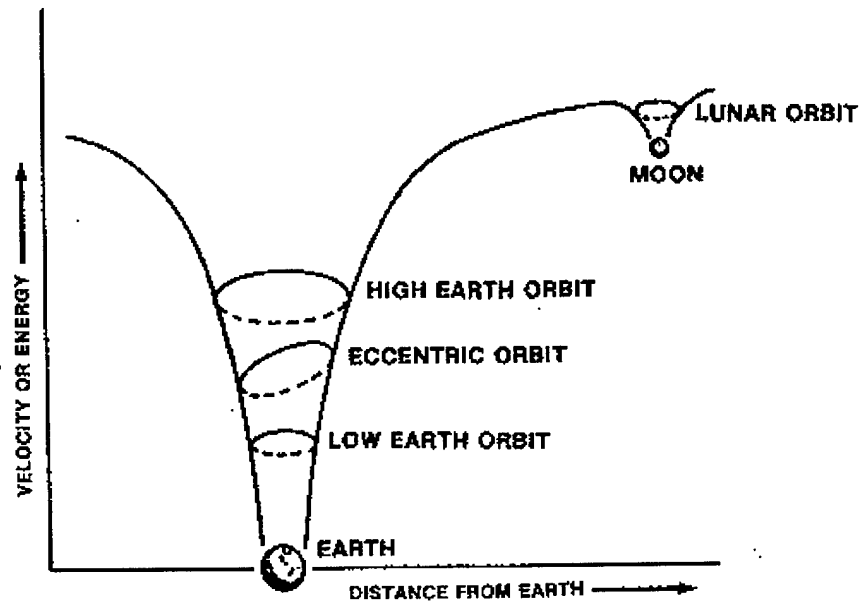
Figure 23. Gravity Wells
