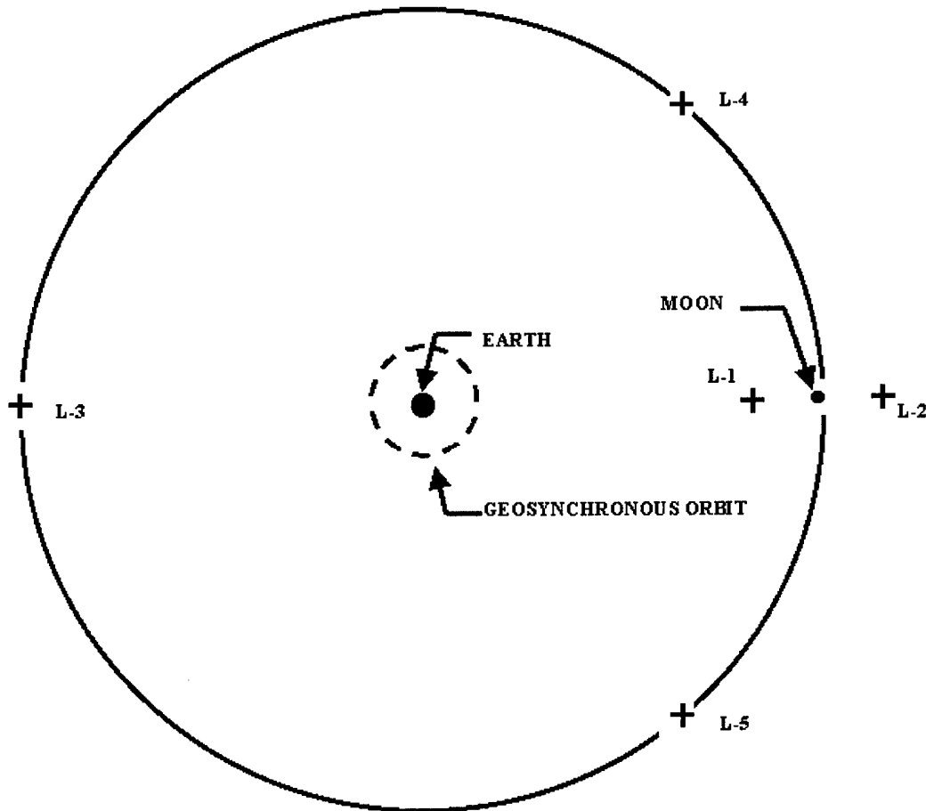
Figure 1. Lagrangian Points in the Earth Moon System
