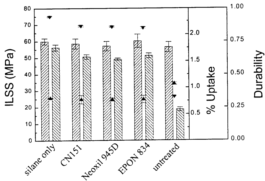
Figure 9. ILSS (dry = left bar, wet = right bar, for given film former), equilibrium moisture uptake percentage at 50 °C (percent uptake = up triangles), and durability (ratio of wet ILSS to dry ILSS = down triangles) for pultruded rod composites with MPS coupling agent and varying film former reactivity towards the matrix vinyl ester resin.
