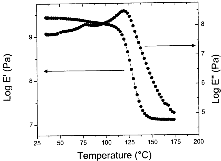
Figure 8. DMA of the vinyl ester matrix showing a glass transition temperature of approximately 125 °C.
