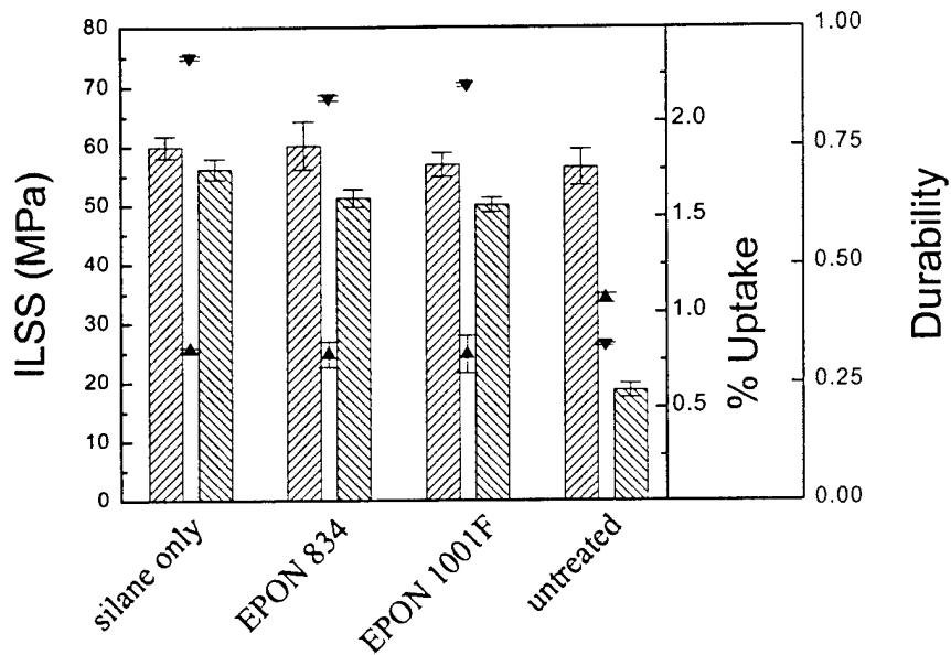
Figure 12. ILSS (dry = left bar, wet = right bar, for given film former), equilibrium moisture uptake percentage at 50 °C (percent uptake = up triangles), and durability (ratio of wet ILSS to dry ILSS = down triangles) for pultruded rod composites with MPS coupling agent and varying film former molecular weights.
