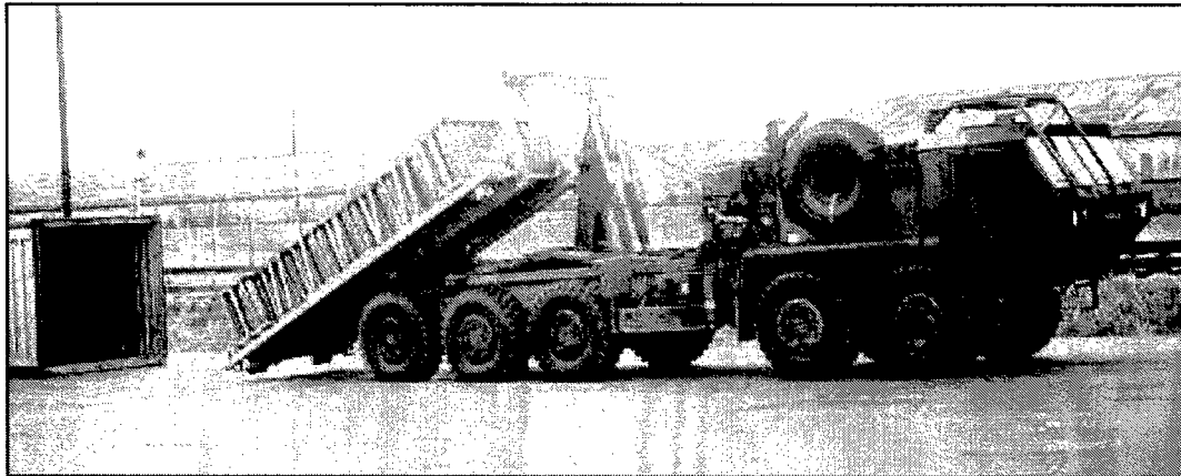
Figure 4. Removing a munition load from an ISO container, using the CROP platform and the PLS loading system
