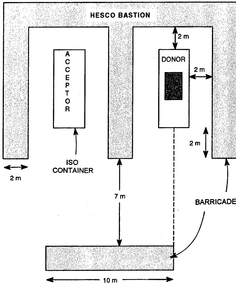
PLAN VIEW
