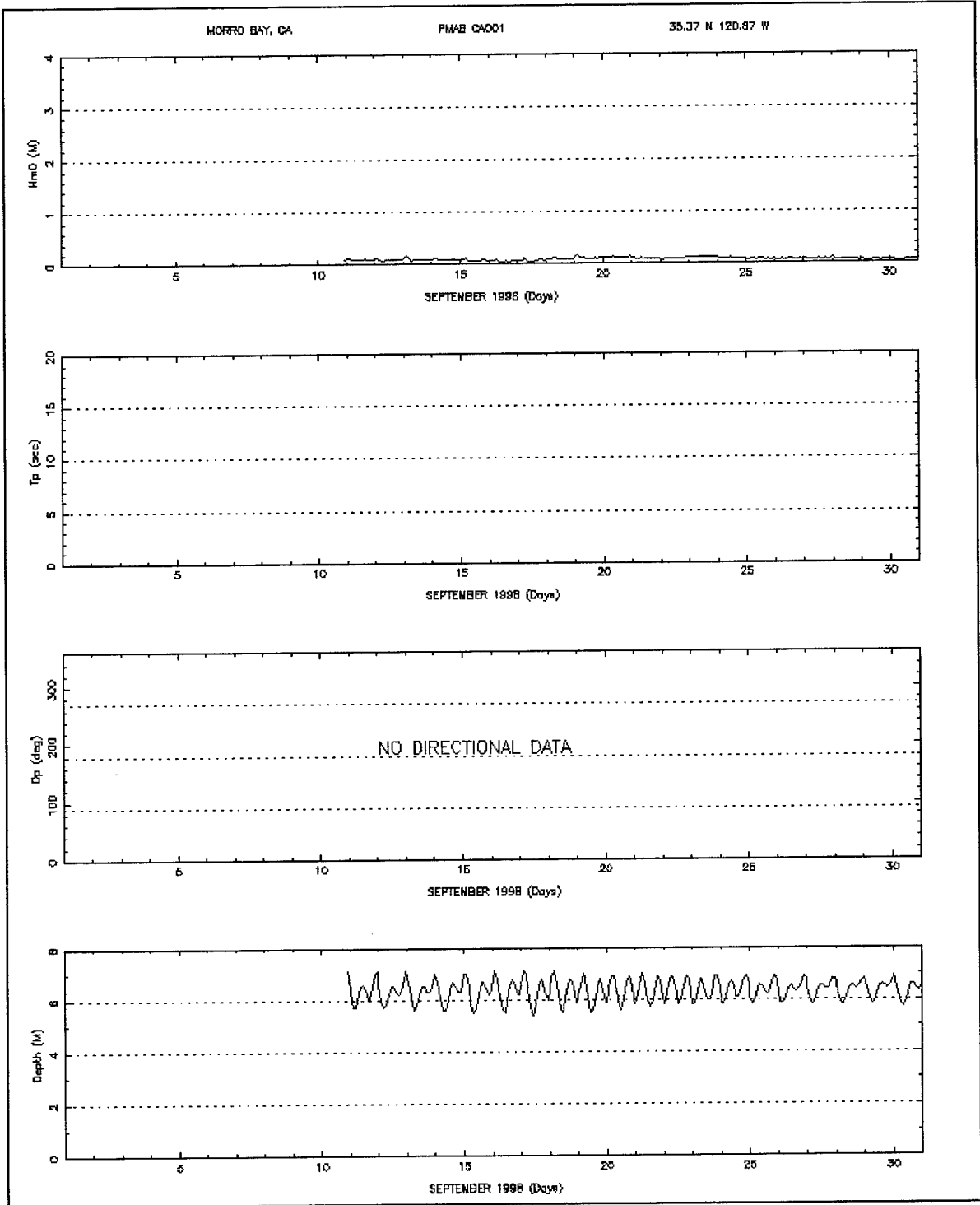
Figure 24. September 1998 monthly time series (CA001)
