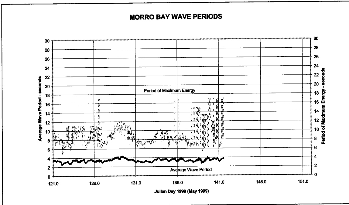
Figure 16. May 1999 average wave periods and periods of maximum energy
