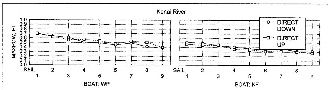
Figure 41. MAXPOW vs. direction vs. distance, high power
