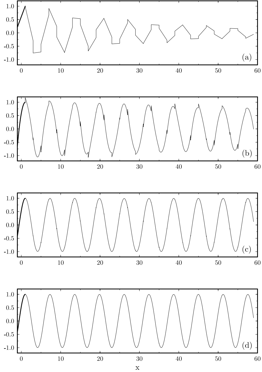
FIG. 4.3. Eigen-functions of the physical mode. K = 2 . \gamma = 0.5 . (a) p = 1 , (b) p = 2 , (c) p = 3 , (d) p = 4 .
