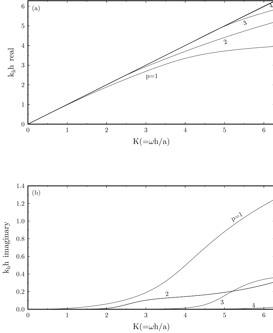
FIG. 4.1. The physical mode, numerical wave number k_h h v.s. actual wave number (normalized frequency) K = \frac{\omega h}{a} . \gamma = 0.5 .
