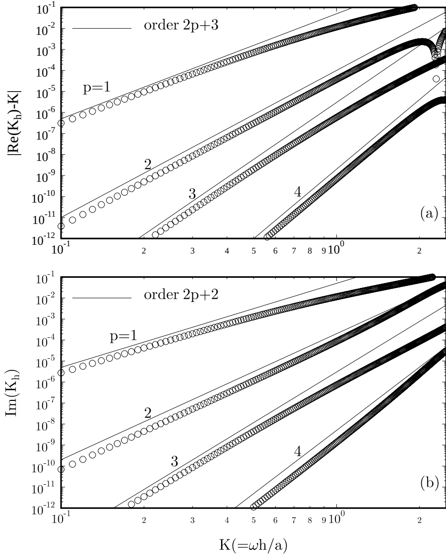
FIG. 4.6. Local order of convergence for the dispersion and dissipation errors of the physical mode. Circle: numerical wave number computed by equation (4.2); solid line: theoretical convergence rate. (a) dispersion error; (b) dissipation error. \gamma = 0.5 .
