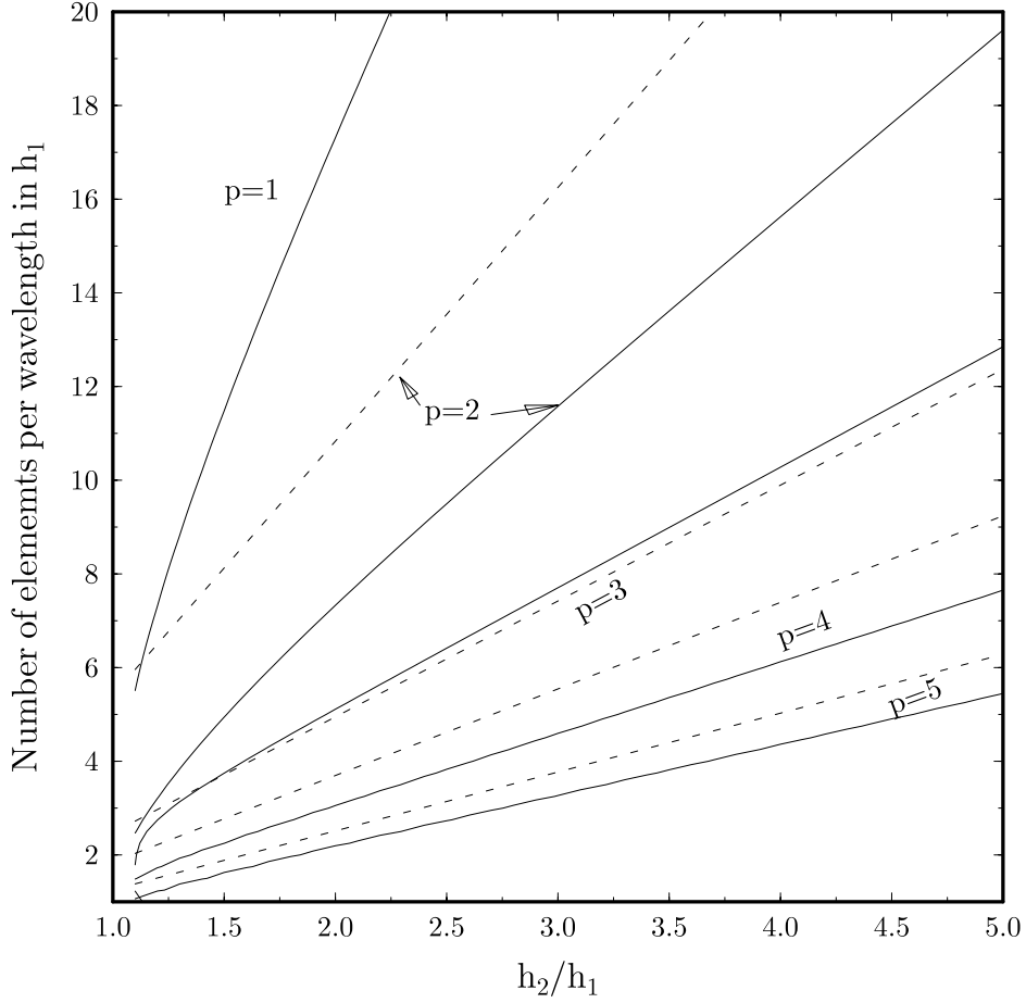
FIG. 5.2. Solid lines, boundaries of 2% numerical reflection. Reflected wave is less than 2% of the incident wave for parameters above the curves. \gamma = 0.5 . Dashed lines, accuracy limits determined from the dispersion relation of a uniform grid h_2 . The accuracy limit for p = 1 (not shown) is far above and out of the picture.
