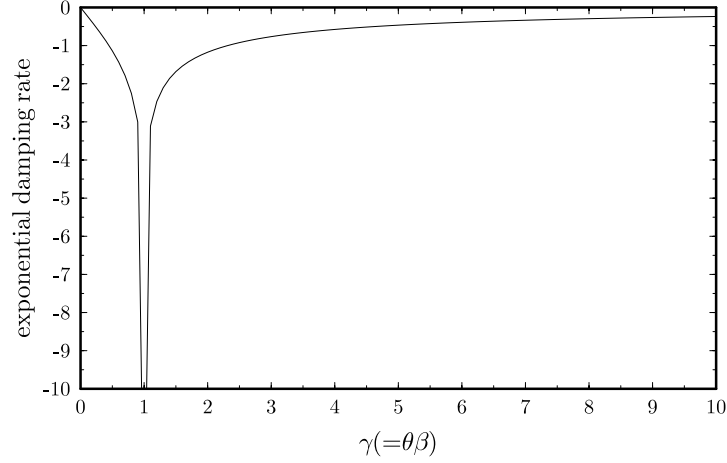
FIG. 4.5. Effects of \gamma on the damping rate of the spurious mode.
