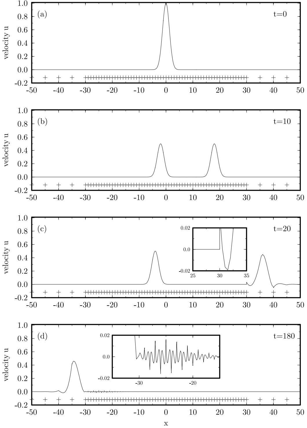
FIG. 6.4. Propagation of an acoustic pulse in a mean flow of M = 0.8 , using Lax-Friedrich flux formula (2.9) with \theta = 1 . Inserts indicate magnified ranges of interest.
