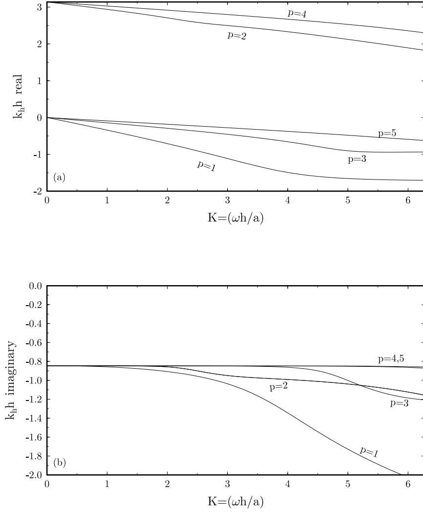
FIG. 4.2. The spurious mode, numerical wave number k_h h v.s. actual wave number (normalized frequency) K = \frac{\omega h}{a} . \gamma = 0.5 .
