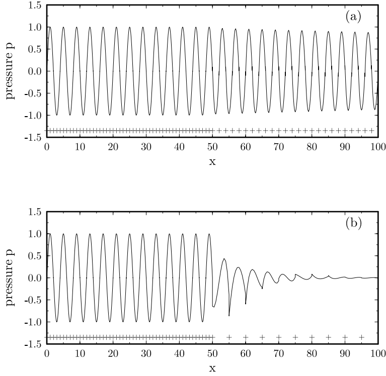
FIG. 6.2. Propagation of a periodic sine wave through a grid discontinuity at x = 50 . M = 0 , \gamma = 1 (exact characteristics flux). + indicates grid points. (a) h_1 = 1 , h_2 = 2 ; (b) h_1 = 1 , h_2 = 5 .
