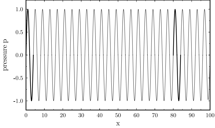
FIG. 6.1. Propagation of a periodic sine wave. The difference of the solutions at two periods shown in dark lines are computed in Table 6.1.
