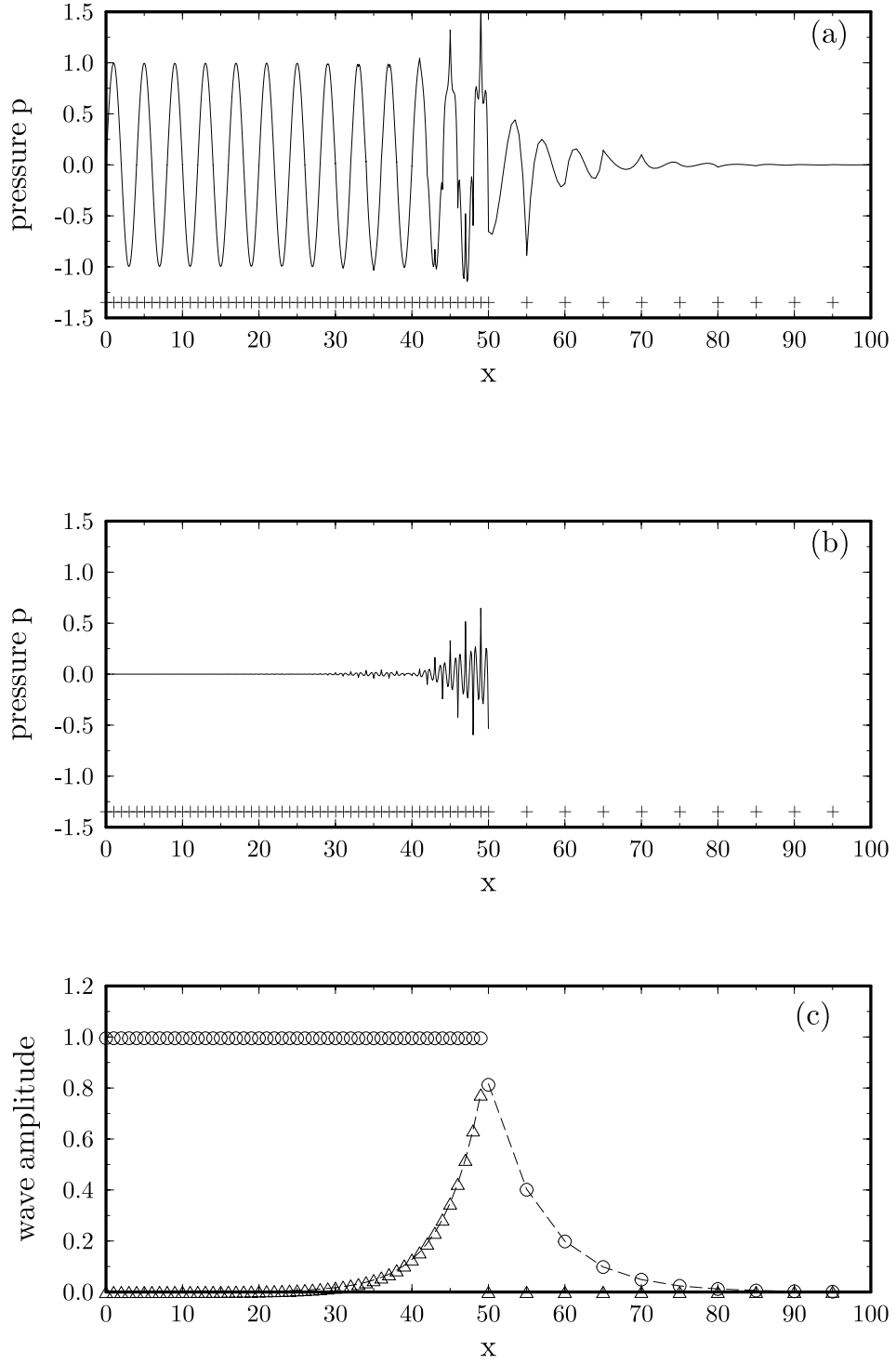
FIG. 6.3. (a) Propagation of a sine wave through a grid discontinuity, h_2/h_1 = 5 , \gamma = 10 . (b) Reflected wave. (c) Decomposition of numerical solution into physical and spurious modes. circles, physical mode; triangles, spurious mode; dashed lines, theoretical predictions of (5.13)-(5.14).
