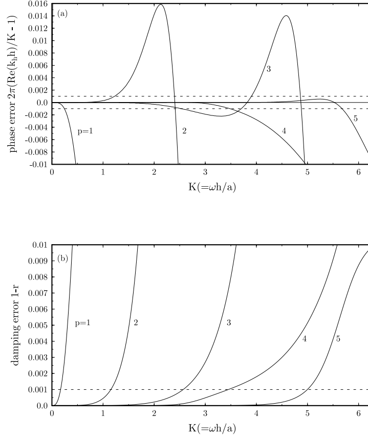
FIG. 5.3. Enlarged numerical phase (a) and damping (b) errors per wavelength of propagation for the physical mode. k_h is the numerical wave number and K is the exact wave number. r = e^{-2\pi \text{Im}(k_h h)/K} is the wave amplitude damping factor. The dotted lines indicate the accuracy limits used in plotting Figure 5.2.
