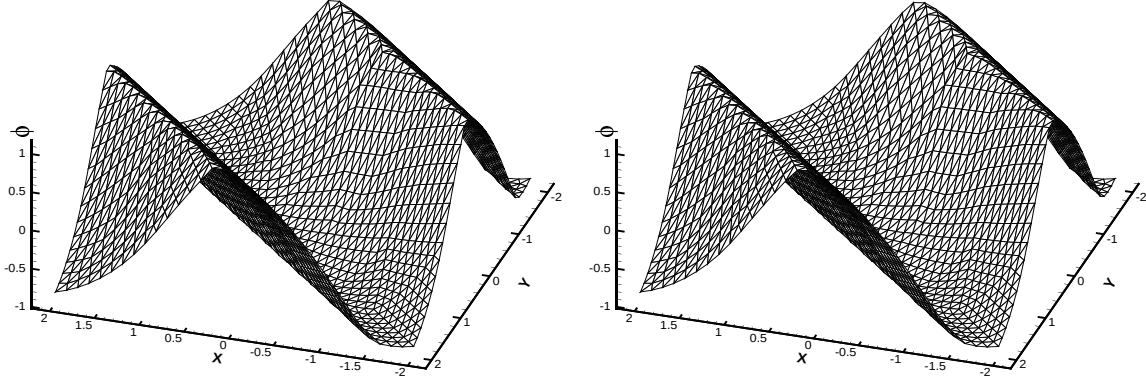
4th-order Linear Scheme, 1473 nodes
