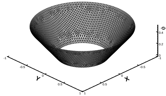
FIG. 3.21. The steady state solution for level set equation using the fourth order WENO scheme.
