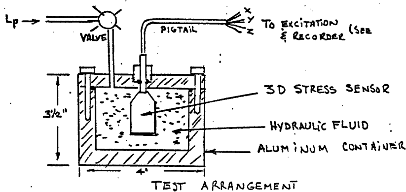
3D SENSOR FLUID-COUPLED #1
