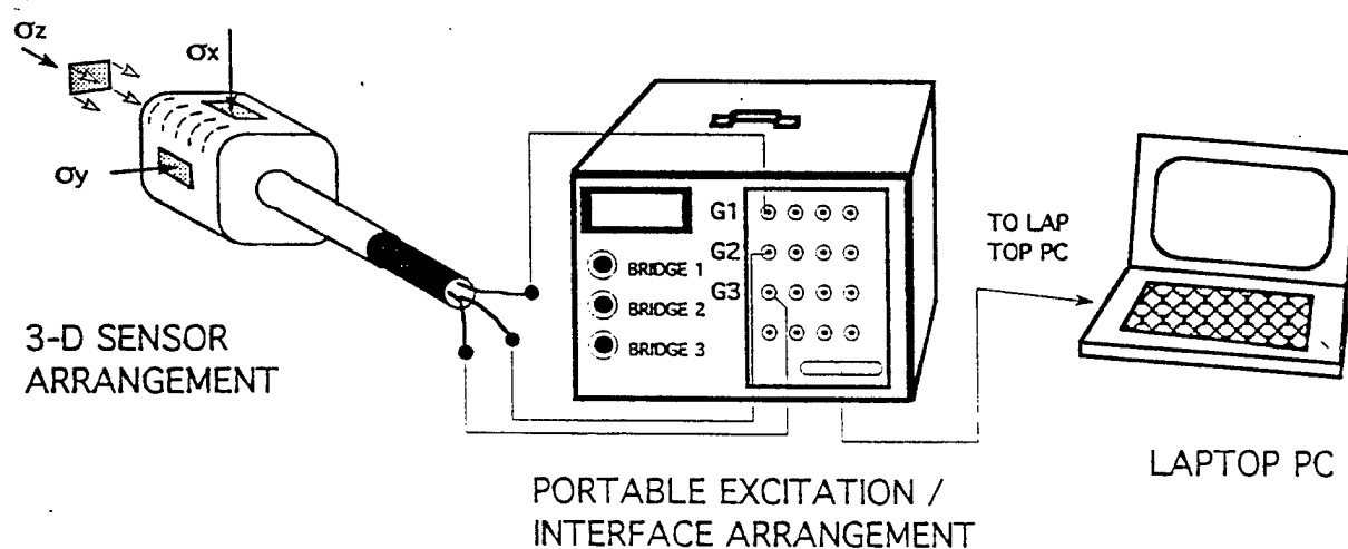
Fig. 1. Field-Portable 3D In-situ Stress Measurement System.
