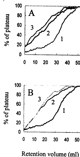
Fig. 2. The effect of MQ enantiomers on the frontal affinity chromatography of 1.0 nM [ ^3\text{H} ]-VBL on the Pgp-SP where: (A) Trace 1: [ ^3\text{H} ]-VBL alone; Trace 2: 200 nM (+)-MQ added to the running buffer; Trace 3: 200 nM (+)-MQ plus 3 mM ATP added to the running buffer. (B) Trace 1: [ ^3\text{H} ]-VBL alone; Trace 2: 200 nM (–)-MQ added to the running buffer; Trace 3: 200 nM (–)-MQ plus 3 mM ATP added to the running buffer. The running buffer was 50 mM Tris-HCl (50 mM, pH 7.4).
