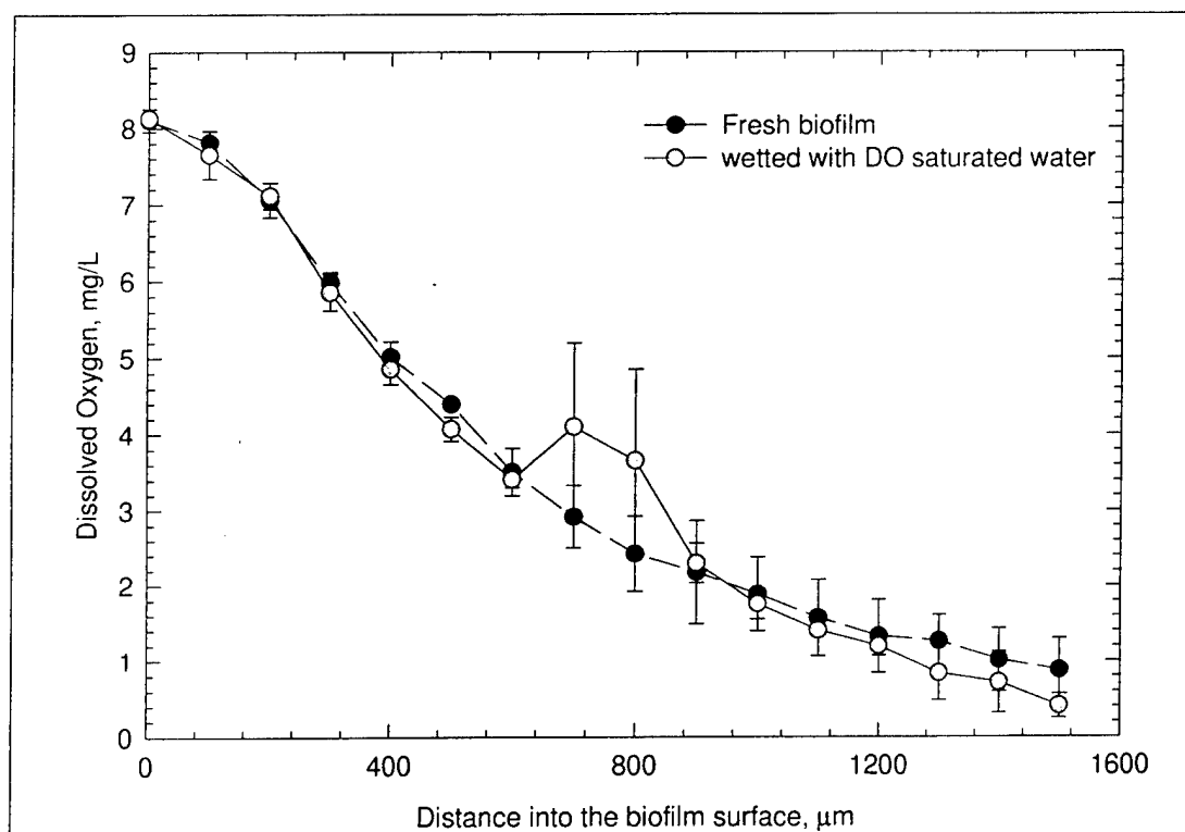
Figure 32. Effect of dropping DO-saturated water on biofilm.
