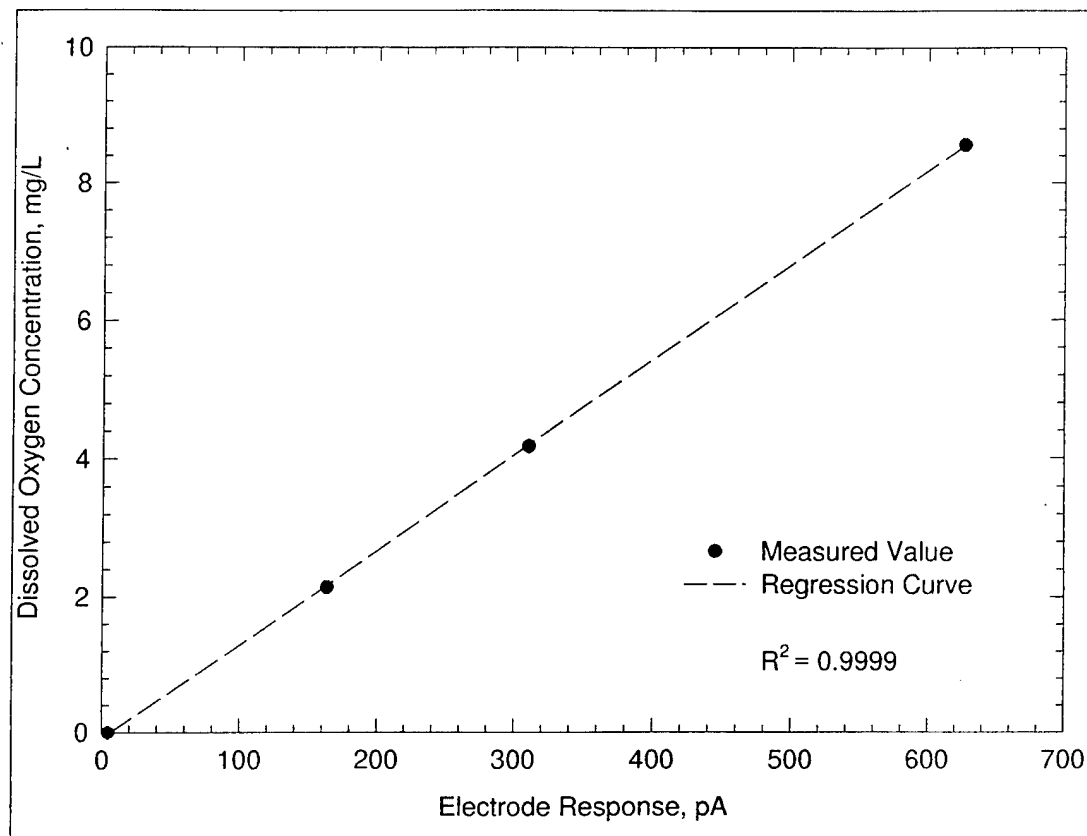
Figure 28. Calibration curve of the oxygen microelectrode.
