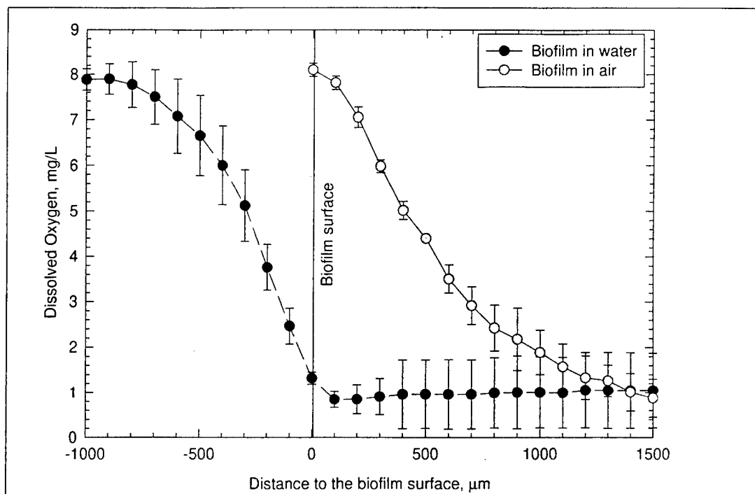
Figure 33. Comparison of oxygen profiles with biofilm in water and in air.
