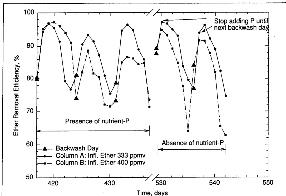
Figure 49. Comparison of biofilter performance with and without phosphorous in nutrient feed.
