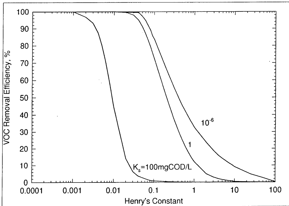
Figure 38. Effect of Monod constant vs effect of Henry's constant on VOC removal.
