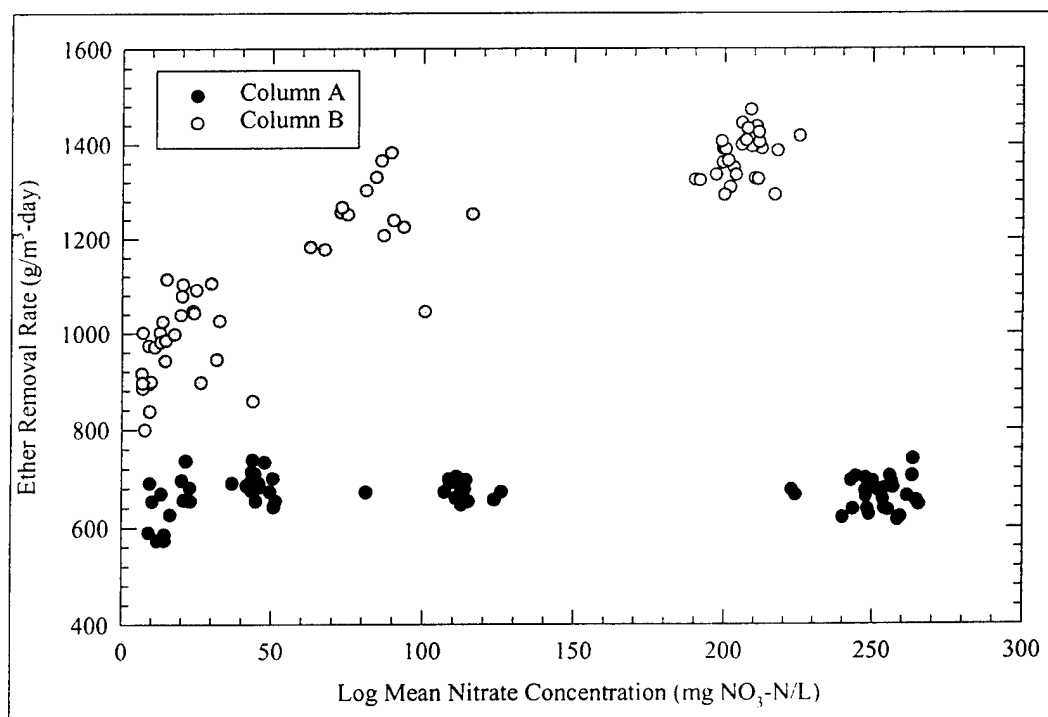
Figure 12. Effect of logmean nitrate concentration on ether removal rate.
