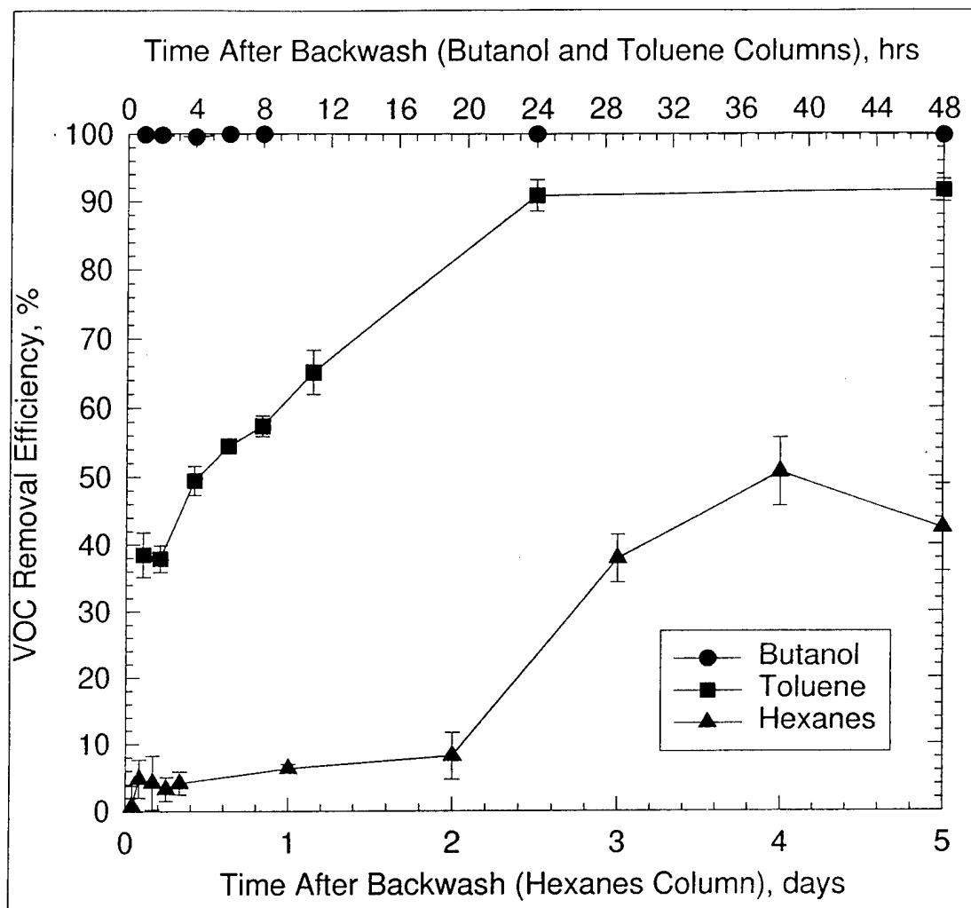
Figure 36. Influence of backwash on different VOC removal at VOC loading of 2 kg/m 3 /day.
