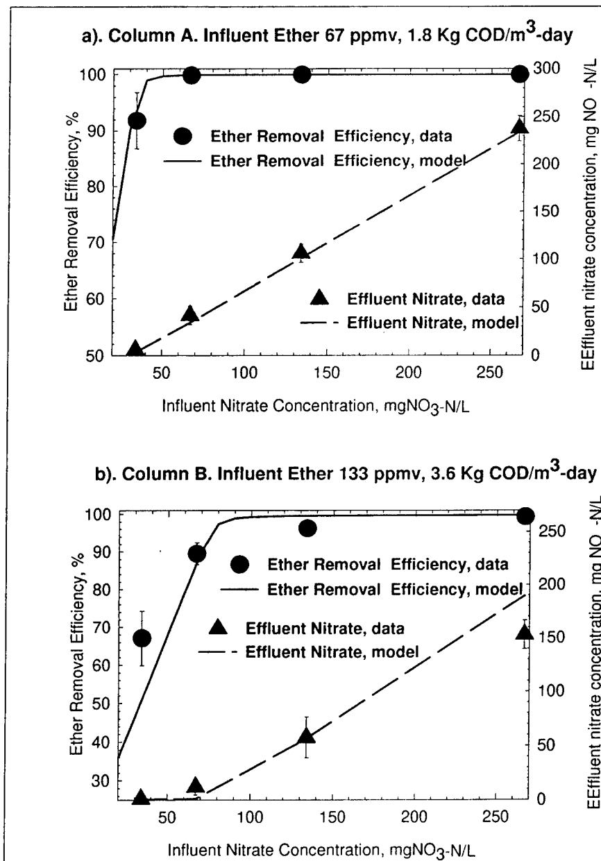
Figure 16. Model simulations of the effect of influent nitrate concentration.
