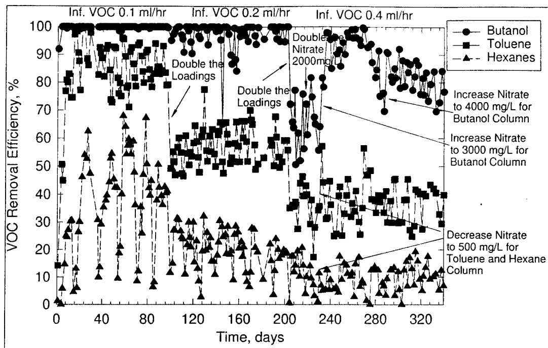
Figure 35. Effect of Henry's constant on biofilter performance.
