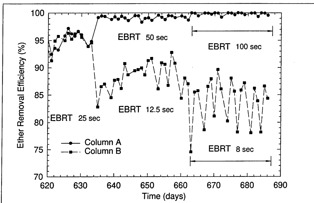
Figure 6. Effect of EBRT on biofilter performance at COD loading of 8.9 kg COD/m 3 /day.
