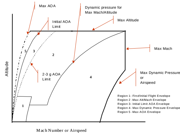
Figure 9 Typical Envelope Expansion Regions
