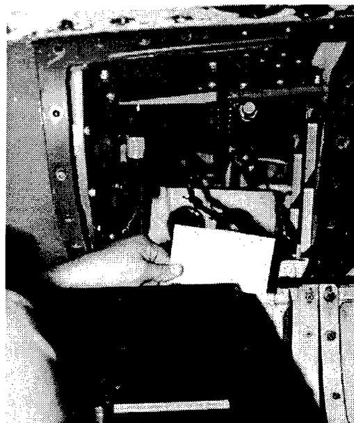
F-15 Data Monitor and Recorder Installation
