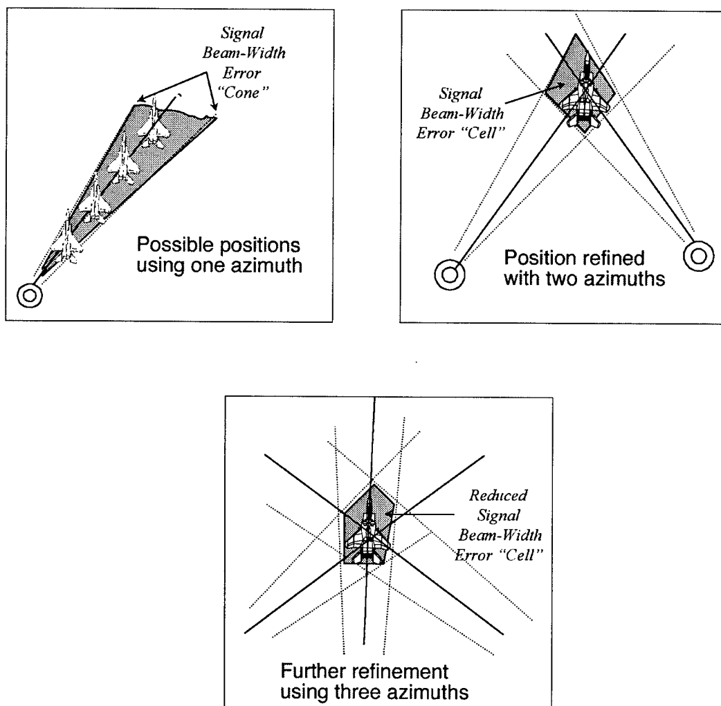
Figure 6. ACMI Position Using Multilateration Techniques
