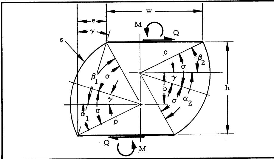
Figure 7. Shear Deformation.
