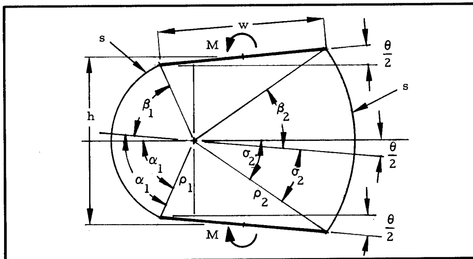
Figure 8. Roll Deformation.
