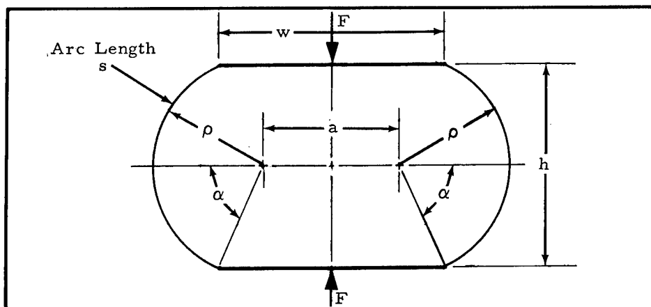
Figure 3. Lateral Compression Deformation.
