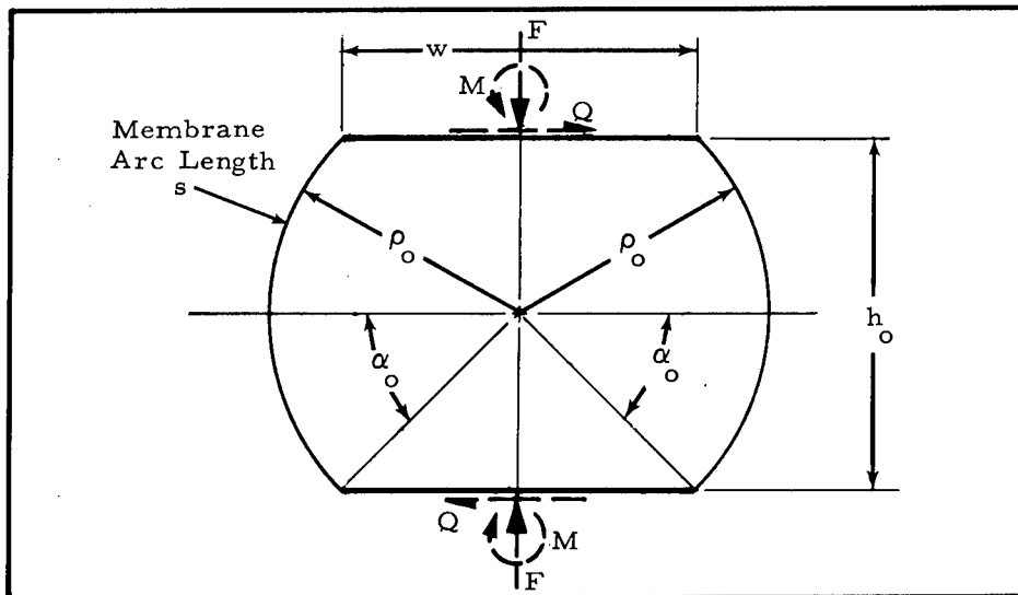
Figure 2. Initial Geometry of Cylindrical Element.
