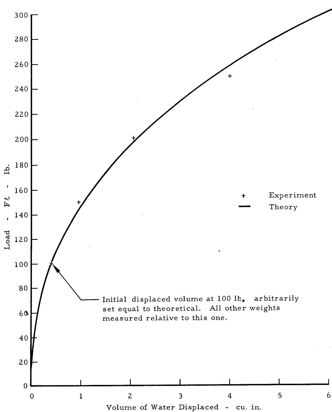
Figure 15. Compression Volume-Change Experiment.
