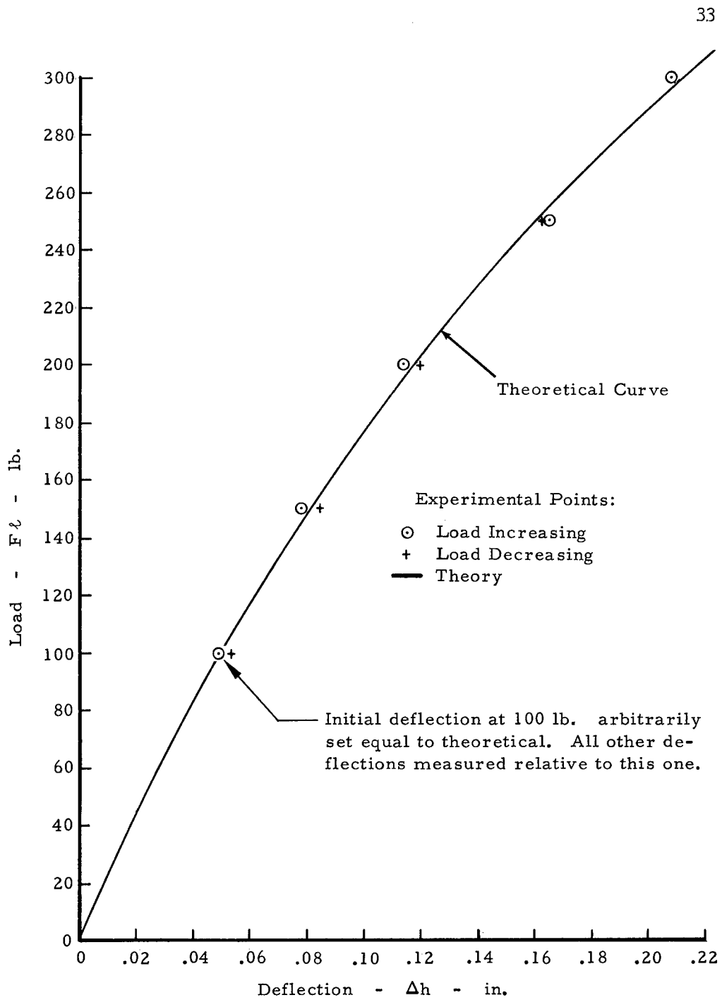
Figure 14. Compression Deformation Experiment.
