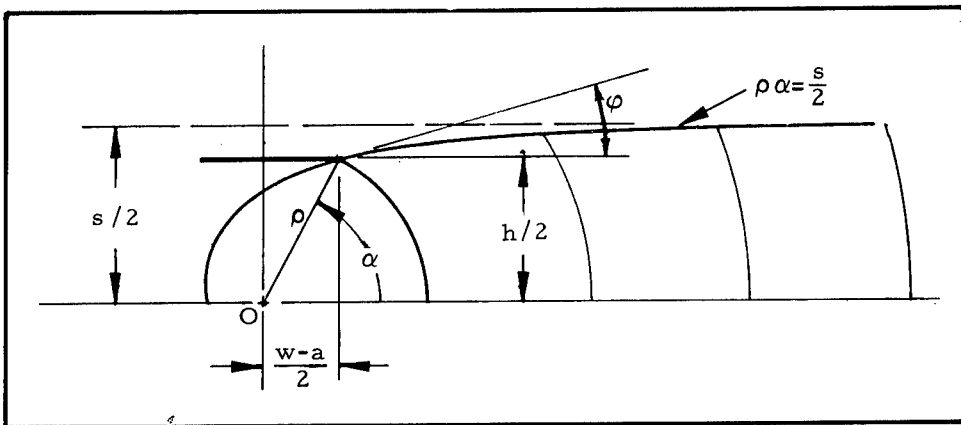
Figure 20. Hyperbolic Spiral.
