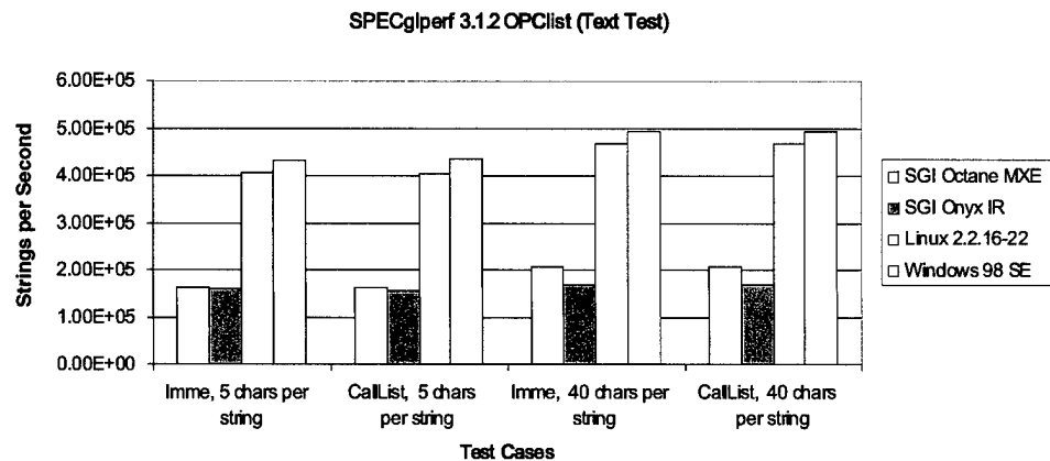
Figure 56. This graph shows the performance of the four target systems on rendering text strings in various modes.
