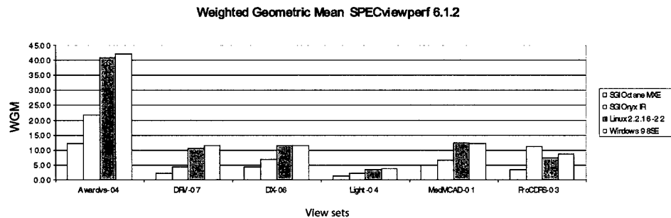
Figure 7. This graph shows the plotted WGM results for the six viewsets in SPECviewperf 6.1.2.
