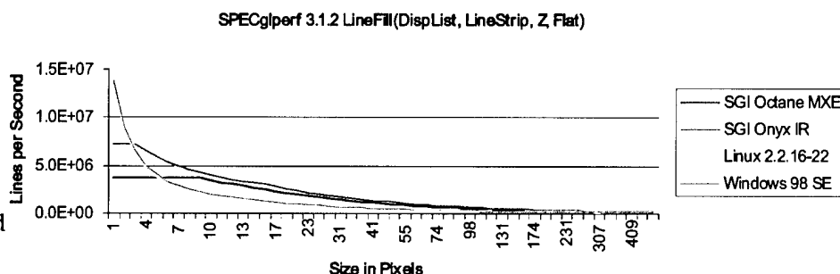
Figure 31. This graph shows the performance of the four target systems on rendering varying sizes of line strips in display-list, and flat shaded mode with the Z buffer turned on.
