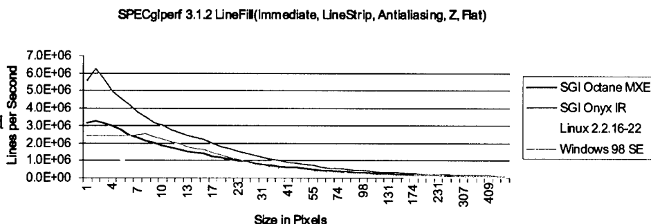
Figure 32. This graph shows the performance of the four target systems on rendering varying sizes of line strips in immediate, and flat shaded mode with both the Z buffer and antialiasing turned on.
