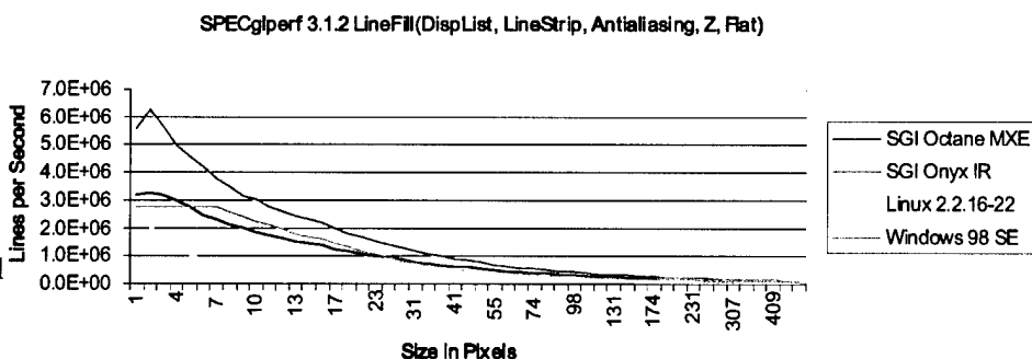
Figure 33. This graph shows the performance of the four target systems on rendering varying sizes of line strips in display-list, and flat shaded mode with the Z buffer turned on.
