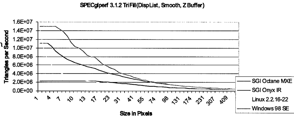
Figure 41. This graphs shows the performance of target systems on rendering triangles strips of varying sizes in display-list and smooth shaded mode with Z buffer turned on.
