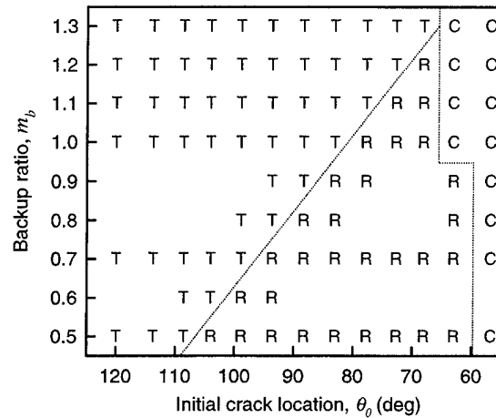
Fig. 9. Effect of backup ratio and initial crack location on crack failure modes, T=tooth fracture, R=rim fracture, C=compression (no crack propagation).
