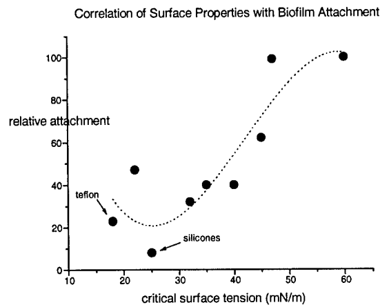
Figure 2-1. Graph illustrating the correlation between surface properties with biofilm attachment to those surfaces (from Baier 9 ).
