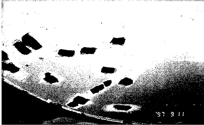
Figure 5-9. Application of toughening tie layer to deficient patches for repair of the NRL-GE duplex coating system.
