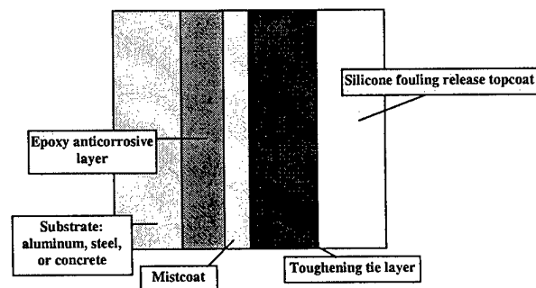
Figure 2-2. The NRL-GE duplex fouling release coating system.
