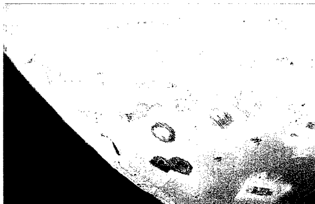
Figure 5-8. Application of adhesive repair package to damaged area of the NRL-GE duplex coating system.
