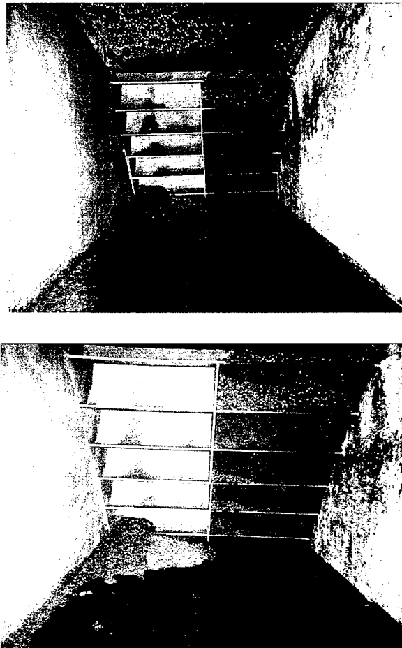
Figure 5-5. Effectiveness of the duplex coating system on intake walls and deflecting vanes in the Consumer Power D.E. Karn Unit #1 cooling water intake, Essexville, Michigan. The right-hand baffles are untreated steel fouled with zebra mussels and quagga mussels.
