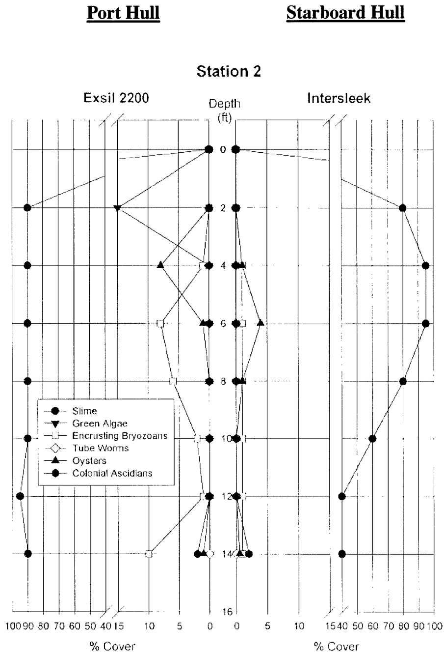
Figure 5-13. Vertical biofouling profile observed on SLICE hulls at Station 2 (forward location).
