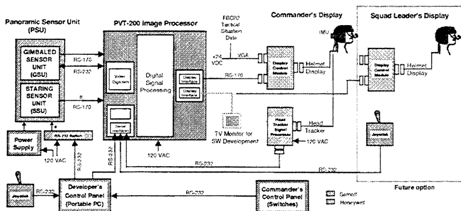
Figure 25. Prototype system block diagram
