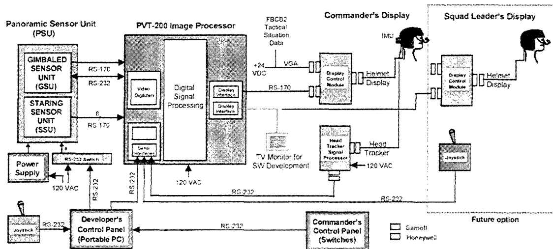
Figure 35. STTV system block diagram
