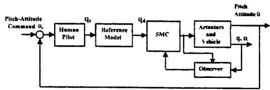
Figure 11 SMC system for pitch-attitude tracking
