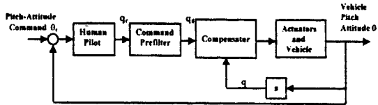
Figure 12 Ref. 21 system for pitch-attitude tracking
