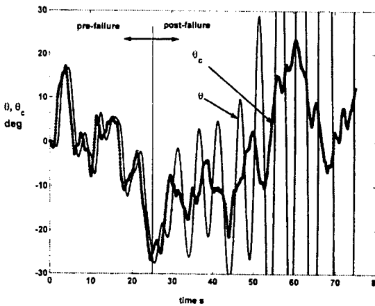
Figure 16 System of Fig. 12 (Ref. 21) pitch-attitude tracking before and after Failure No. 1
