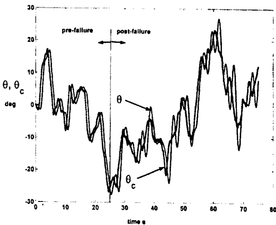
Figure 17 SMC pitch-attitude tracking before and after Failure No. 2
