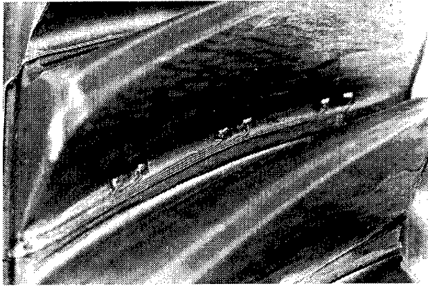
Figure 5.—Close-up of strain gage and associated wiring.
