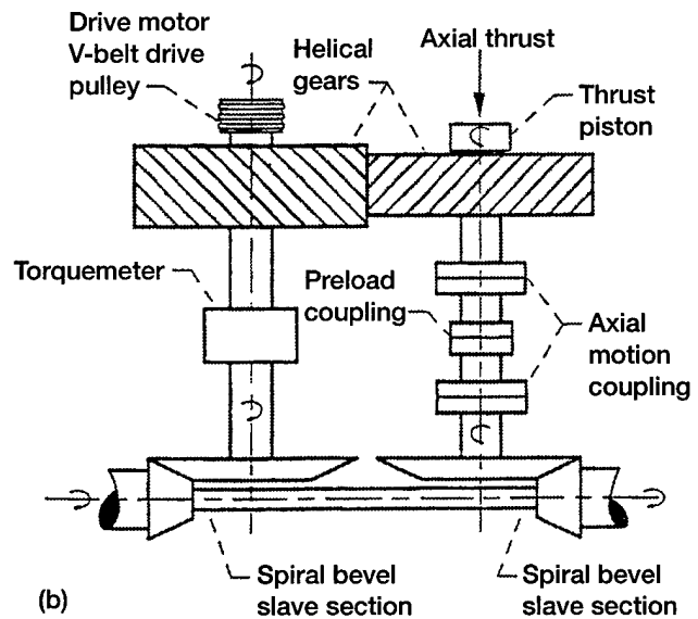
Figure 4.—NASA Glenn Research Center Spiral Bevel Gear Facility. (a) Sketch. (b) Facility cross section.
