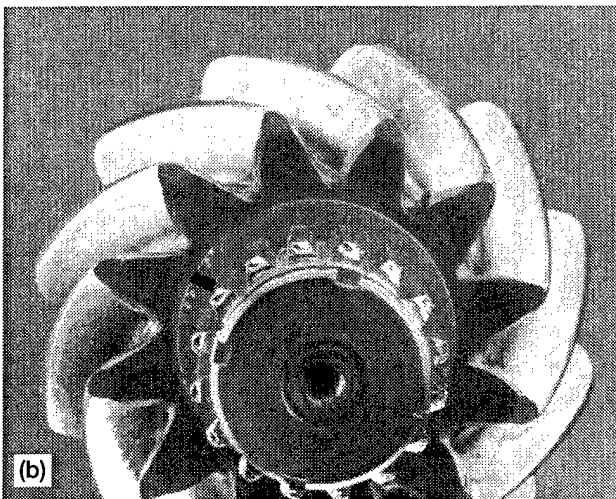
Figure 3.—Pinions. (a) Face-milled. (b) Face-hobbed.
