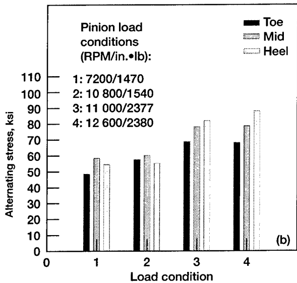
Figure 8.—Comparison of root gauge alternating stress magnitude across the face width of the two different pinions. (a) Face-milled. (b) Face-hobbed.
