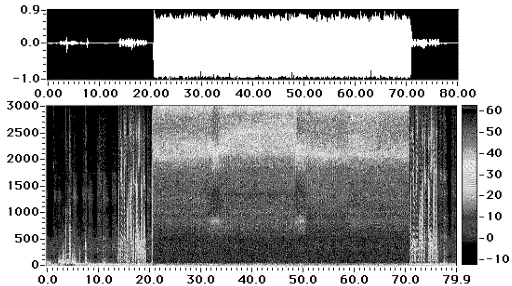
Figure 18: Boom microphone detecting voice in high noise environment (105 dB C).
