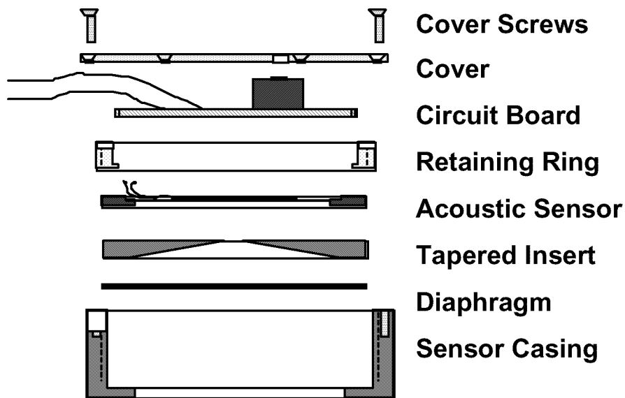
Figure 3: Sensor assembly drawing.
