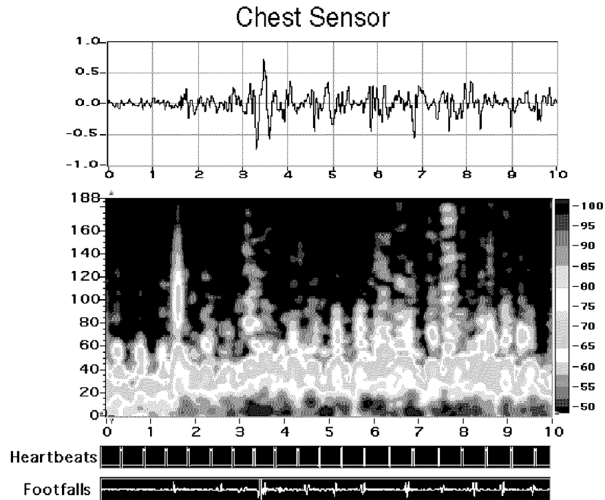
Figure 12: Chest data of soldier walking, heartbeats and footfalls in low-frequency region.
