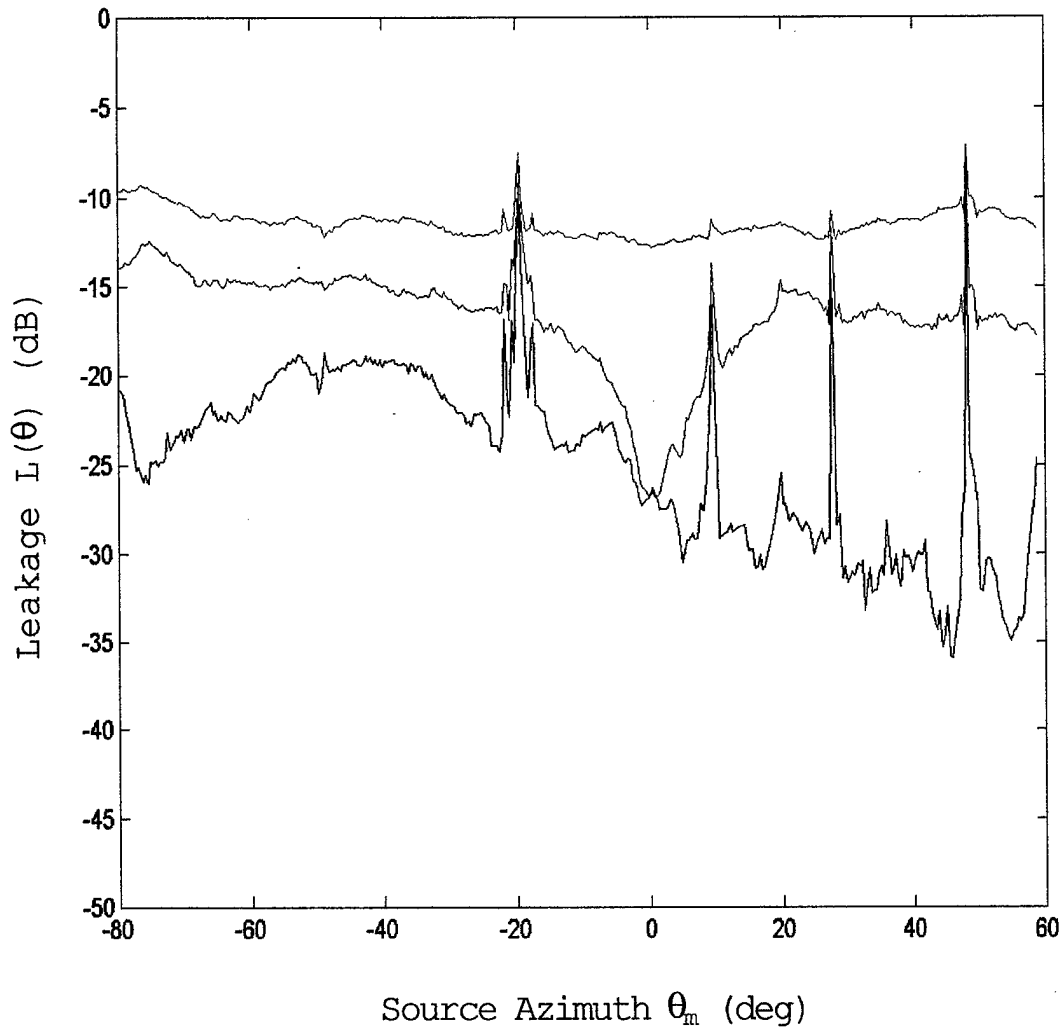
Figure 6: Leakage power calculated with C (black), phase-only matrix C P (red), and gain-and-phase matrix C GP (blue).
