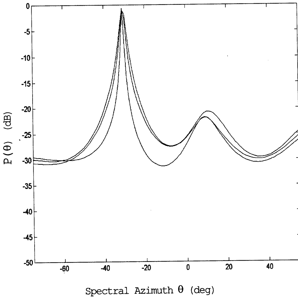
Figure 12c: Some directional spectra of synthetic snapshots with azimuth \theta_m \approx -30^\circ . Gain-and-phase matrix C_{GP} was used to calibrate the snapshots.
