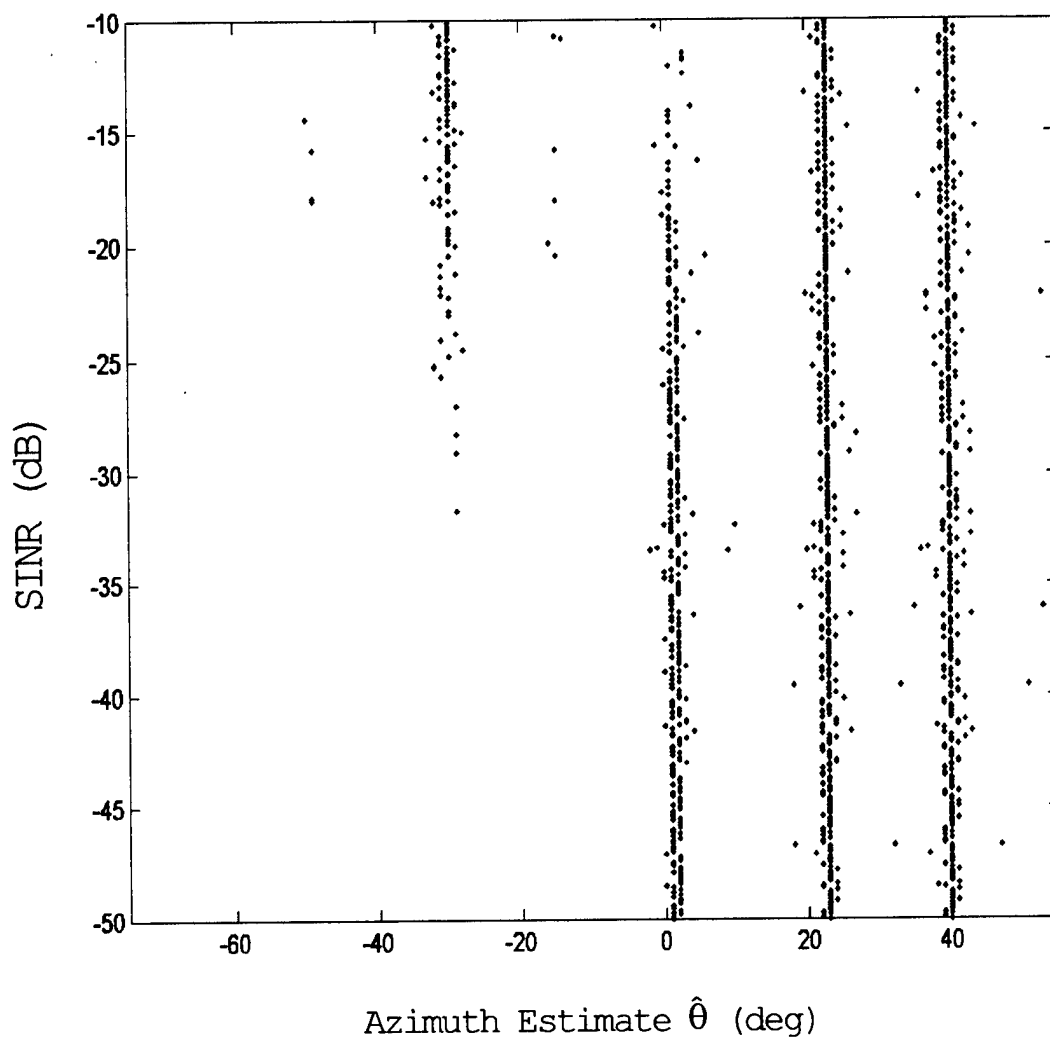
Figure 19c: DFT candidate direction estimates calculated with gain-and-phase matrix C_{GP} and the synthetic snapshots.
