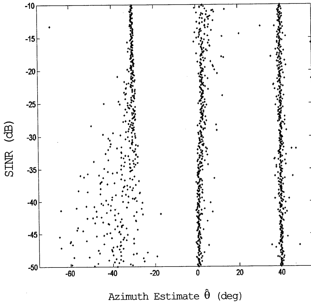
Figure 16c: Candidate direction estimates calculated with the synthetic snapshots used to produce Figure 14c. Gain-and-phase matrix C_{GP} was used to calibrate the snapshots.
