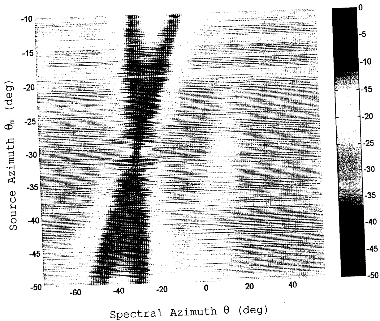
Figure 11c: Directional spectra of two equal-strength intersecting targets. Gain-and-phase matrix C_{GP} was used to calibrate the snapshots.
