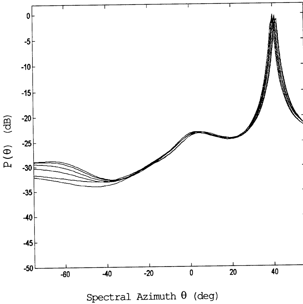
Figure 9c: Directional spectra of six array snapshots with source azimuth \theta_m \approx 40^\circ . Gain-and-phase matrix C_{GP} was used to calibrate the snapshots.
