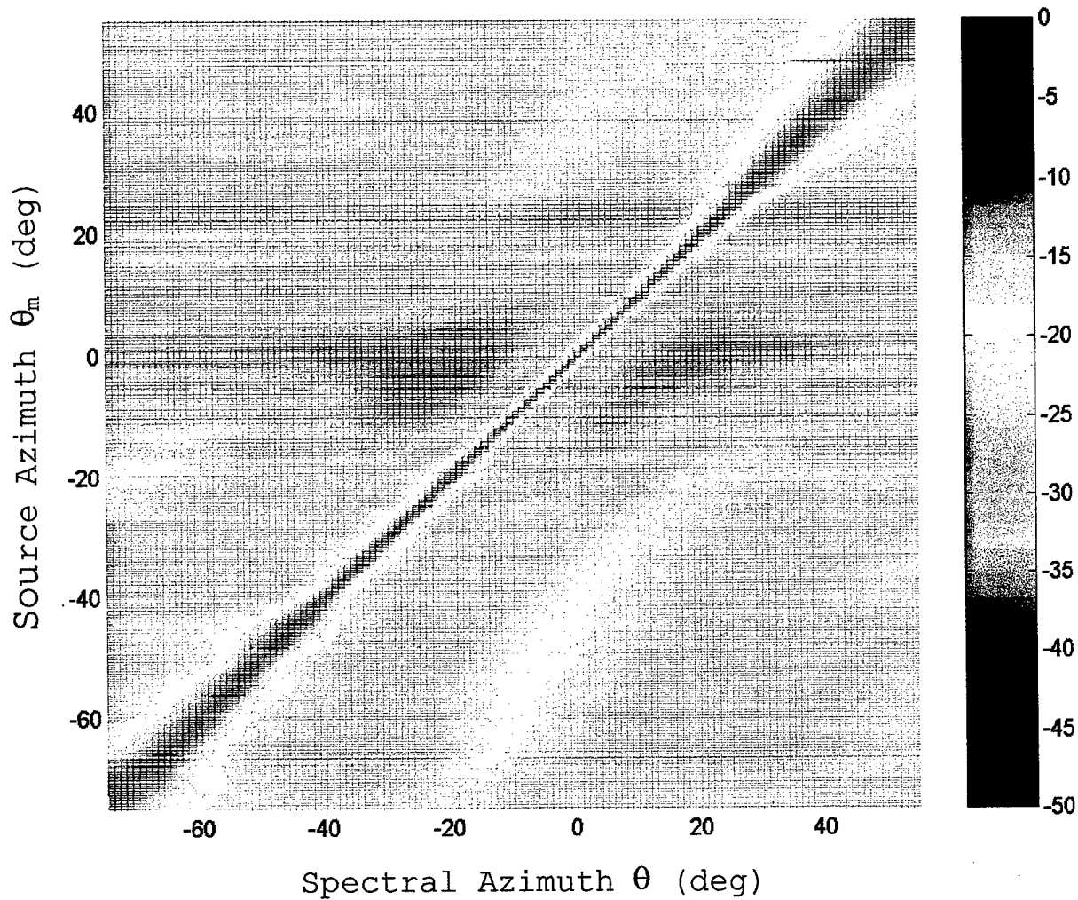
Figure 8c: Directional spectra of array snapshots in preprocessed calibration data file. Gain-and-phase matrix C_{GP} was used to calibrate the snapshots.
