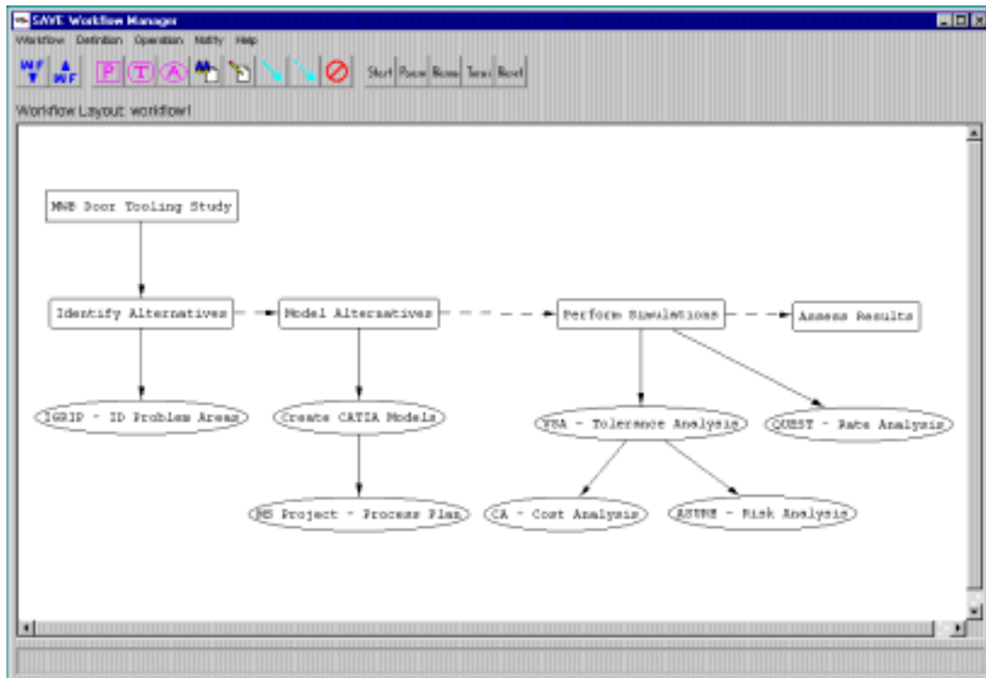
Figure 6-4. Study Workflow
