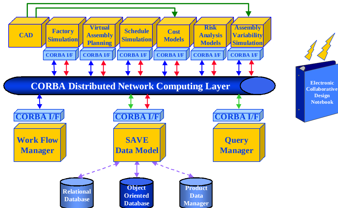
Figure 2-1. SAVE Architecture
