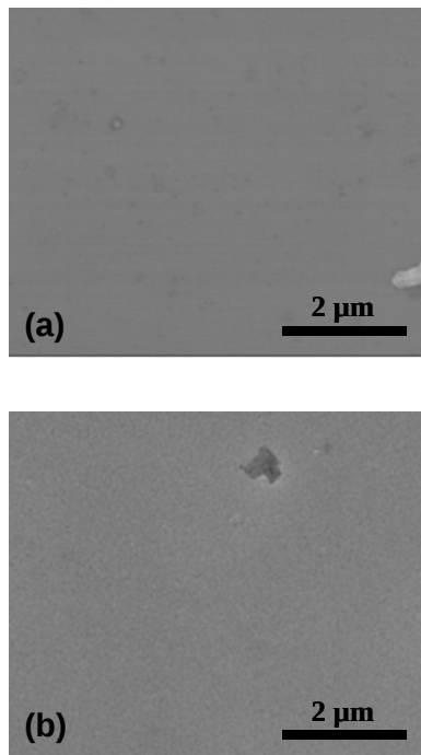
Figure 5. Plan-view FESEM micrographs showing the surface morphology of the (a) as-deposited and (b) 950^\circ\text{C} annealed \text{Ni}_2\text{Si} Ohmic contacts to n\text{-SiC} .
