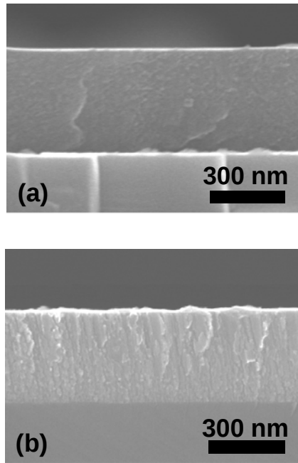
Figure 4. Cross-sectional FESEM micrographs of (a) as-deposited and (b) 950^\circ\text{C} annealed \text{Ni}_2\text{Si} Ohmic contacts to n\text{-SiC} .
