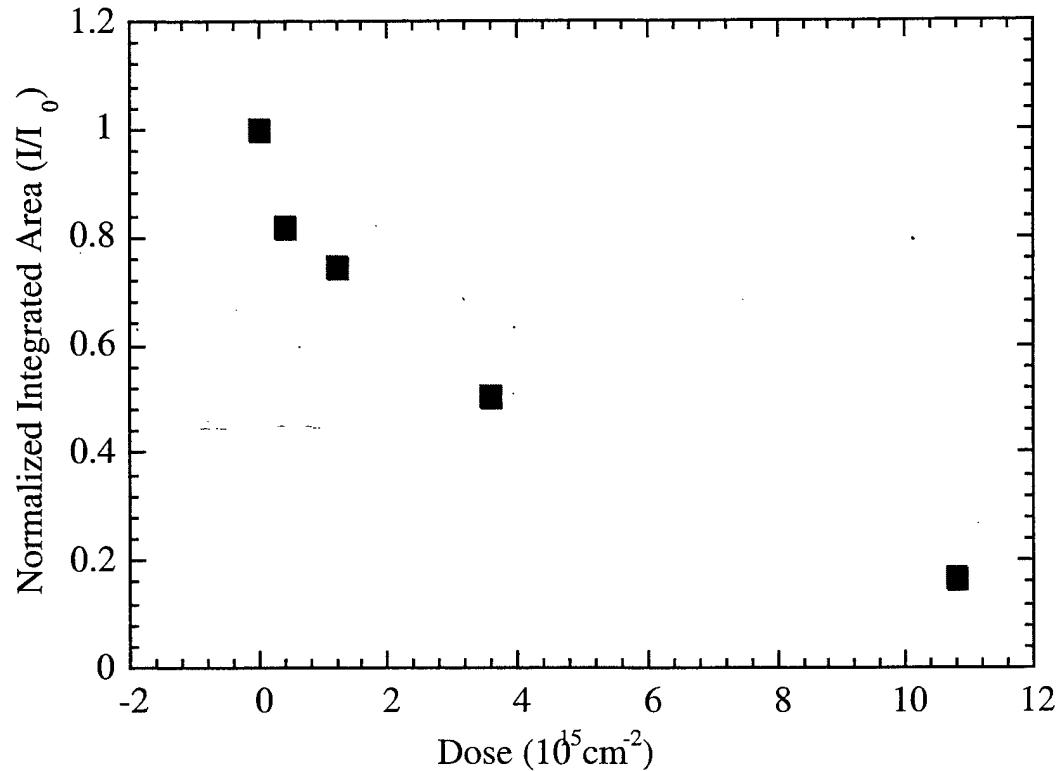
Fig. 2. Normalized integrated area ( I/I_0 ) of the PL spectra plotted as a function of the fast neutron irradiation dose. I_0 is the integrated area of spectrum (a) and I is the integrated area for spectra (b) - (e) in Fig. 1.
