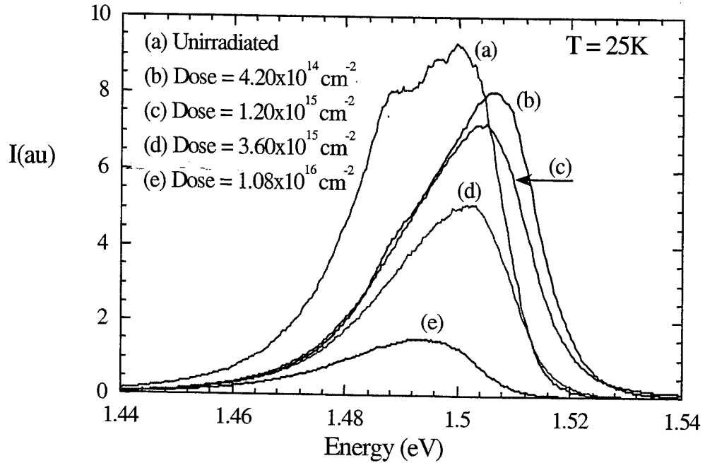
Fig. 1. Photoluminescence spectra obtained at T = 25K and plotted as a function of fast neutron irradiation dose. Spectrum (a) was obtained for the reference sample (unirradiated). The rest of the spectra were obtained for samples irradiated with different doses as indicated.
