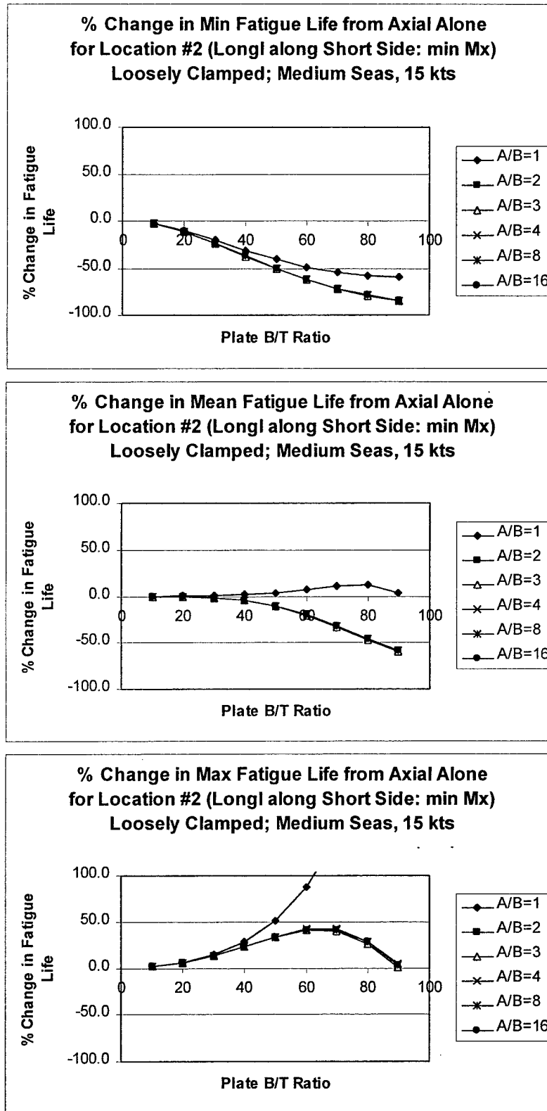
Figure 13. Fatigue Analysis with Loosely Clamped Edges in Medium Seas at 15 Knots: Location #2
