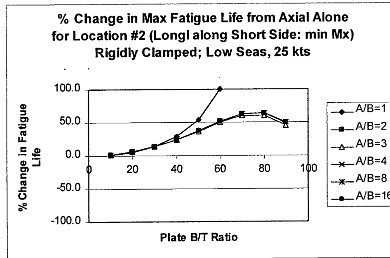
Figure 37. Fatigue Analysis with Rigidly Clamped Edges in Low Seas at 25 Knots: Location #2
