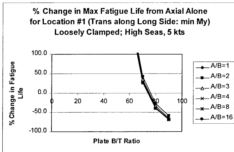
Figure 6. Fatigue Analysis with Loosely Clamped Edges in High Seas at 5 Knots: Location #1
