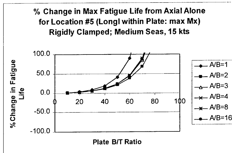
Figure 34. Fatigue Analysis with Rigidly Clamped Edges in Medium Seas at 15 Knots: Location #5
