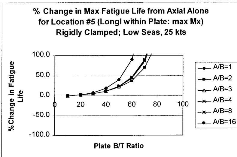
Figure 40. Fatigue Analysis with Rigidly Clamped Edges in Low Seas at 25 Knots: Location #5
