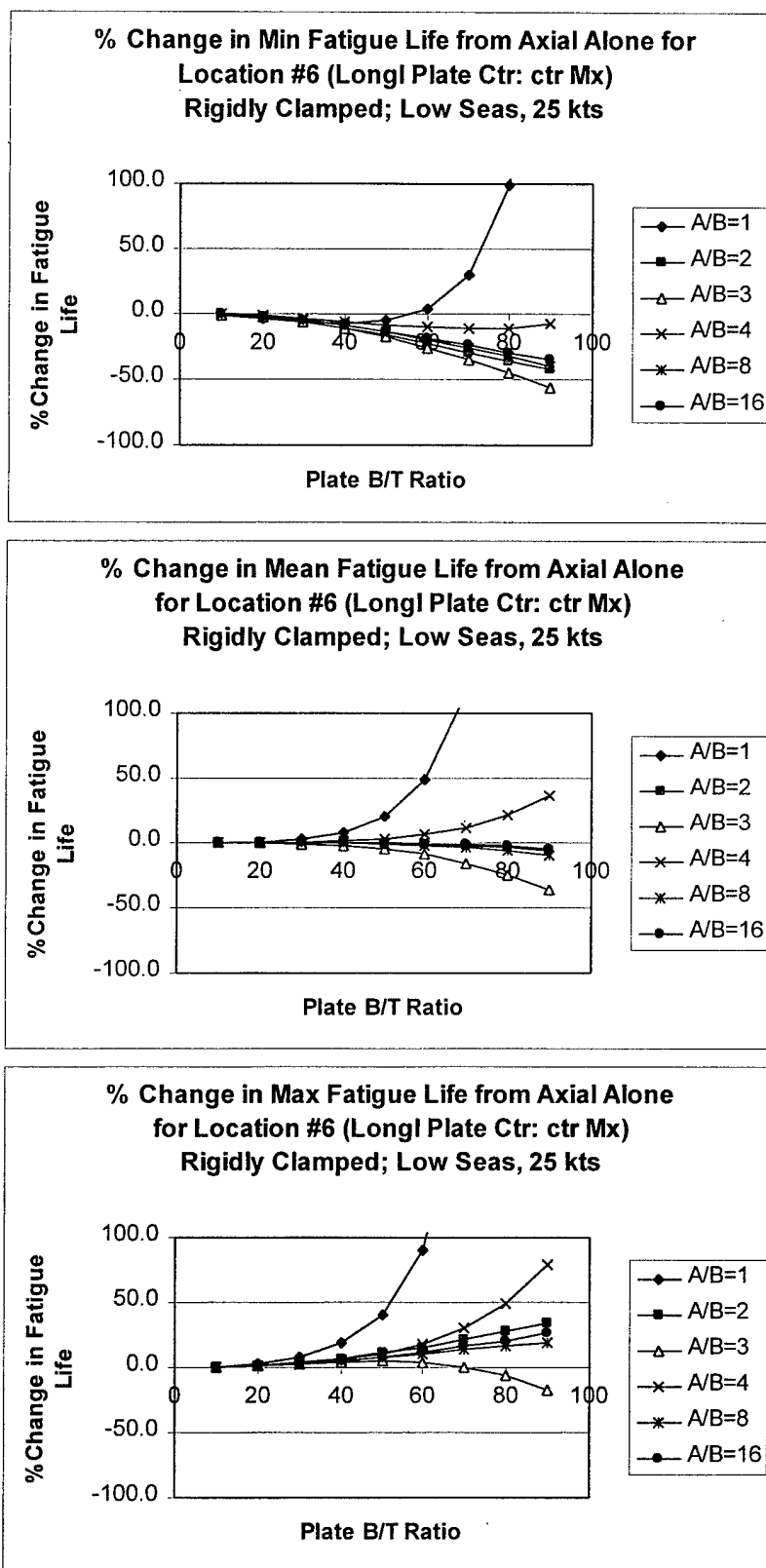
Figure 41. Fatigue Analysis with Rigidly Clamped Edges in Low Seas at 25 Knots: Location #6
