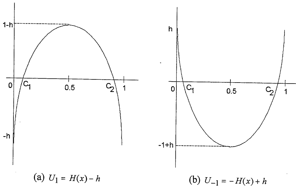
Fig. 12.1. Graphs of the potentials of choice. (a) Graph for agent I; the potential is not negative only at the interval [c_1, c_2] . (b) Graph for agent II; the potential is not negative for intervals [0, c_1] and [c_2, 1] .
