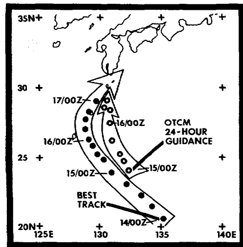
Figure 3-08-4. Plot of OTCM (One-way Interactive Tropical Cyclone Model) forecast tracks for period 140000Z to 161800Z July.
