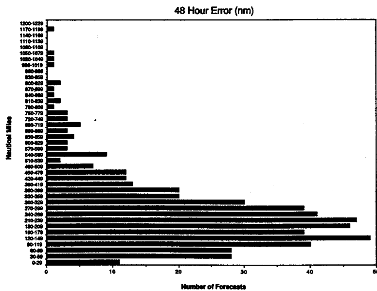
Figure 5-2. Frequency distribution of the 24-, 48-, and 72-hour forecast errors in 30 nm (56 km) increments for all significant tropical cyclones in the western North Pacific during 1986.
