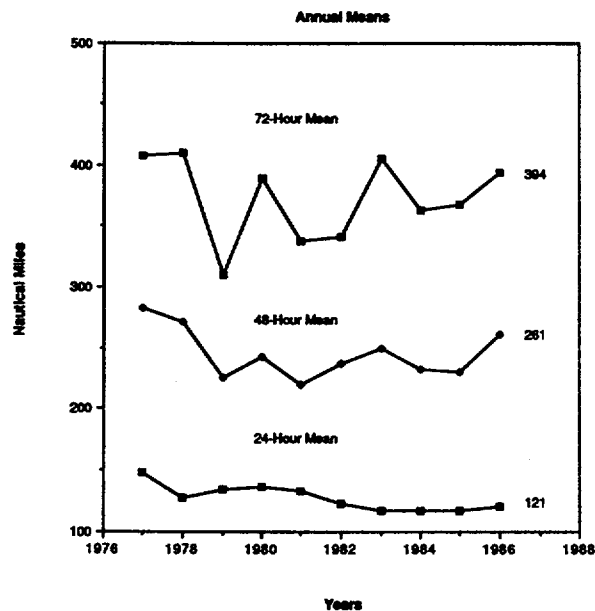
Figure 5-3. Annual mean forecast errors (in nm) for all tropical cyclones in the western North Pacific.
