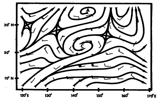
Figure 3-11-8. The 220000Z August 700 mb NVA analysis showing the trough (associated with the remnants of Typhoon Tip (10W)) to the northeast of Vera #2.
