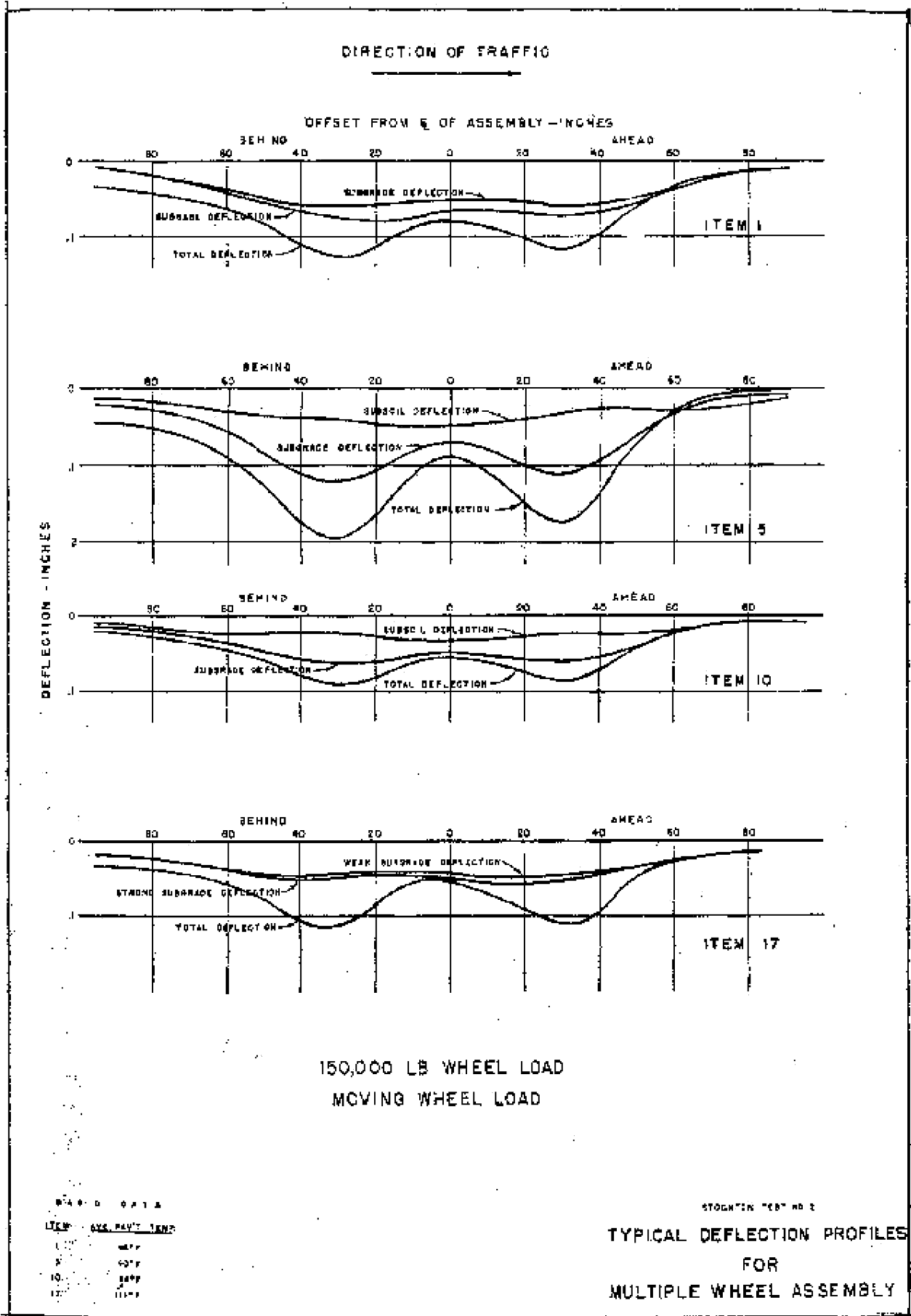
Figure 10. Typical longitudinal deflection profiles from tests at Stockton Airfield.
