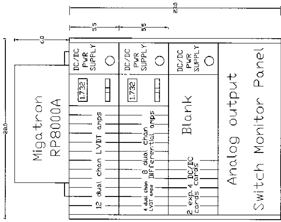
Figure 5. Spatial layout of signal-conditioning system. Dimensions are in inches.
