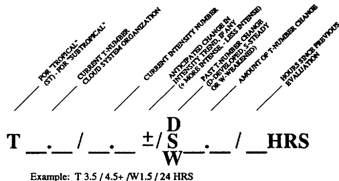
Figure 2-1. Dvorak code for communicating estimates of current and forecast intensity derived from satellite data. In the example, the current "T-number" is 3.5, but the current intensity is 4.5. The cloud system has weakened by 1.5 "T-numbers" since the previous evaluation conducted 24-hours earlier. The plus (+) symbol indicates an expected reversal of the weakening trend or very little further weakening of the tropical cyclone during the next 24-hour period.
