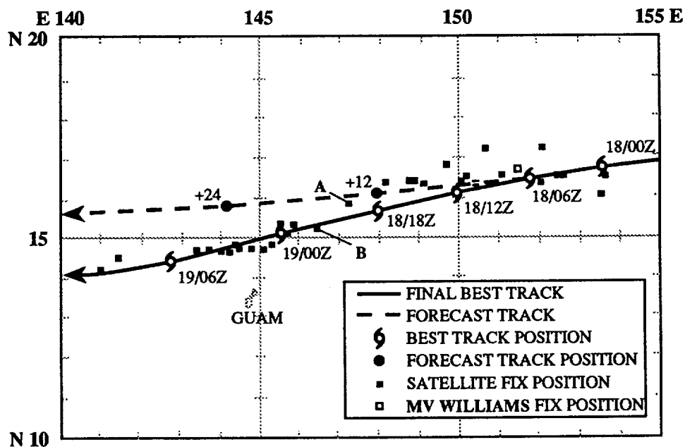
Figure 3-01-5. Comparison of expected track, raw fix data and final best track for Winona. The first daylight visual satellite fixes (A and B) were key elements in establishing Winona's continued movement to the west-southwest.
