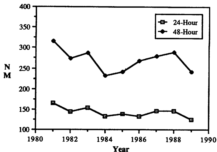
Figure 5-5. Annual mean forecast errors (nm) for all significant tropical cyclones in the South Pacific and South Indian Oceans.
