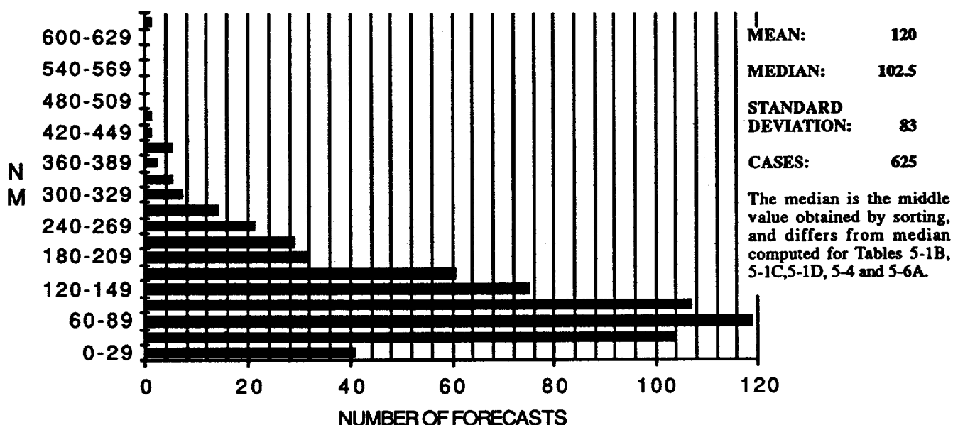
Figure 5-2B. Frequency distribution of 24-hour forecast errors (30 nm increments) for the western North Pacific in 1989.
