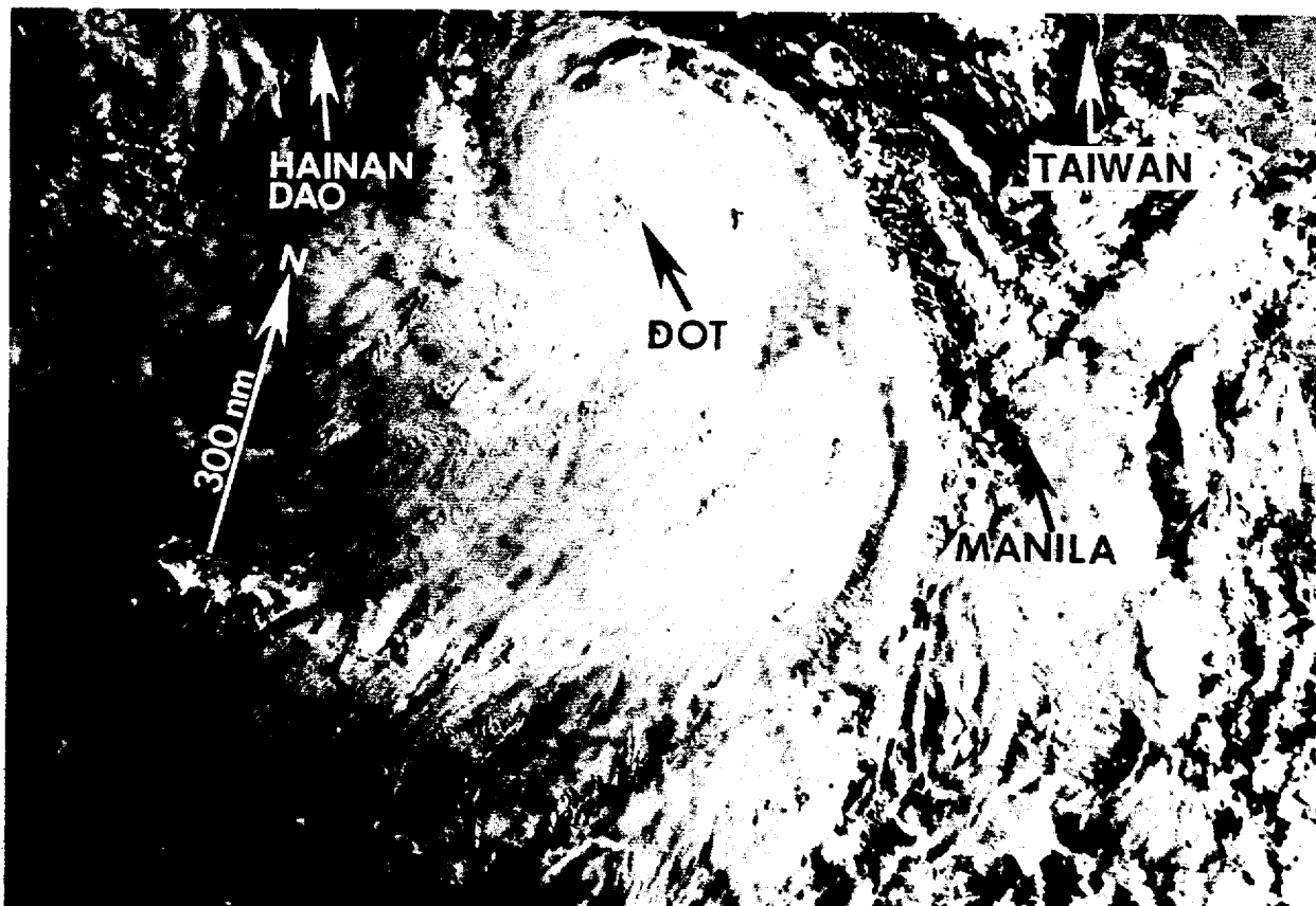
Figure 3-05-4. Nearing peak intensity, Typhoon Dot tracks towards Hainan Island (082225Z June DMSP visual imagery).
