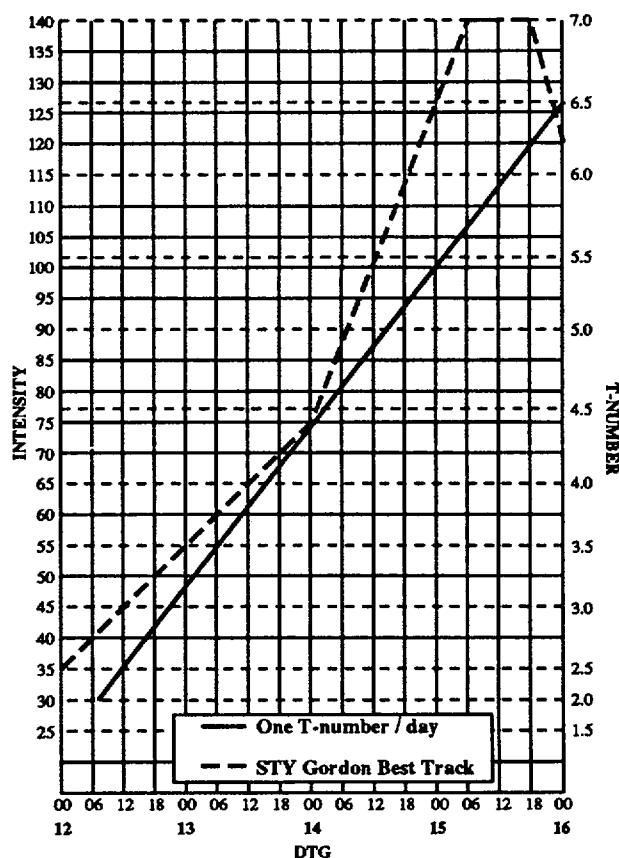
Figure 3-08-2. Gordon's rapid intensification after 140000Z compared with an increase of one "T" number per day.
