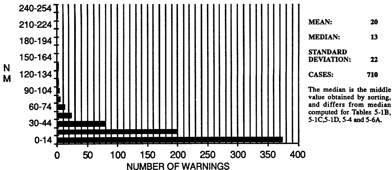
Figure 5-2A. Frequency distribution of initial position errors (15 nm increments) for the western North Pacific in 1989.
