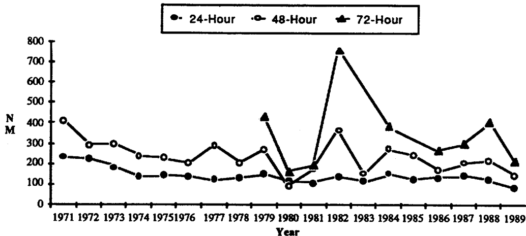
Figure 5-4. Annual mean forecast errors (nm) for all significant tropical cyclones in the North Indian Ocean.
