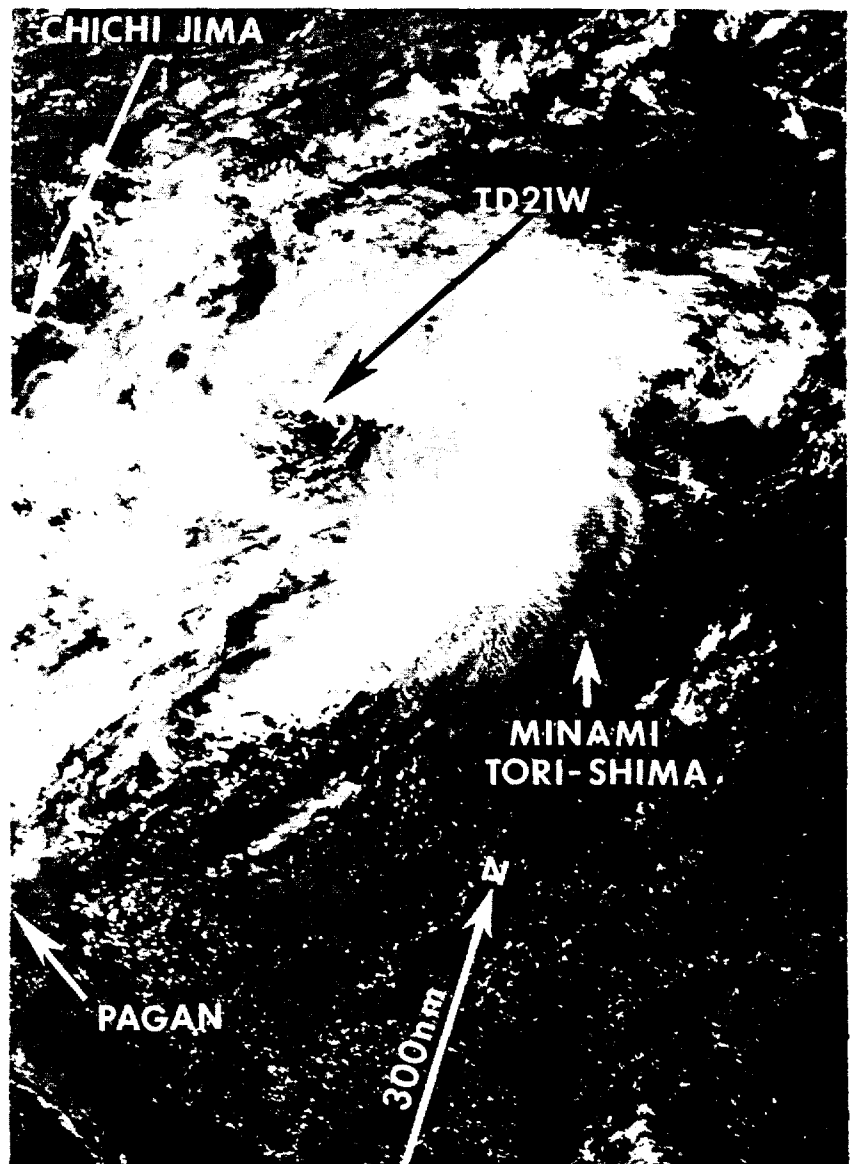
Figure 3-21-1. Convective organization continues to increase after the Alert was issued (242242Z August DMSP visual imagery).
