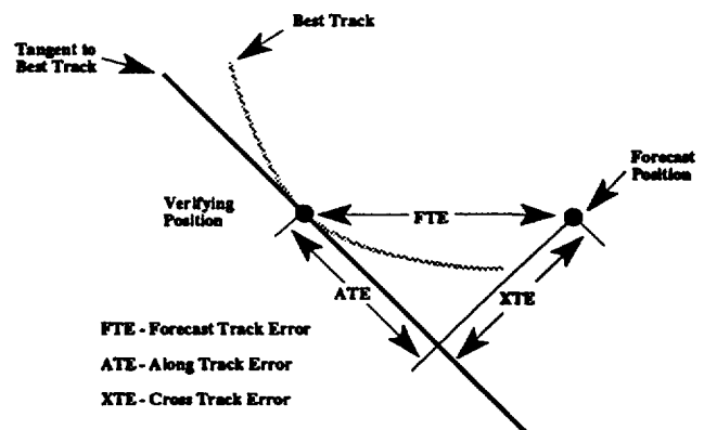
Figure 5-1. Definition of cross-track error (XTE), along-track error (ATE) and forecast track error (FTE). In this example, the XTE is positive (to the right of the best track) and the ATE is negative (behind or slower than the best track).
