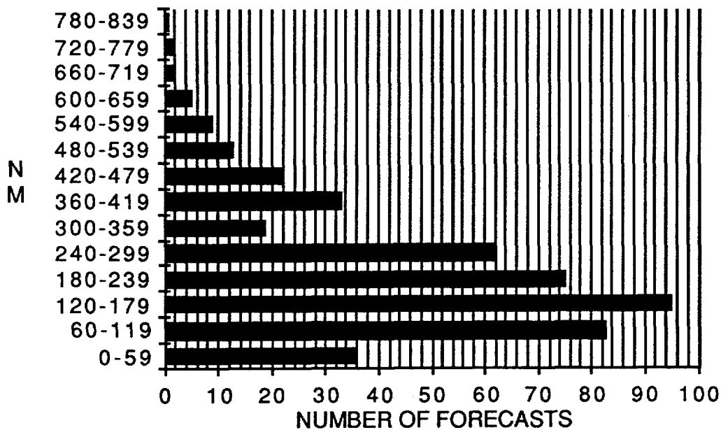
Figure 5-2C. Frequency distribution of 48-hour forecast errors (60 nm increments) for the western North Pacific in 1989.
