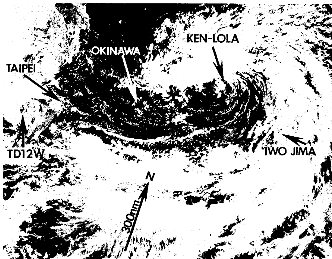
Figure 3-13-2. Imagery supporting the final warning on Tropical Storm Ken and formation of Lola. Note remnants of TD12W in the Taiwan Strait (310025Z July DMSP visual imagery).
