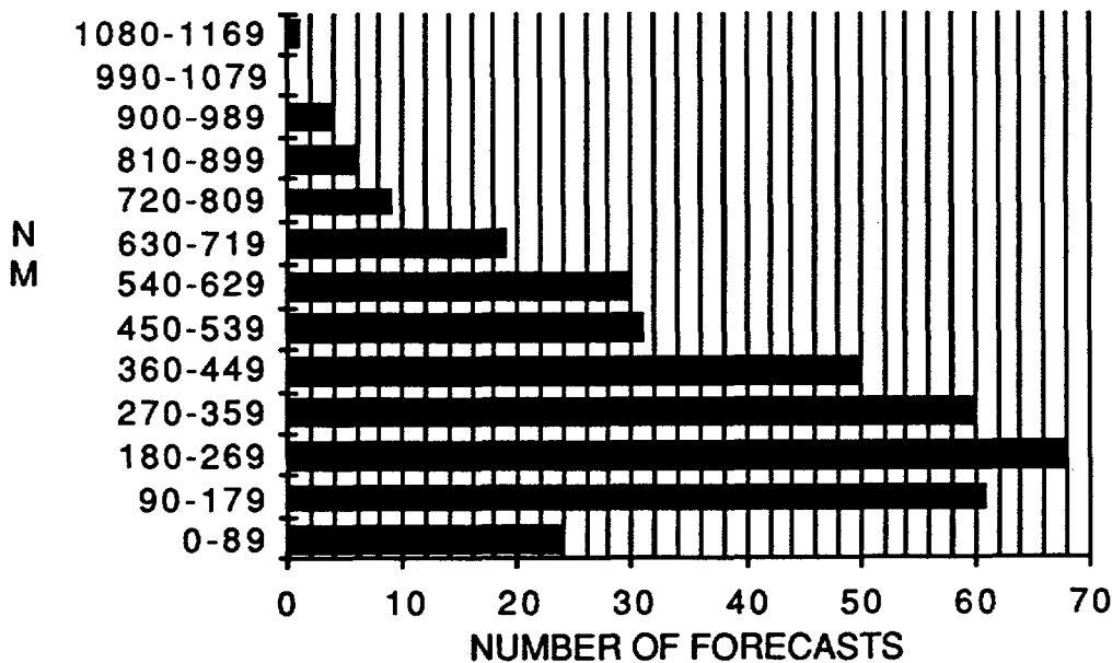
Figure 5-2D. Frequency distribution of 72-hour forecast errors (90 nm increments) for the western North Pacific in 1989.
