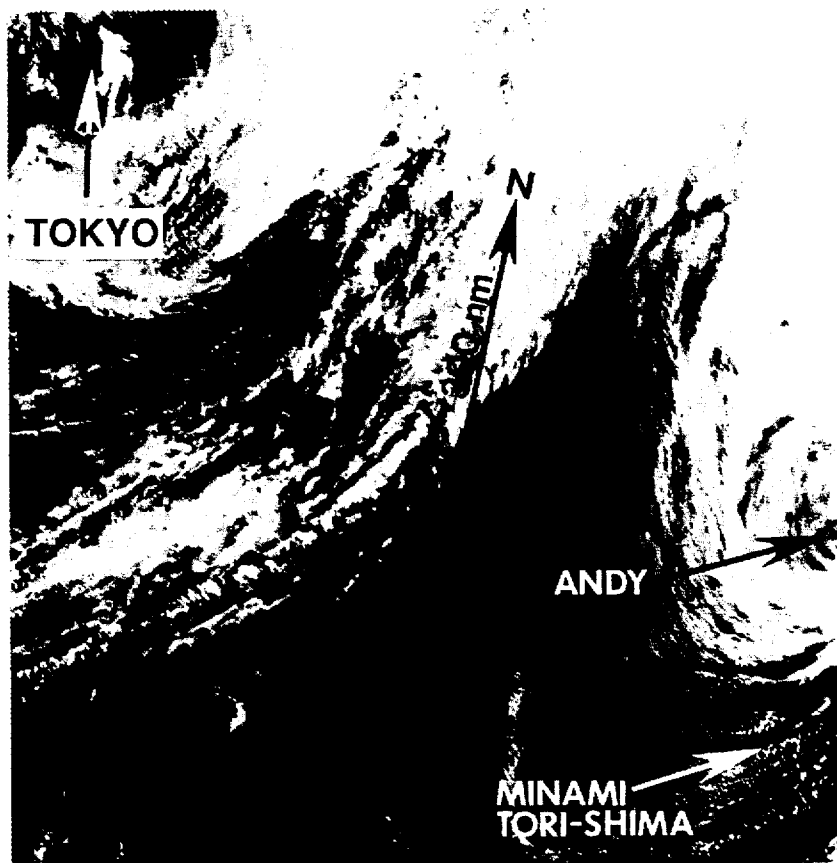
Figure 3-02-7. Remnants of Andy's low-level circulation (242322Z April DMSP visual imagery).
