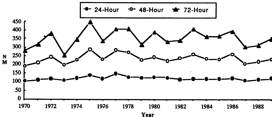
Figure 5-3. Annual mean forecast errors (nm) for all significant tropical cyclones in the western North Pacific.
