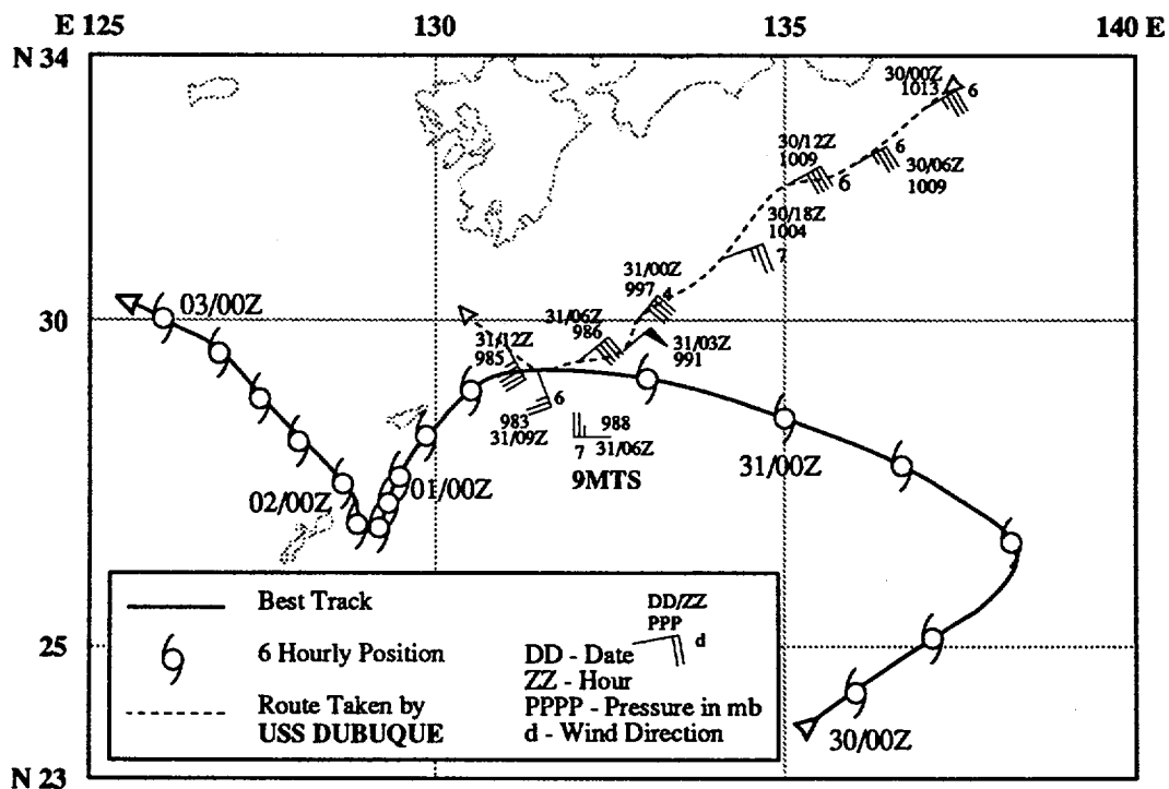
Figure 3-13-3. Wind and pressure reports from the USS Dubuque (LPD8) from 300000Z through 311200Z July with a report from ship 9MTS at 310600Z help define the circulation center. Tropical storm symbols represent six-hourly best track positions for Tropical Storm Ken-Lola.
