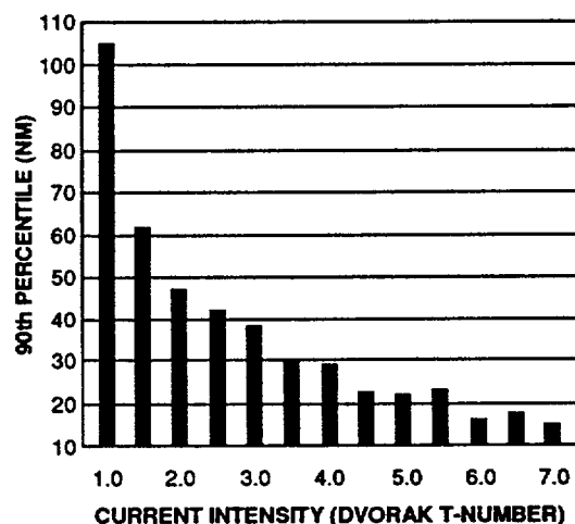
Figure 2-3. A stratification of western North Pacific satellite fix errors (90th percentile) and current intensities (Dvorak T-numbers). For example: for a tropical cyclone with a current intensity of T1.0, 90% of the fixes fell within 105 nm (195 km) of the final best track position.
