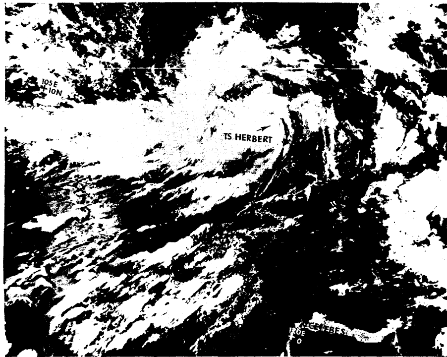
Figure 3-13-1. Herbert as a tropical depression in the South China Sea (060730Z NOAA 7 visual imagery).
