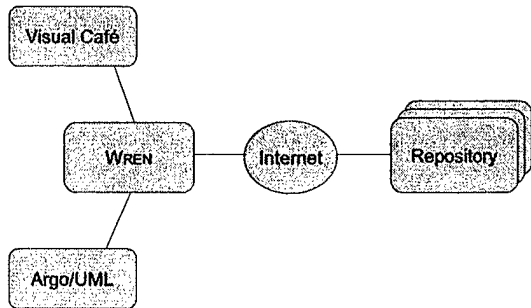
Figure 2: Architecture of WREN.
