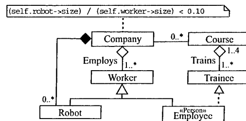
Figure 1. An example design expressed in UML
