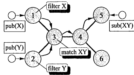
Figure 9: Applying filters and patterns upstream
