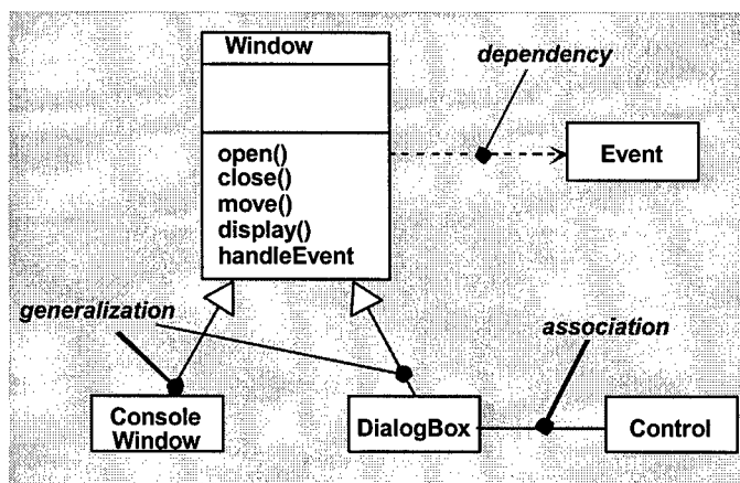
Figure 4. UML relationships.
