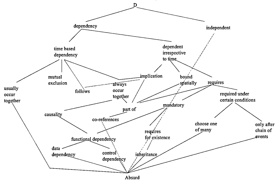
Fig. 4. Dependency type hierarchy
