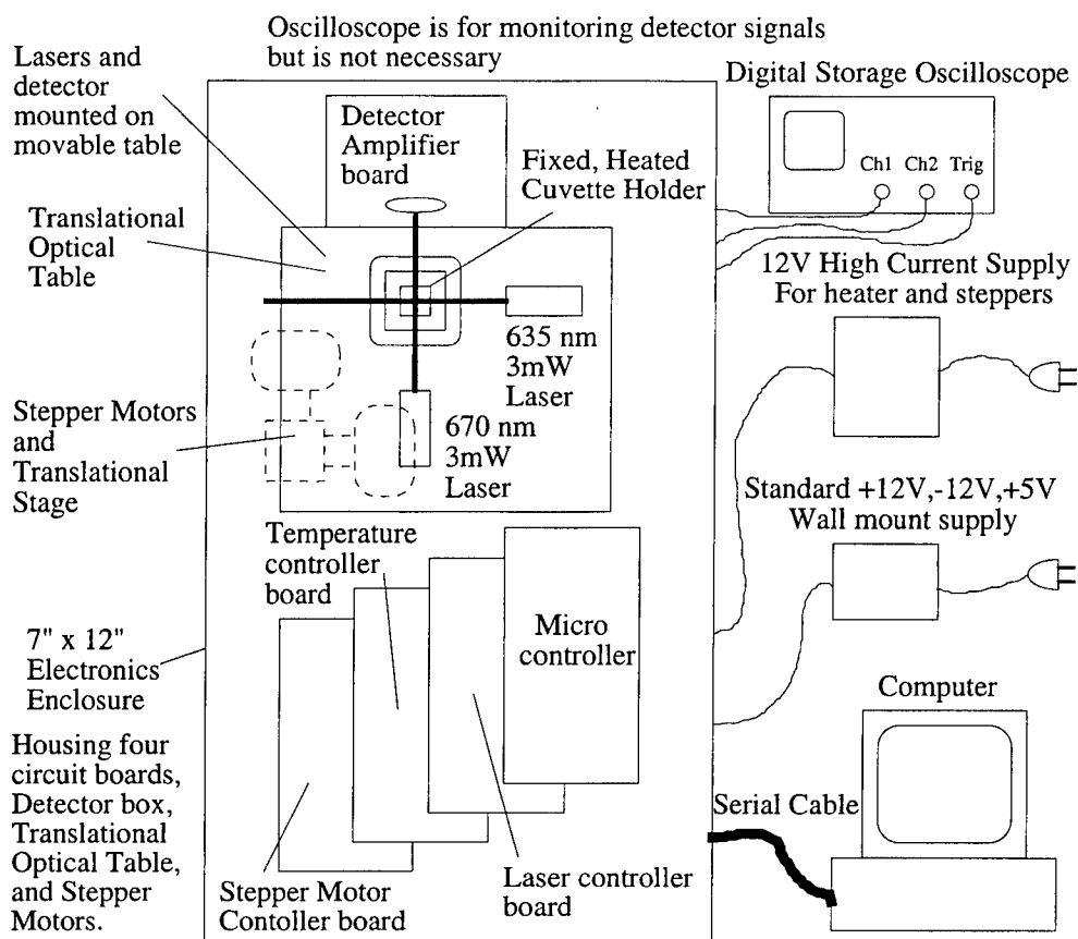
Fig 3.2.10: Block diagram of the miniature prototype.
