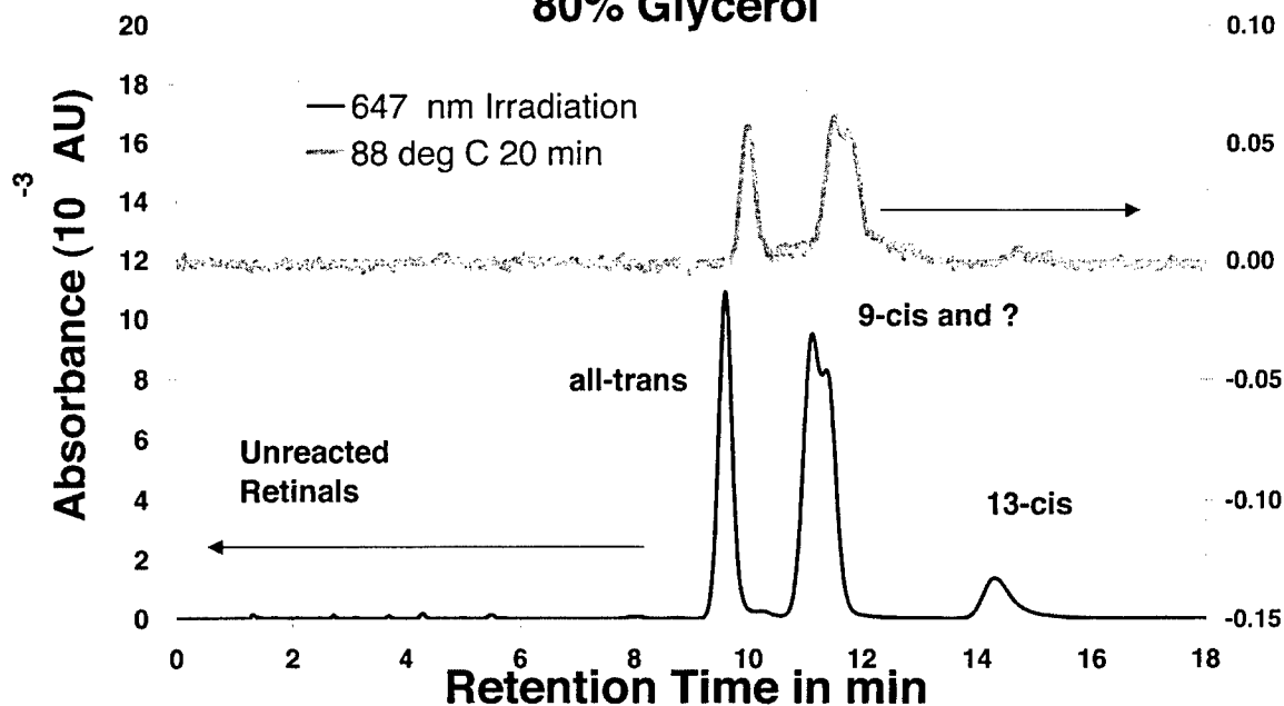
Figure 3.1.1.9. HPLC chromatograms of two chromophore analysis experiments on the renaturable, photochemically formed Q state (bottom, left vertical axis), and the first permanent thermally denatured state of bR (top, right vertical axis).
