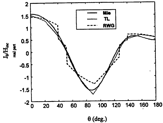
Figure 8. Current distribution (real part only) over a PEC sphere of radius 0.4\lambda , obtained using a 160 triangular patch discretization for RWG basis and first order basis (TL), compared against the exact Mie's solution. The wave is incident from \theta = 0^\circ .
