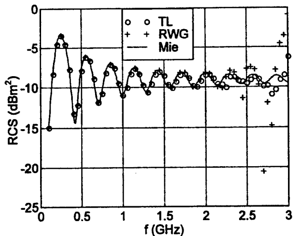
Figure 11. RCS prediction as a function of frequency for a sphere of radius 0.2\text{ m} , using a 424-facet model (discretization \cong 0.05\text{ m} ) for RWG basis functions and first order basis (TL) functions, compared against the exact Mie's solution.
