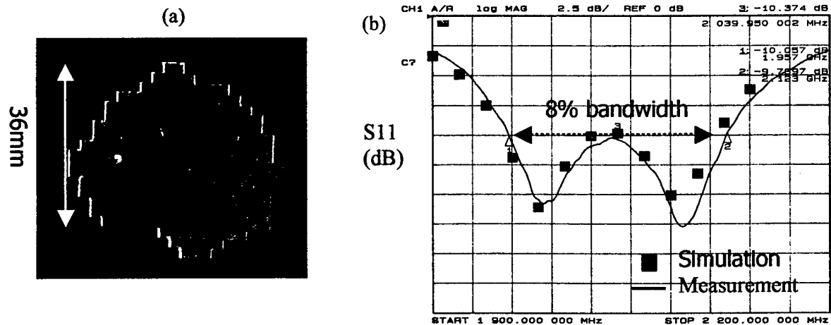
Fig. 1. A broadband microstrip antenna designed using the genetic algorithm and built on FR-4 material. The right figure shows the return loss (dB) of the antenna from simulation (□) and measurement (—). The antenna has an operating frequency of 2 GHz and an 8% bandwidth, which is 4 times broader than a conventional square microstrip.
