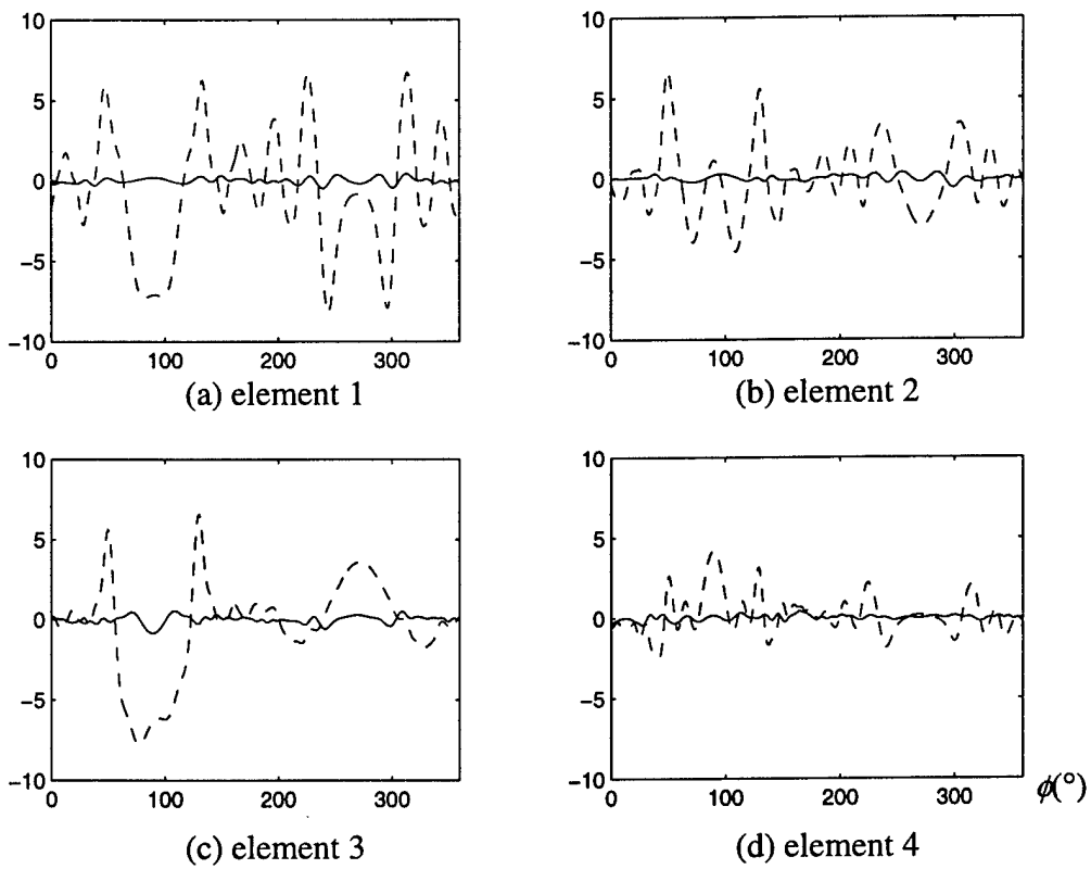
Fig. 5. Phase error of the reconstructed active element patterns
