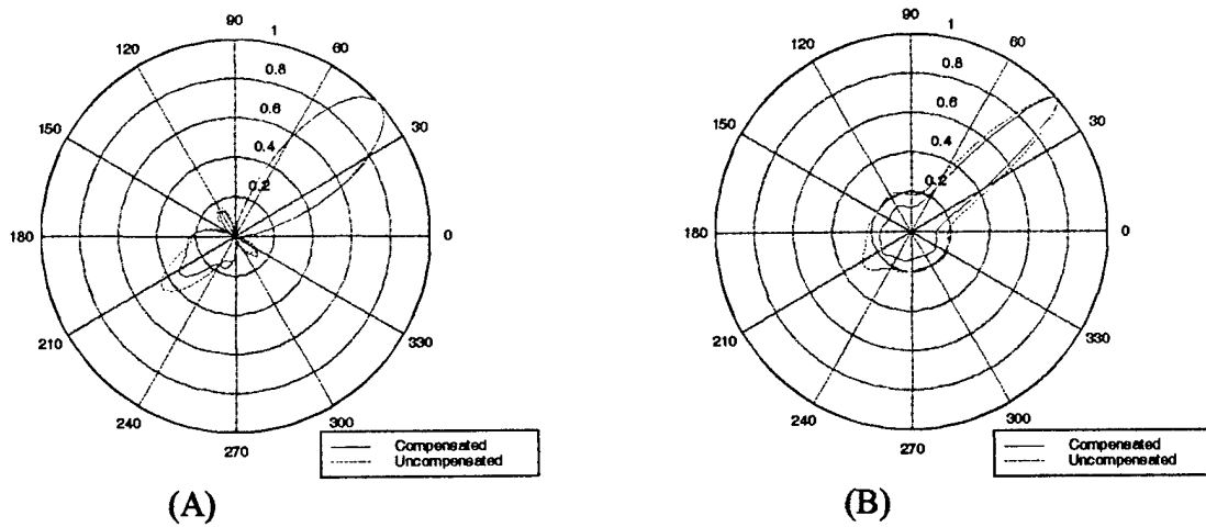
Figure 4 – Experimental Data Mobile Position 1 Spatial Spectra - (A) Bartlett DOA Algorithm (B) MUSIC DOA Algorithm
