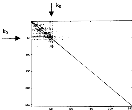
Figure 4. The moment matrix represented by PWP basis, [\tilde{Z}] , for the inlet with N=256 (in logarithmic scale).
