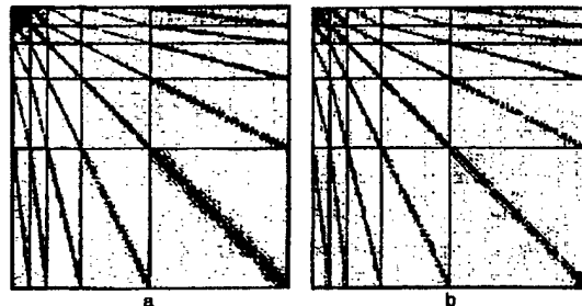
Fig. 1 Wavelet transformed moment matrix [\tilde{\mathbf{Z}}] and its inverse [\tilde{\mathbf{Z}}]^{-1} for rectangular cavity
