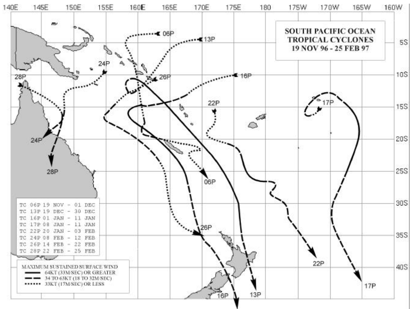
Figure 4-5 Tropical Cyclone best tracks for the South Pacific Ocean
