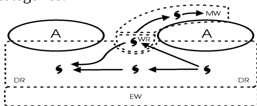
Figure 1-2 Standard Pattern
