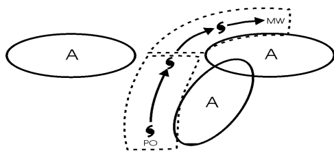
Figure 1-3 Poleward Pattern
