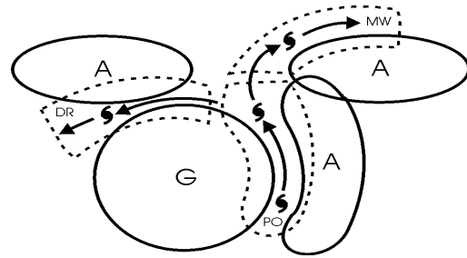
Figure 1-4 Gyre Pattern
