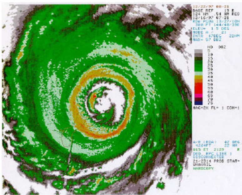
Figure 3-05C-2 NEXRAD imagery of Paka early on 16 December, 1997.
