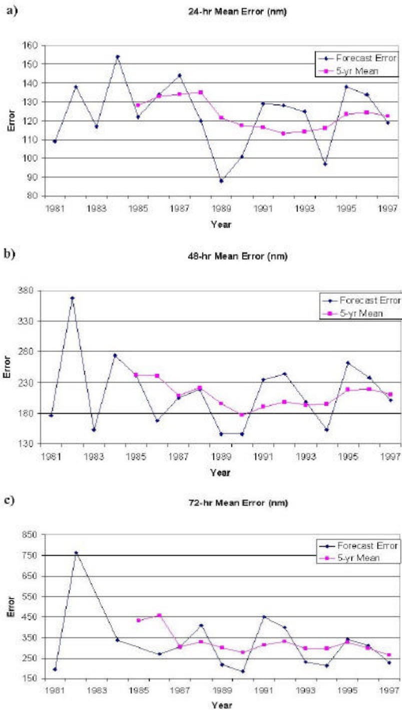
Figure 5-5 Mean track forecast error (nm) and 5-year running mean for a) 24 hours b) 48 hours and c) 72 hours for the western North Indian Ocean tropical cyclones for the period 1981 to 1997.
